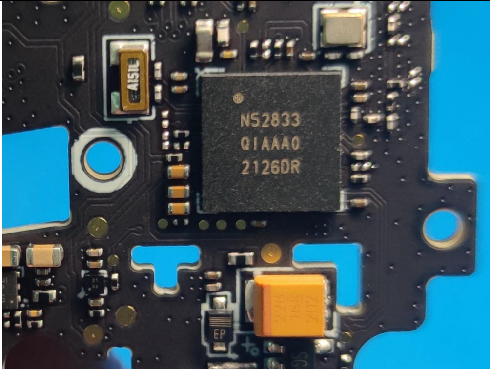
EUT Photo(8) -Left-Antenna
