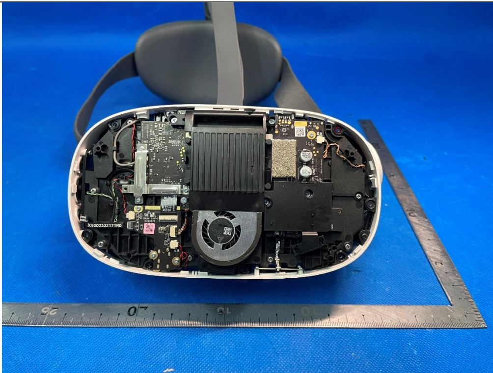
(4) EUT Photo - EUT1
