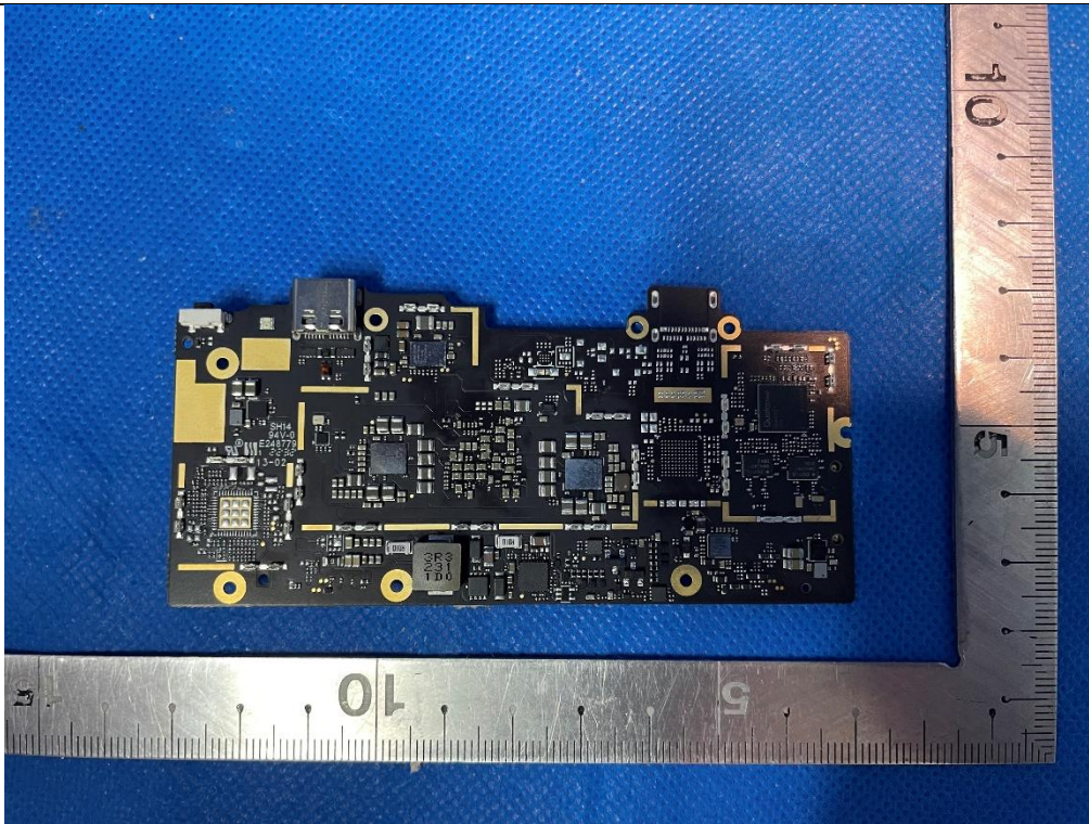
(8) EUT Photo - EUT1
