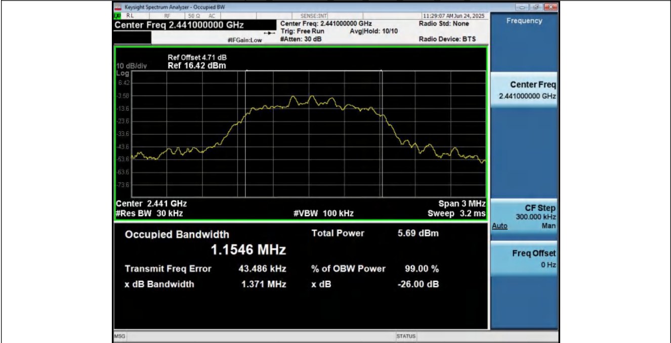
99% Occupied Bandwidth_NVNT_ANT1_3-DH1_2441_00
