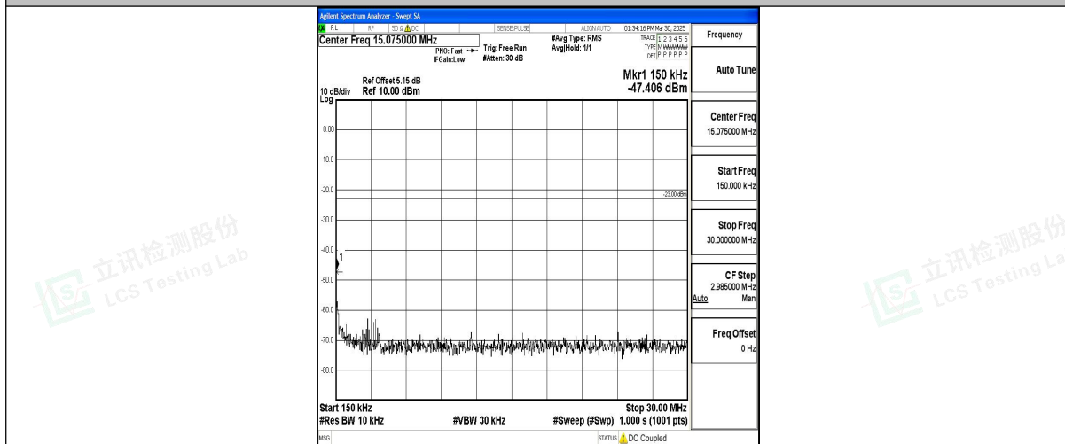
Band12_10MHz_QPSK_23095_1RB#0_0.15~30_0.15~30
