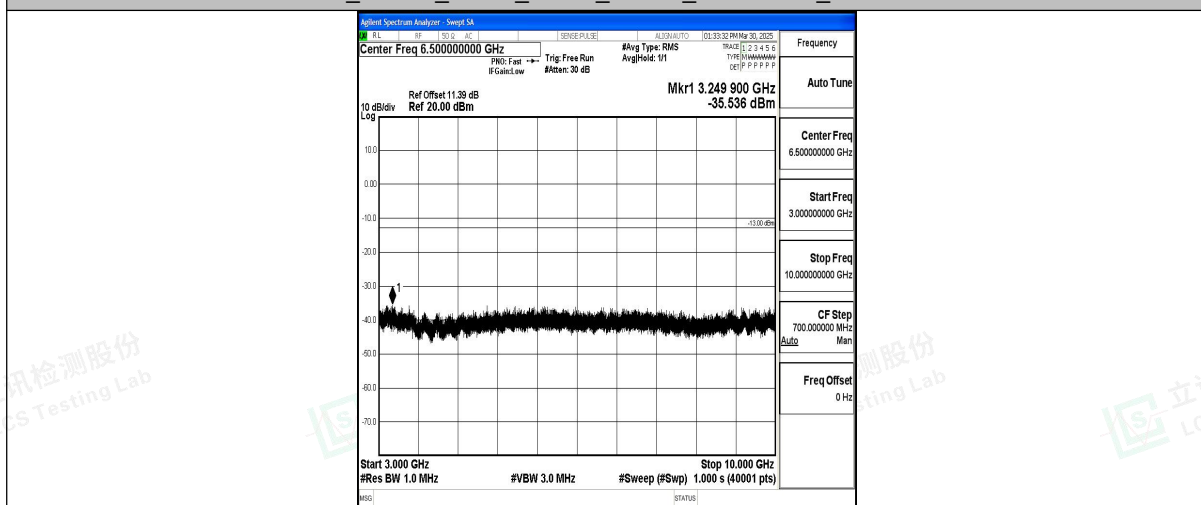
Band12_10MHz_QPSK_23060_1RB#0_3000~10000_3000~10000
