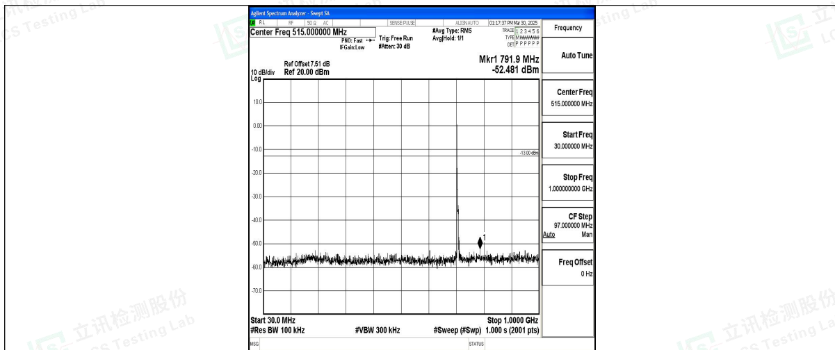
Band12_5MHz_16QAM_23155_1RB#0_30~1000_30~1000
