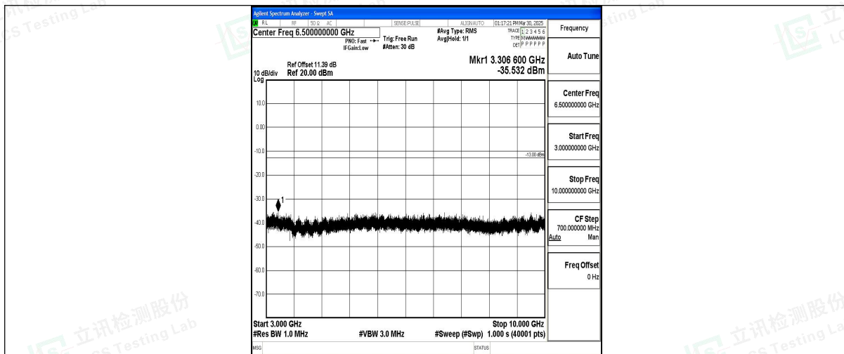
Band12_5MHz_QPSK_23155_1RB#0_3000~10000_3000~10000
