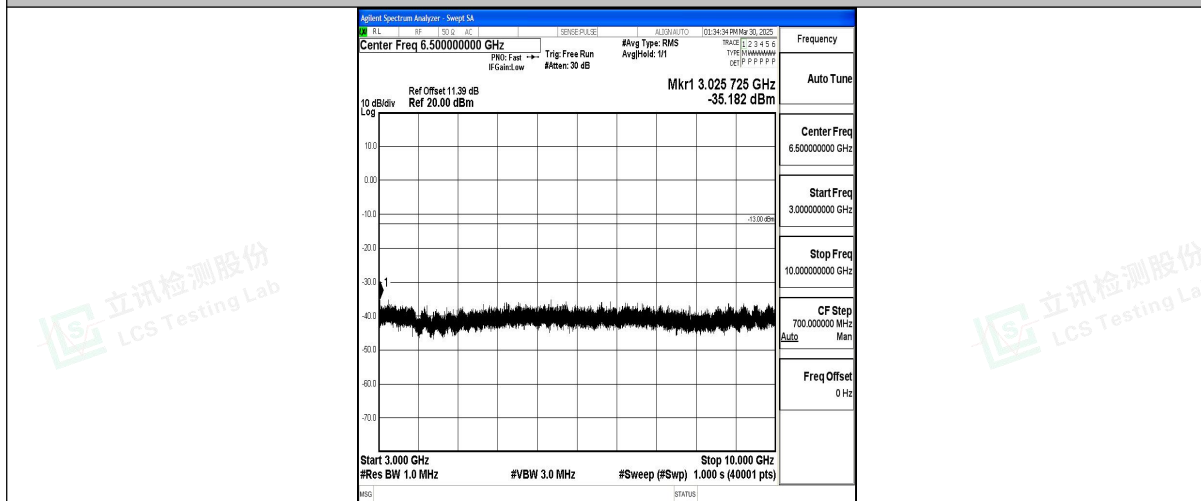
Band12_10MHz_QPSK_23095_1RB#0_3000~10000_3000~10000
