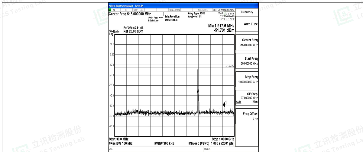
Band12_10MHz_QPSK_23095_1RB#0_30~1000_30~1000
