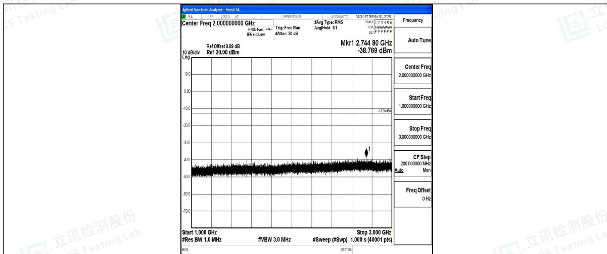
Band12_10MHz_16QAM_23095_1RB#0_1000~3000_1000~3000
