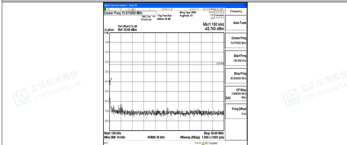
Band12_5MHz_16QAM_23155_1RB#0_0.15~30_0.15~30
