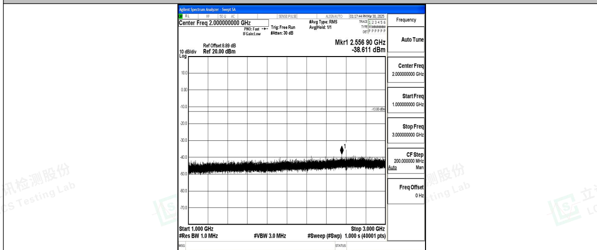
Band12_5MHz_16QAM_23155_1RB#0_1000~3000_1000~3000
