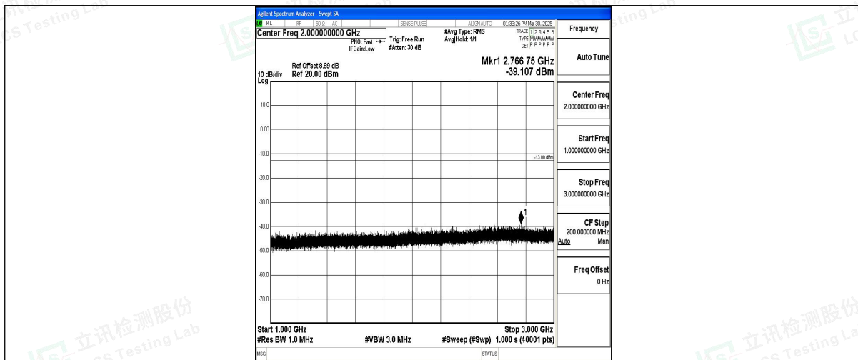
Band12_10MHz_QPSK_23060_1RB#0_1000~3000_1000~3000
