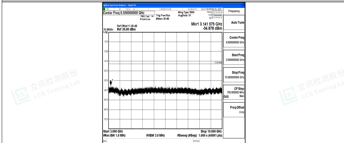
Band12_5MHz_16QAM_23155_1RB#0_3000~10000_3000~10000
