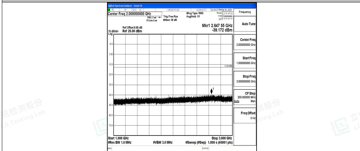
Band12_10MHz_QPSK_23095_1RB#0_1000~3000_1000~3000
