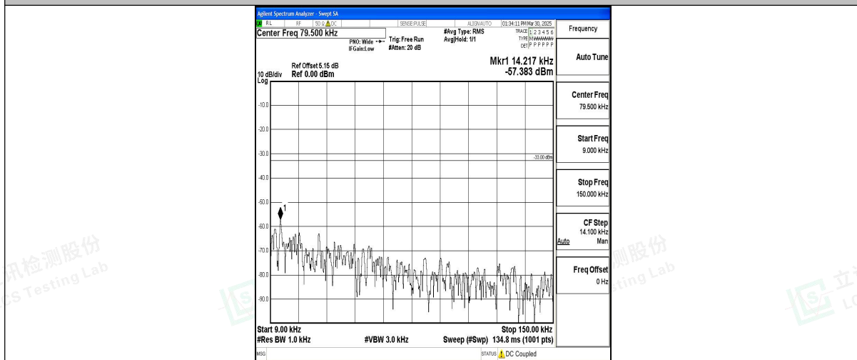
Band12_10MHz_QPSK_23095_1RB#0_0.009~0.15_0.009~0.15
