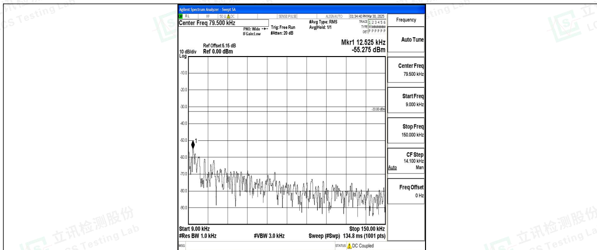
Band12_10MHz_16QAM_23095_1RB#0_0.009~0.15_0.009~0.15
