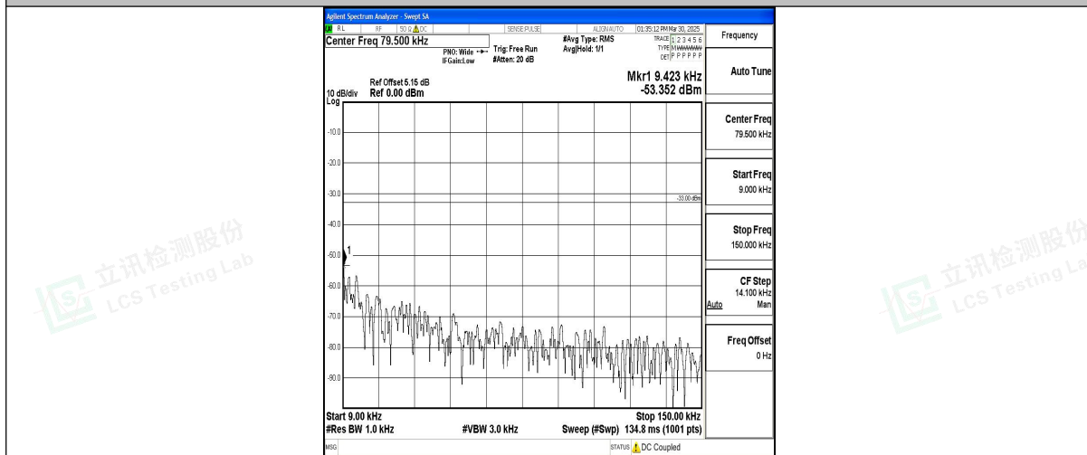
Band12_10MHz_QPSK_23130_1RB#0_0.009~0.15_0.009~0.15
