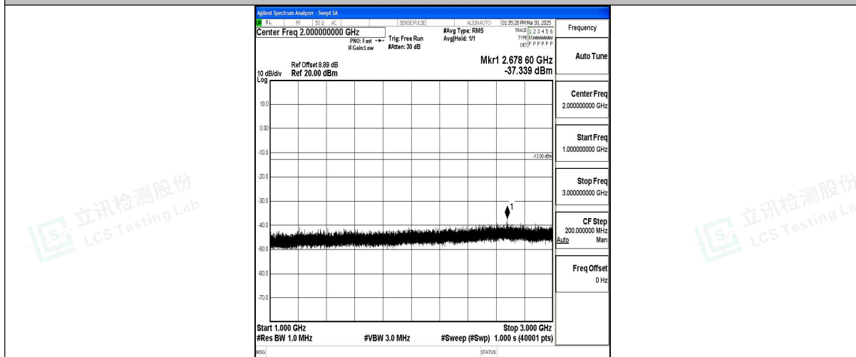
Band12_10MHz_QPSK_23130_1RB#0_1000~3000_1000~3000
