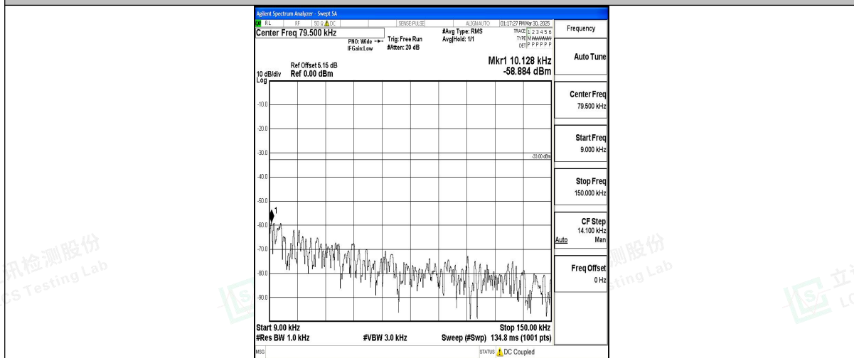
Band12_5MHz_16QAM_23155_1RB#0_0.009~0.15_0.009~0.15
