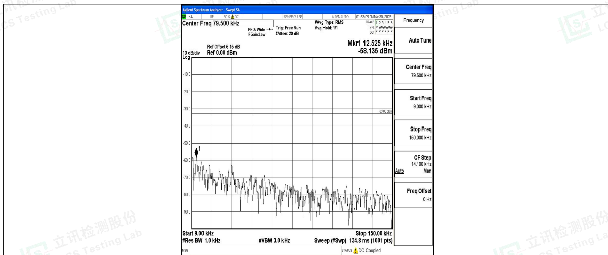
Band12_10MHz_QPSK_23060_1RB#0_0.009~0.15_0.009~0.15
