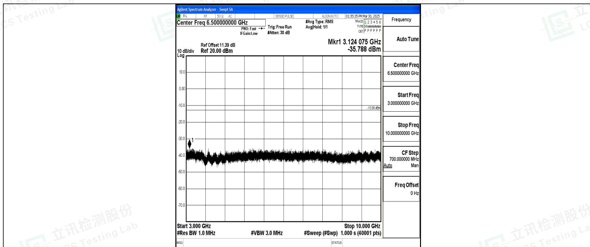
Band12_10MHz_QPSK_23130_1RB#0_3000~10000_3000~10000
