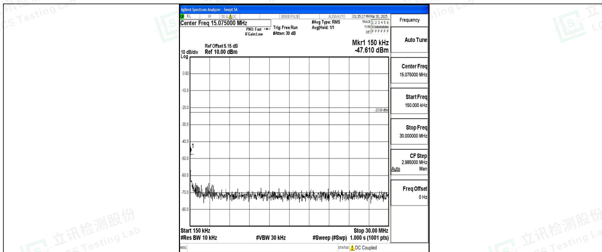
Band12_10MHz_QPSK_23130_1RB#0_0.15~30_0.15~30
