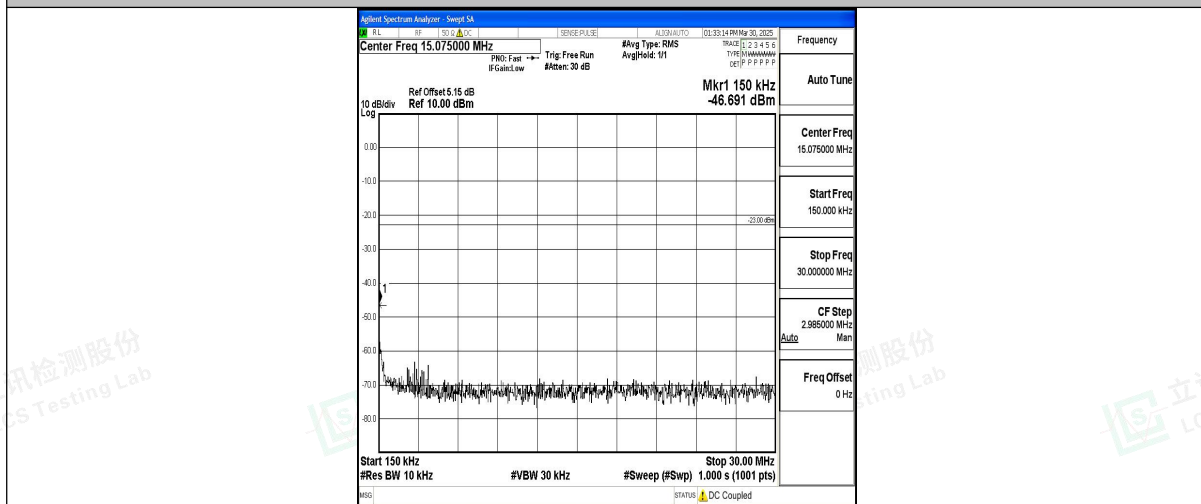
Band12_10MHz_QPSK_23060_1RB#0_0.15~30_0.15~30
