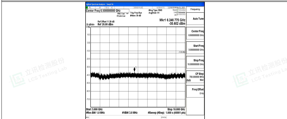
Band12_3MHz_16QAM_23165_1RB#0_3000~10000_3000~10000
