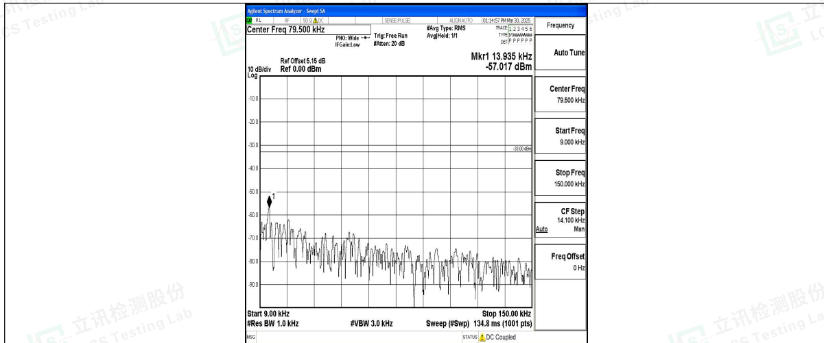
Band12_5MHz_QPSK_23035_1RB#0_0.009~0.15_0.009~0.15
