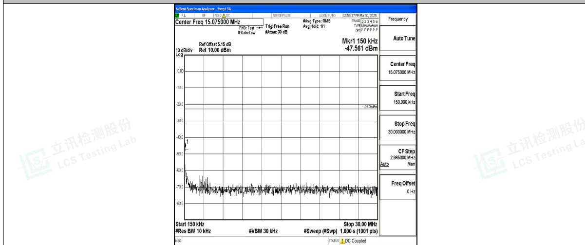
Band12_3MHz_16QAM_23165_1RB#0_0.15~30_0.15~30
