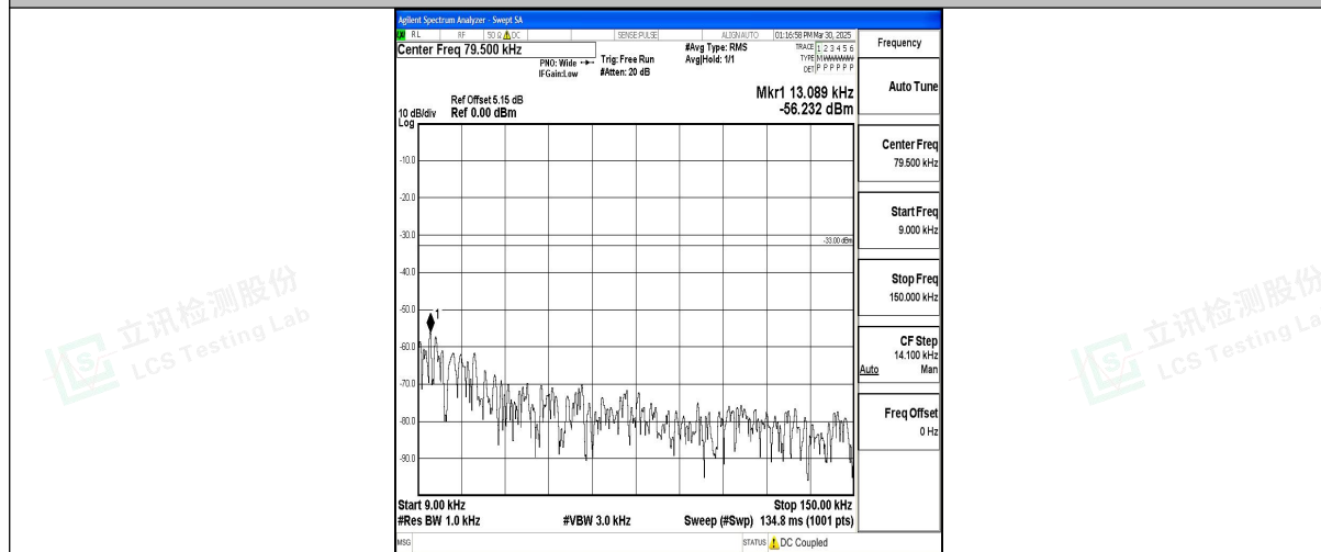
Band12_5MHz_QPSK_23155_1RB#0_0.009~0.15_0.009~0.15
