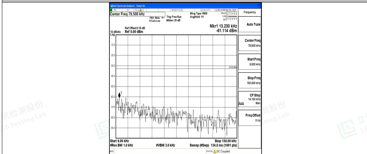
Band12_3MHz_16QAM_23165_1RB#0_0.009~0.15_0.009~0.15
