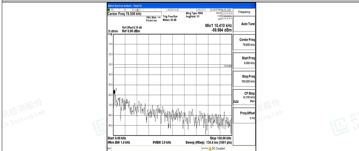
Band12_5MHz_QPSK_23095_1RB#0_0.009~0.15_0.009~0.15
