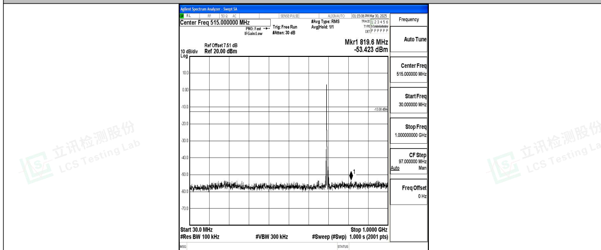
Band12_5MHz_QPSK_23035_1RB#0_30~1000_30~1000
