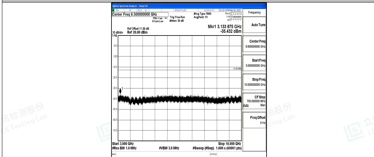
Band12_5MHz_QPSK_23035_1RB#0_3000~10000_3000~10000
