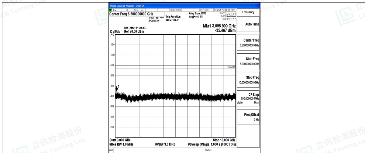
Band12_3MHz_QPSK_23165_1RB#0_3000~10000_3000~10000
