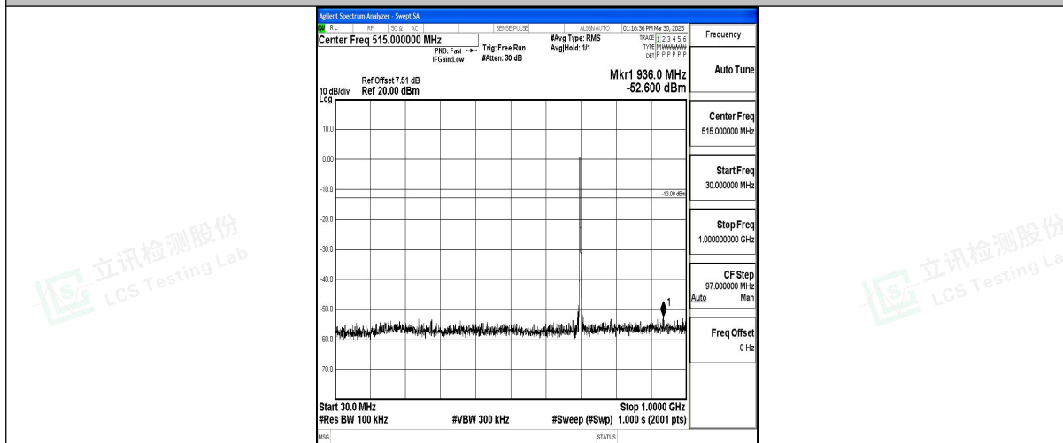
Band12_5MHz_16QAM_23095_1RB#0_30~1000_30~1000
