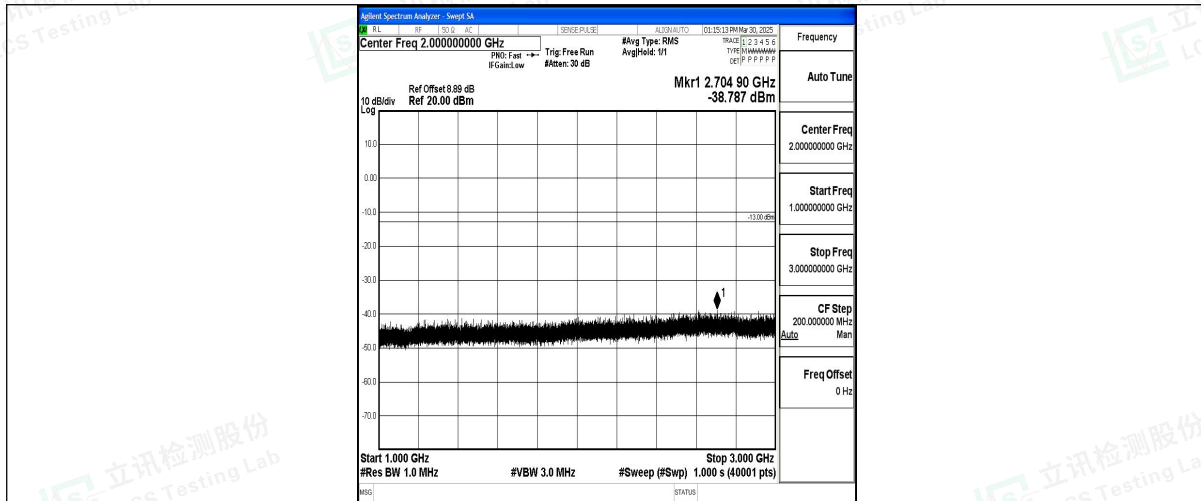
Band12_5MHz_QPSK_23035_1RB#0_1000~3000_1000~3000
