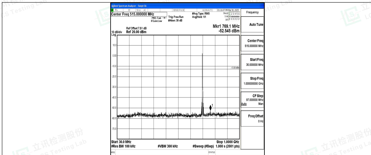
Band12_5MHz_QPSK_23095_1RB#0_30~1000_30~1000
