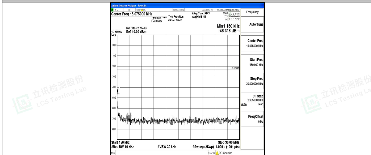
Band12_5MHz_QPSK_23095_1RB#0_0.15~30_0.15~30
