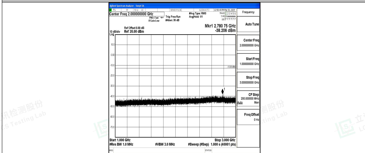
Band12_3MHz_16QAM_23165_1RB#0_1000~3000_1000~3000
