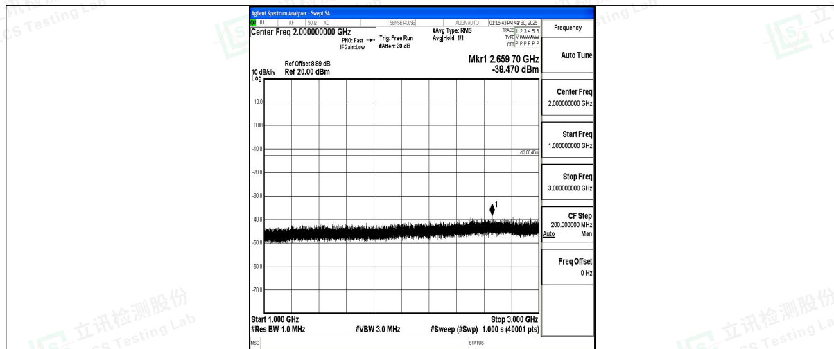
Band12_5MHz_16QAM_23095_1RB#0_1000~3000_1000~3000
