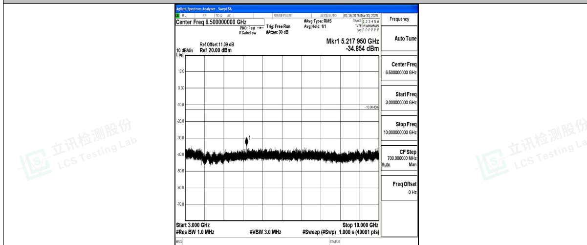
Band12_5MHz_QPSK_23095_1RB#0_3000~10000_3000~10000
