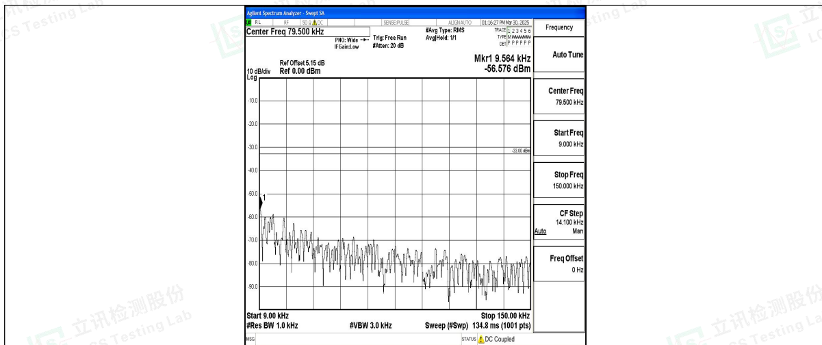
Band12_5MHz_16QAM_23095_1RB#0_0.009~0.15_0.009~0.15
