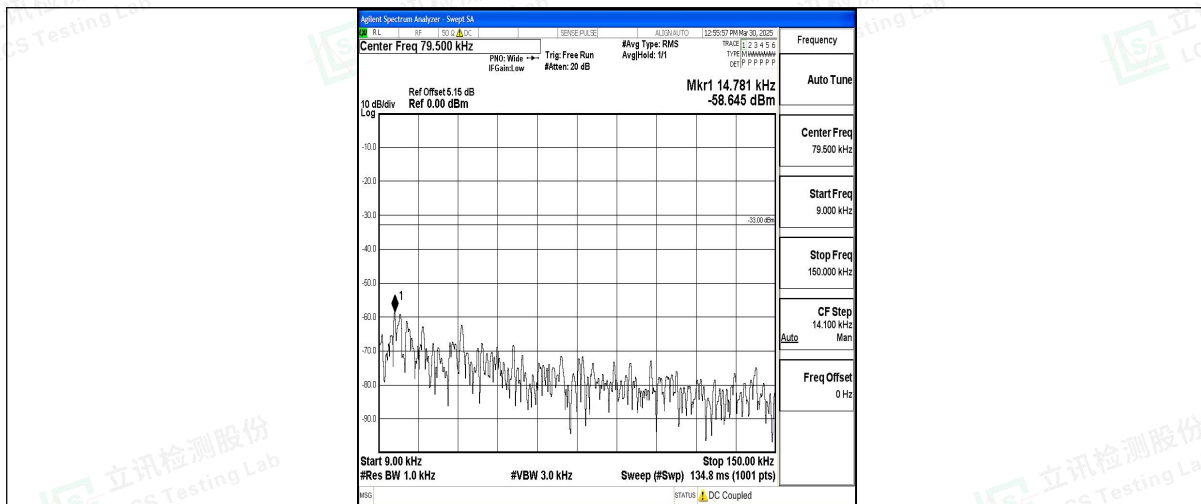
Band12_3MHz_QPSK_23025_1RB#0_0.009~0.15_0.009~0.15
