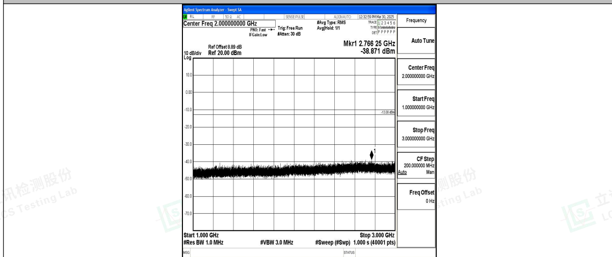
Band12_1.4MHz_16QAM_23173_1RB#0_1000~3000_1000~3000
