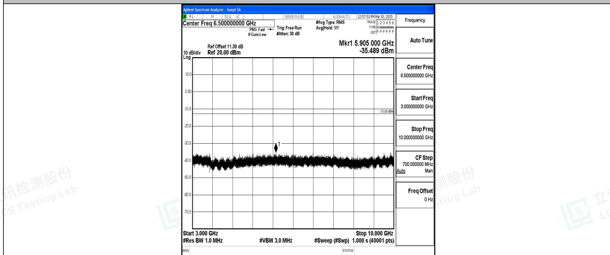
Band12_3MHz_16QAM_23095_1RB#0_3000~10000_3000~10000
