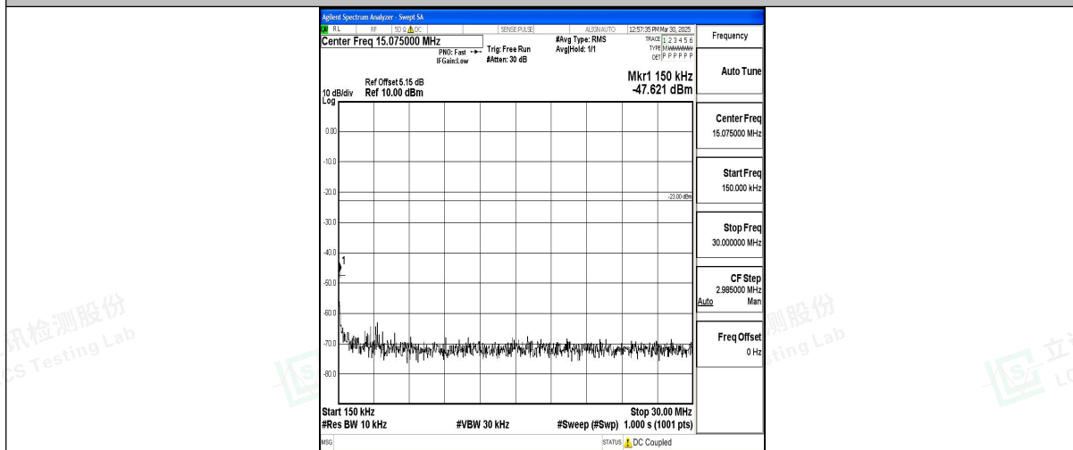
Band12_3MHz_16QAM_23095_1RB#0_0.15~30_0.15~30
