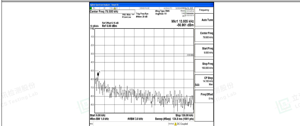
Band12_1.4MHz_16QAM_23173_1RB#0_0.009~0.15_0.009~0.15
