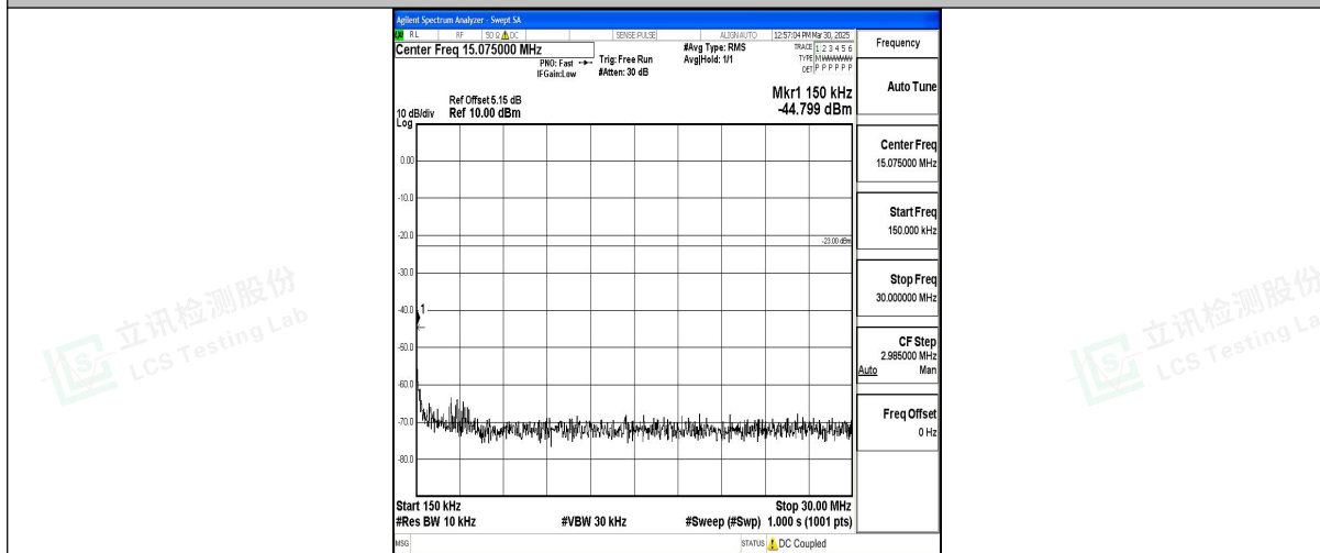
Band12_3MHz_QPSK_23095_1RB#0_0.15~30_0.15~30
