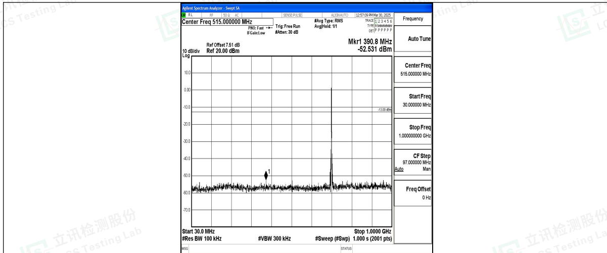
Band12_3MHz_QPSK_23095_1RB#0_30~1000_30~1000
