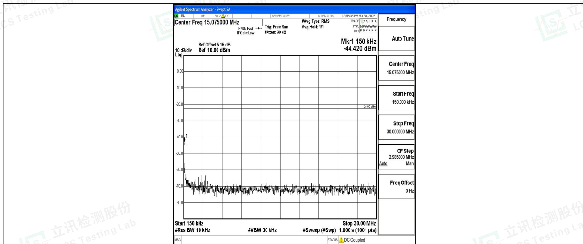
Band12_3MHz_16QAM_23025_1RB#0_0.15~30_0.15~30
