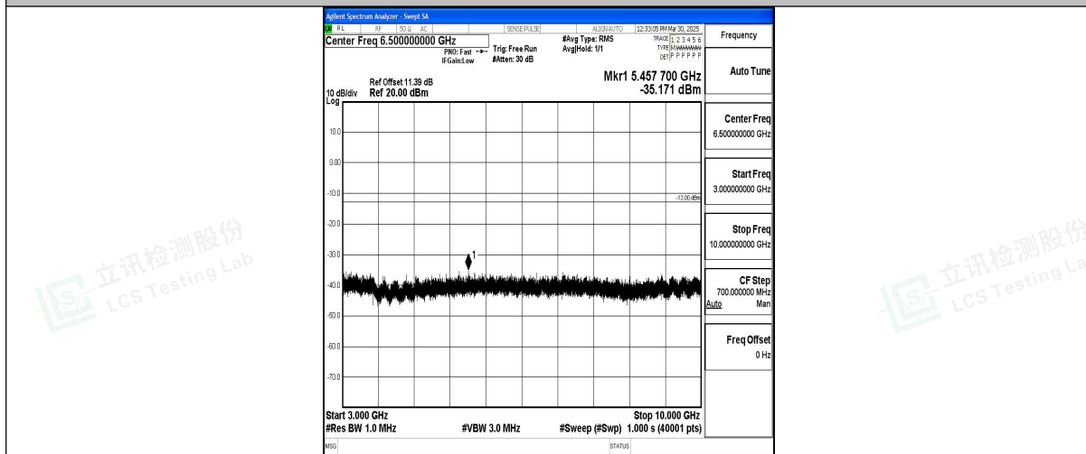
Band12_1.4MHz_16QAM_23173_1RB#0_3000~10000_3000~10000
