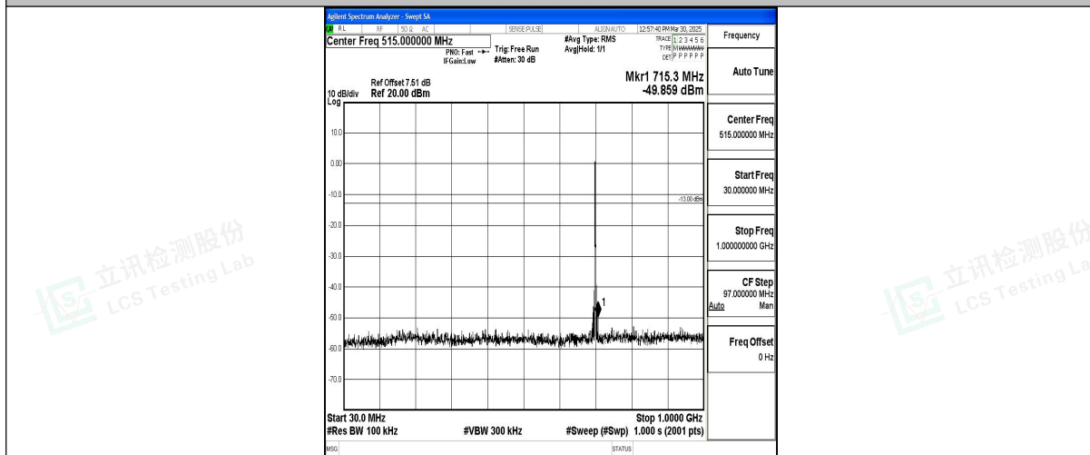
Band12_3MHz_16QAM_23095_1RB#0_30~1000_30~1000
