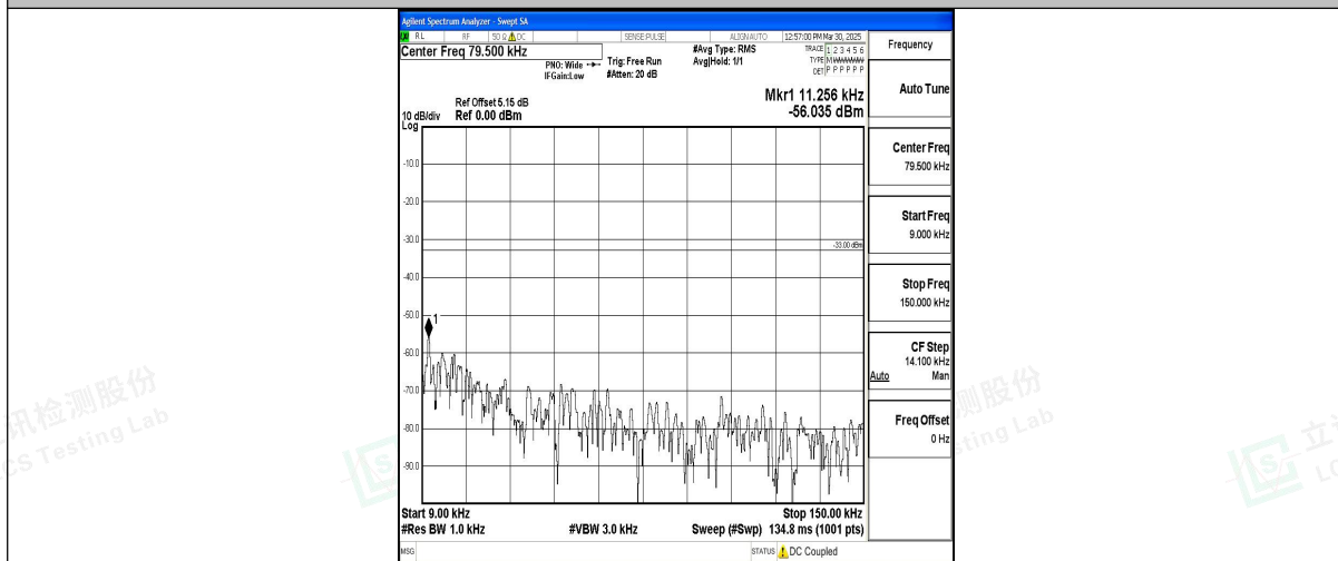
Band12_3MHz_QPSK_23095_1RB#0_0.009~0.15_0.009~0.15
