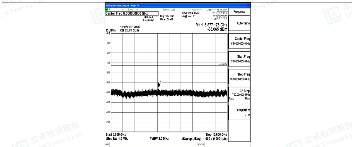
Band12_3MHz_16QAM_23025_1RB#0_3000~10000_3000~10000
