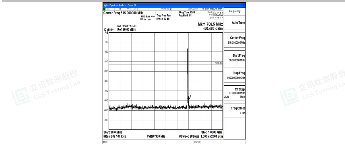
Band12_3MHz_QPSK_23025_1RB#0_30~1000_30~1000
