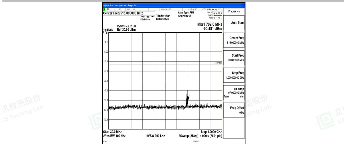
Band12_3MHz_16QAM_23025_1RB#0_30~1000_30~1000
