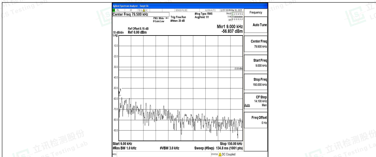
Band12_3MHz_16QAM_23095_1RB#0_0.009~0.15_0.009~0.15
