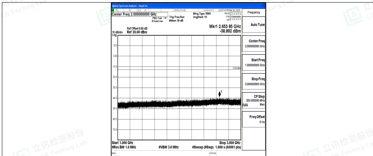
Band12_3MHz_16QAM_23095_1RB#0_1000~3000_1000~3000
