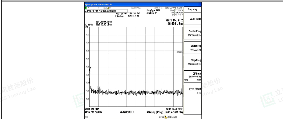
Band12_3MHz_QPSK_23025_1RB#0_0.15~30_0.15~30
