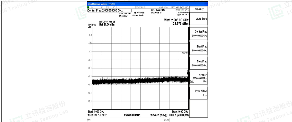
Band12_3MHz_QPSK_23025_1RB#0_1000~3000_1000~3000
