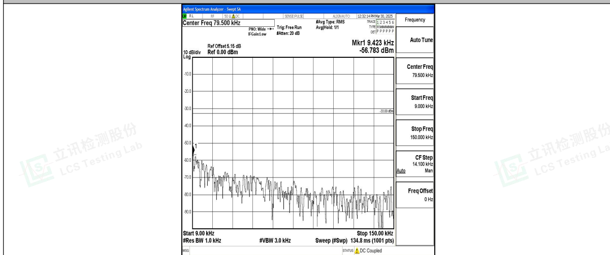
Band12_1.4MHz_QPSK_23173_1RB#0_0.009~0.15_0.009~0.15
