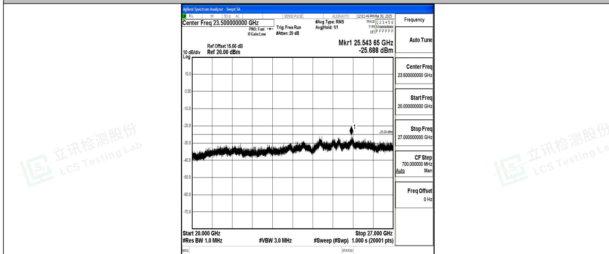
Band7_15MHz_16QAM_21375_1RB#0_20000~27000_20000~27000
