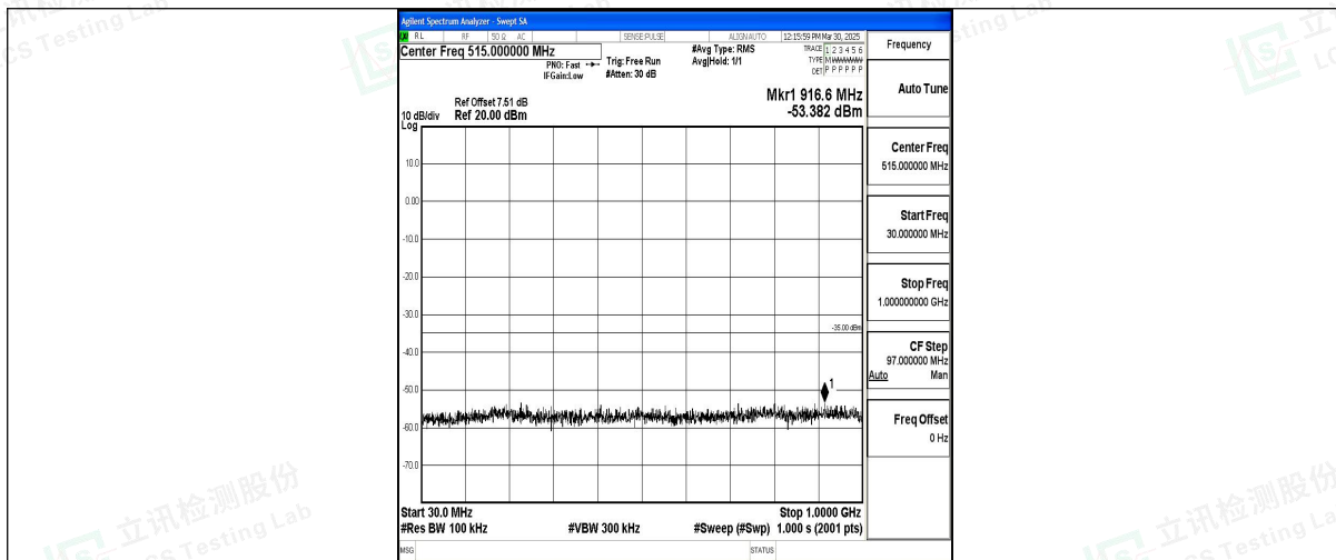
Band7_20MHz_QPSK_21100_1RB#0_30~1000_30~1000
