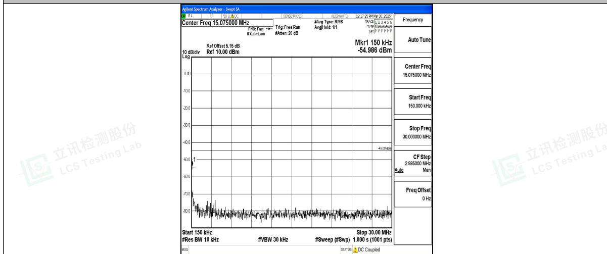
Band7_20MHz_16QAM_21350_1RB#0_0.15~30_0.15~30
