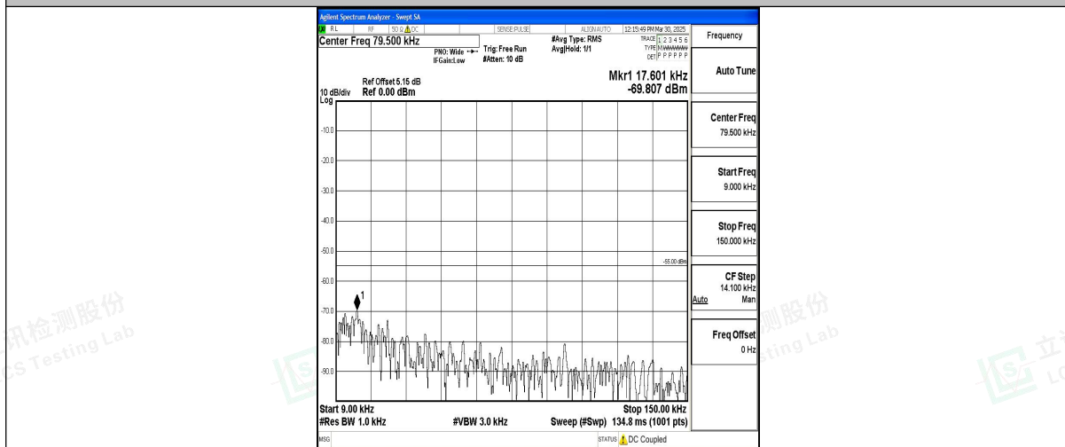
Band7_20MHz_QPSK_21100_1RB#0_0.009~0.15_0.009~0.15
