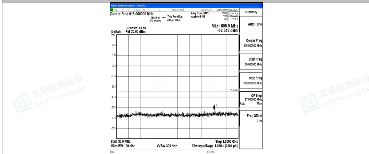
Band7_20MHz_QPSK_20850_1RB#0_30~1000_30~1000
