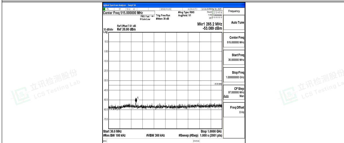
Band7_20MHz_16QAM_21100_1RB#0_30~1000_30~1000
