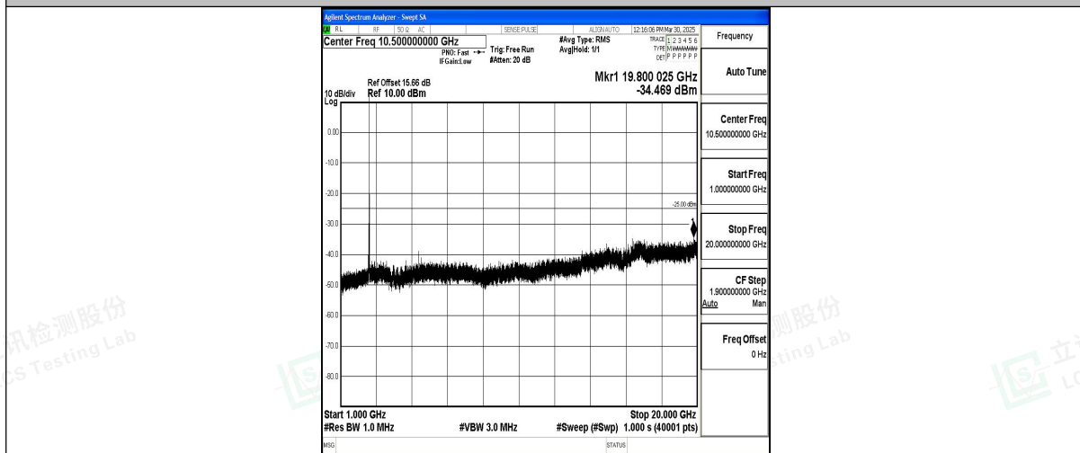
Band7_20MHz_QPSK_21100_1RB#0_1000~20000_1000~20000
