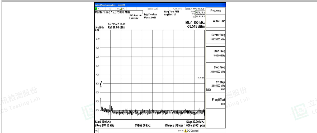
Band7_20MHz_16QAM_21100_1RB#0_0.15~30_0.15~30
