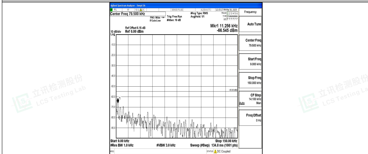
Band7_20MHz_16QAM_20850_1RB#0_0.009~0.15_0.009~0.15
