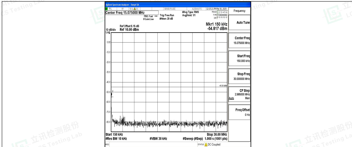
Band7_20MHz_16QAM_20850_1RB#0_0.15~30_0.15~30
