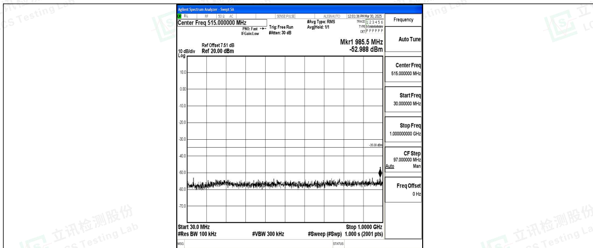
Band7_15MHz_16QAM_21375_1RB#0_30~1000_30~1000
