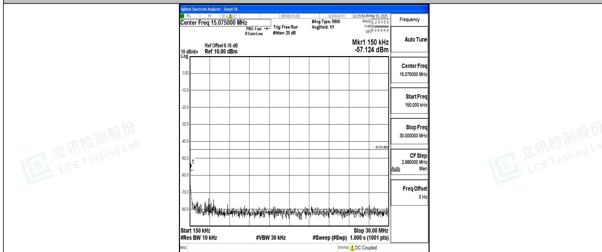
Band7_20MHz_QPSK_21100_1RB#0_0.15~30_0.15~30
