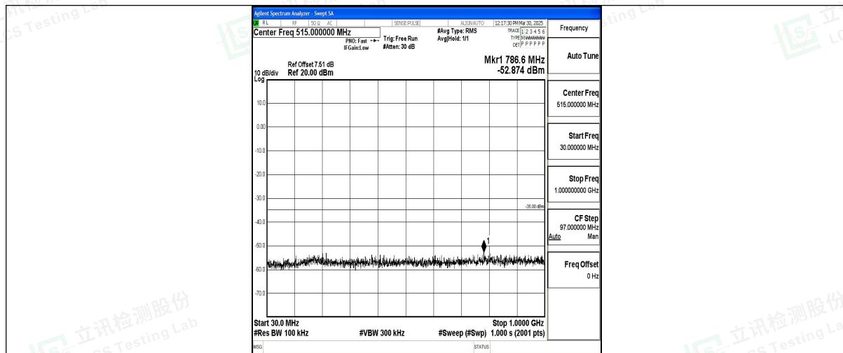
Band7_20MHz_16QAM_21350_1RB#0_30~1000_30~1000
