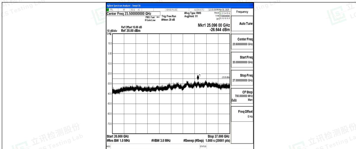
Band7_20MHz_16QAM_20850_1RB#0_20000~27000_20000~27000
