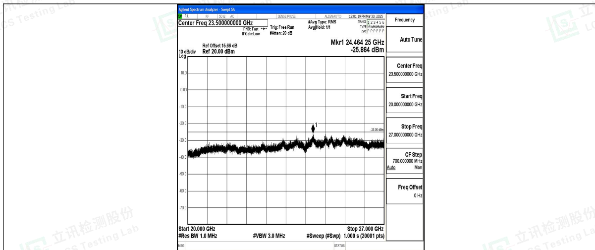
Band7_15MHz_QPSK_21375_1RB#0_20000~27000_20000~27000
