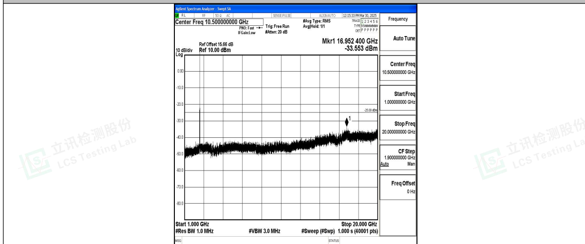
Band7_20MHz_16QAM_20850_1RB#0_1000~20000_1000~20000
