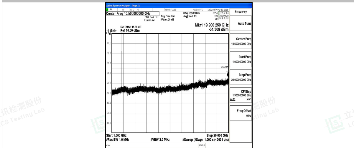
Band7_15MHz_16QAM_21375_1RB#0_1000~20000_1000~20000
