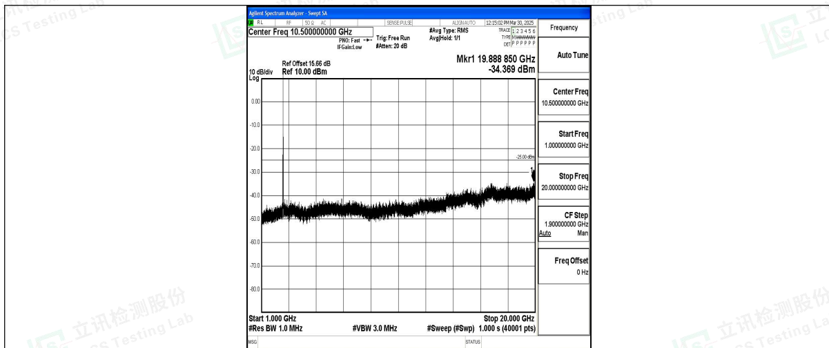
Band7_20MHz_QPSK_20850_1RB#0_1000~20000_1000~20000
