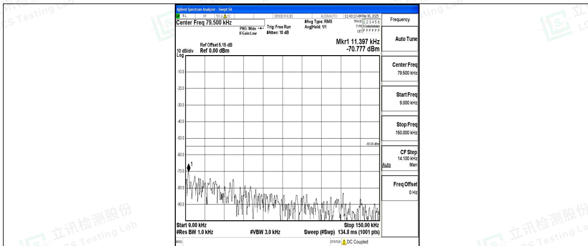
Band7_10MHz_QPSK_20800_1RB#0_0.009~0.15_0.009~0.15
