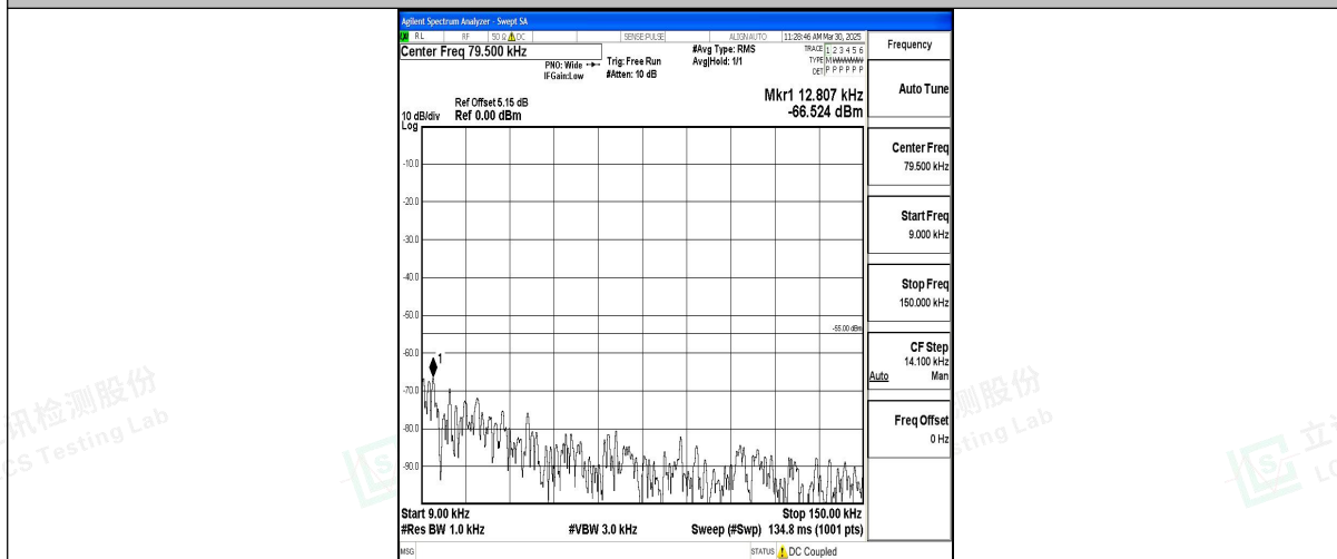
Band7_5MHz_16QAM_21425_1RB#0_0.009~0.15_0.009~0.15
