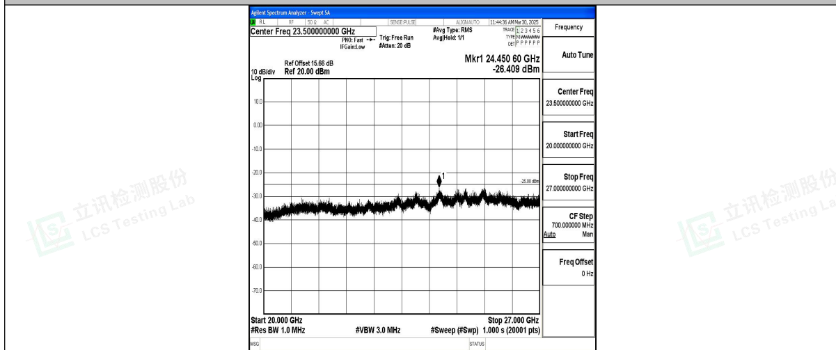
Band7_10MHz_QPSK_21100_1RB#0_20000~27000_20000~27000
