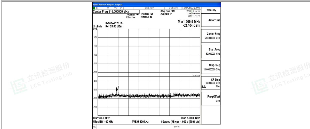
Band7_10MHz_QPSK_20800_1RB#0_30~1000_30~1000
