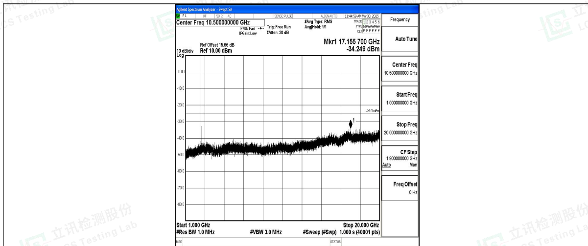
Band7_10MHz_16QAM_21100_1RB#0_1000~20000_1000~20000
