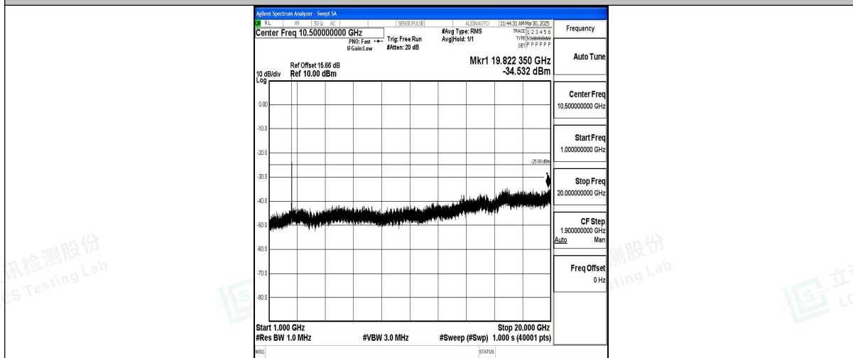
Band7_10MHz_QPSK_21100_1RB#0_1000~20000_1000~20000
