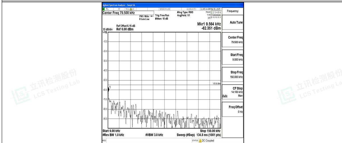
Band7_10MHz_QPSK_21400_1RB#0_0.009~0.15_0.009~0.15
