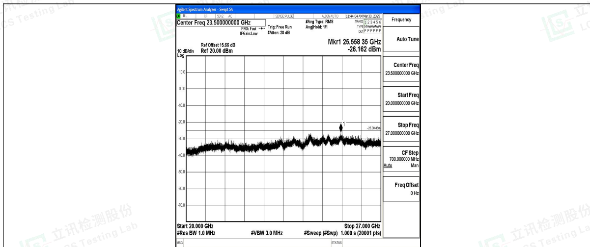
Band7_10MHz_16QAM_20800_1RB#0_20000~27000_20000~27000
