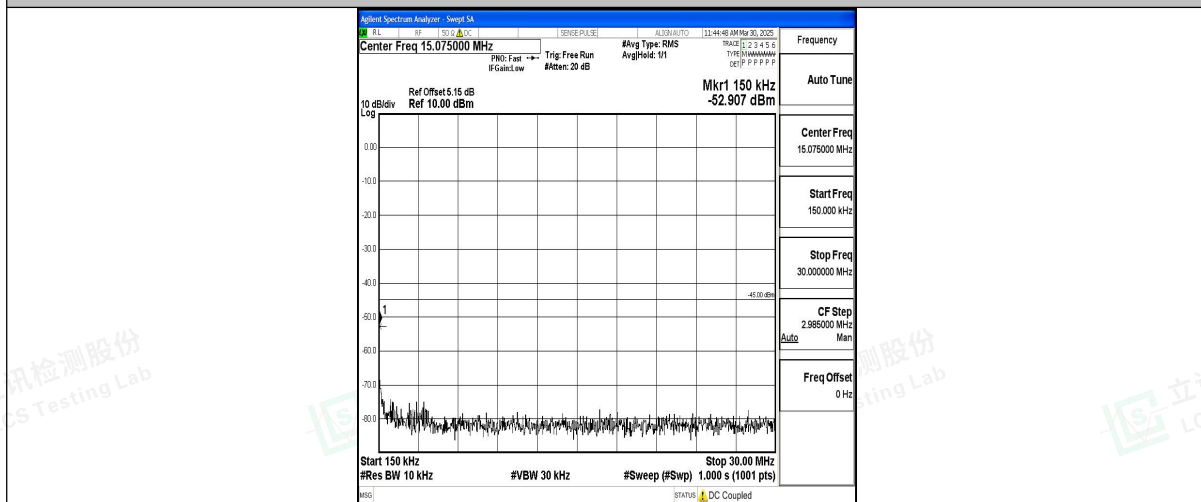
Band7_10MHz_16QAM_21100_1RB#0_0.15~30_0.15~30
