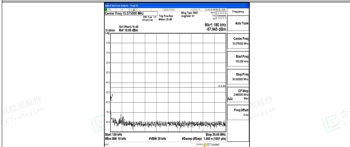
Band7_10MHz_QPSK_20800_1RB#0_0.15~30_0.15~30
