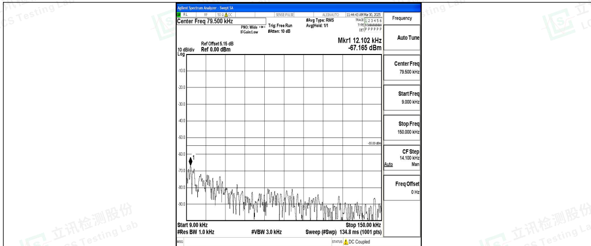
Band7_10MHz_16QAM_21100_1RB#0_0.009~0.15_0.009~0.15
