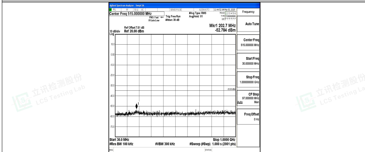
Band7_10MHz_16QAM_21100_1RB#0_30~1000_30~1000
