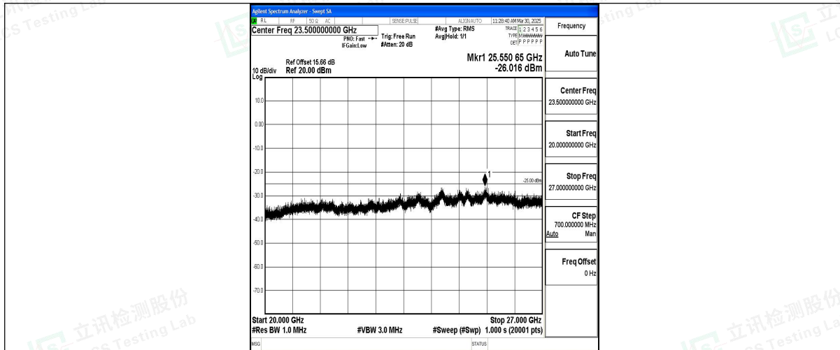
Band7_5MHz_QPSK_21425_1RB#0_20000~27000_20000~27000
