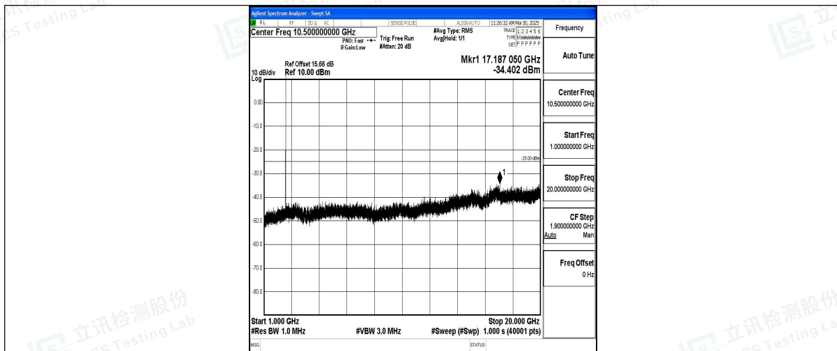
Band7_5MHz_QPSK_20775_1RB#0_1000~20000_1000~20000
