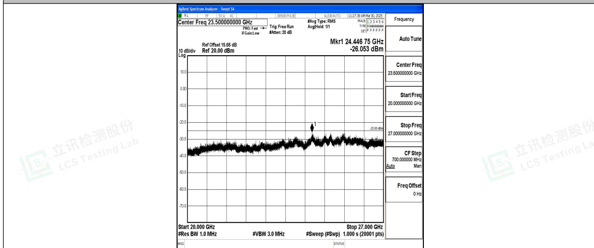
Band7_5MHz_QPSK_21100_1RB#0_20000~27000_20000~27000
