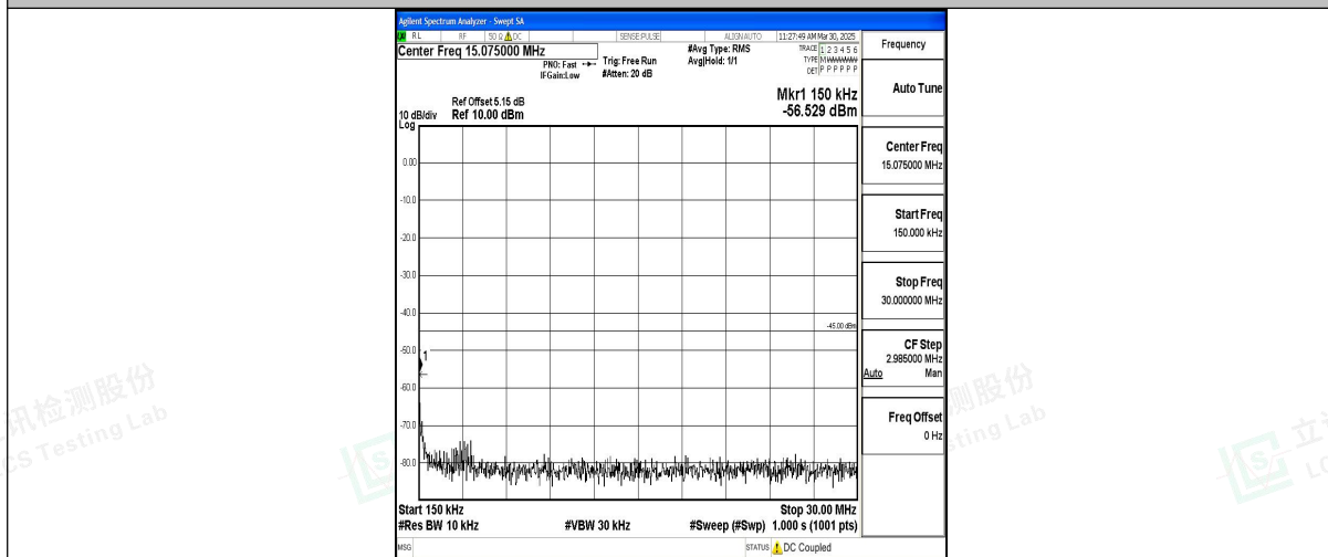
Band7_5MHz_16QAM_21100_1RB#0_0.15~30_0.15~30
