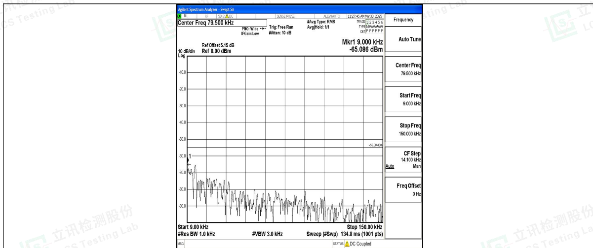
Band7_5MHz_16QAM_21100_1RB#0_0.009~0.15_0.009~0.15
