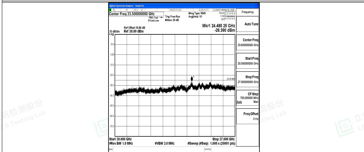
Band7_5MHz_16QAM_21100_1RB#0_20000~27000_20000~27000
