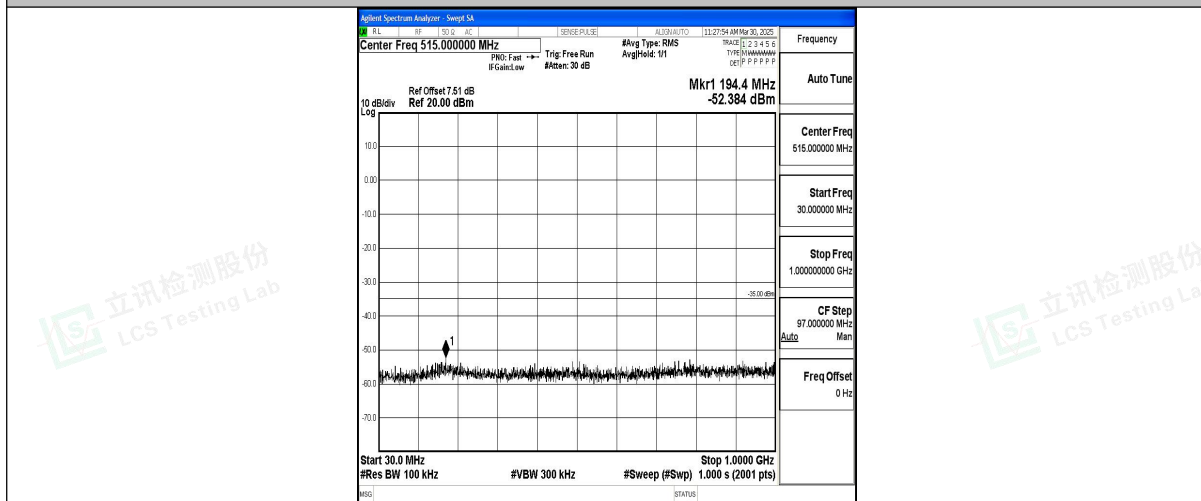
Band7_5MHz_16QAM_21100_1RB#0_30~1000_30~1000
