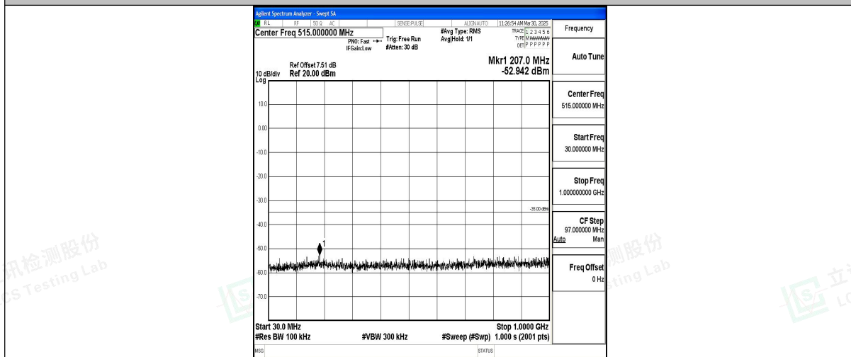
Band7_5MHz_16QAM_20775_1RB#0_30~1000_30~1000
