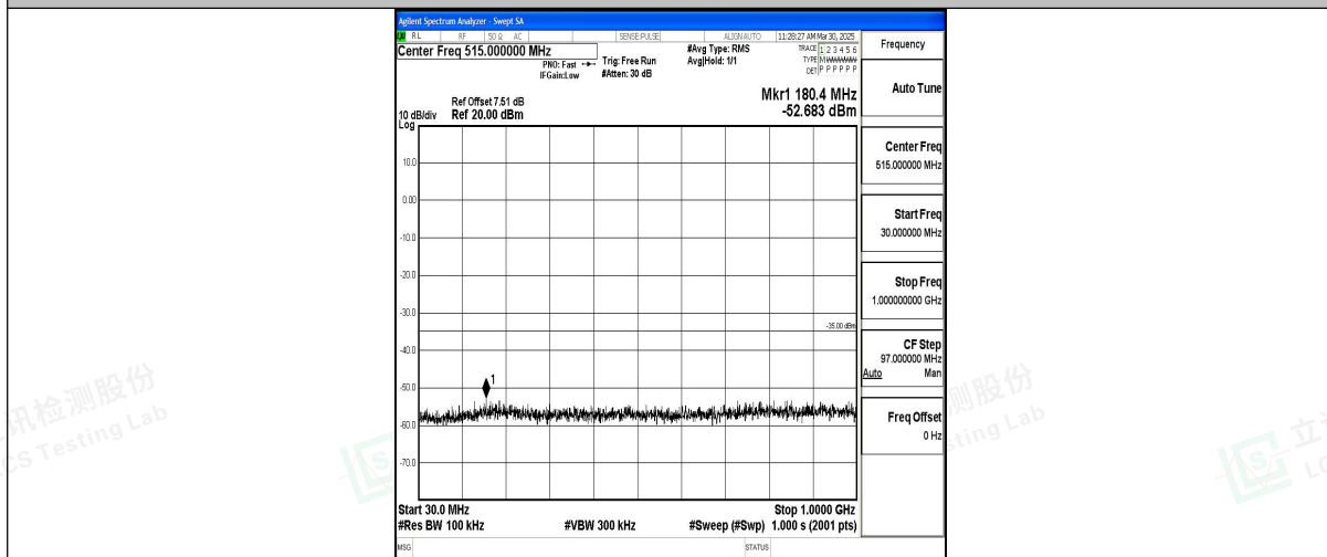
Band7_5MHz_QPSK_21425_1RB#0_30~1000.30~1000
