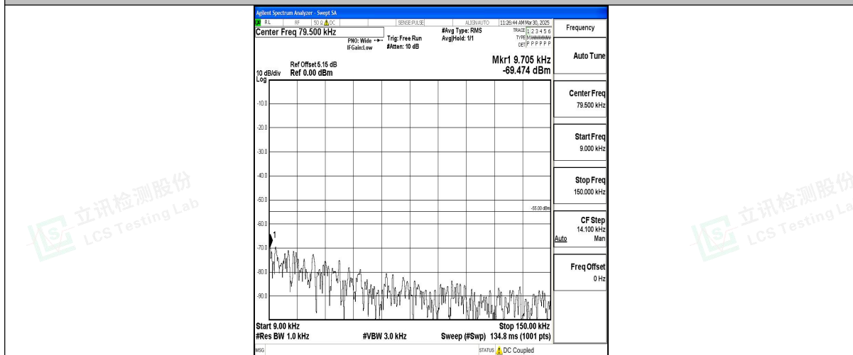
Band7_5MHz_16QAM_20775_1RB#0_0.009~0.15_0.009~0.15
