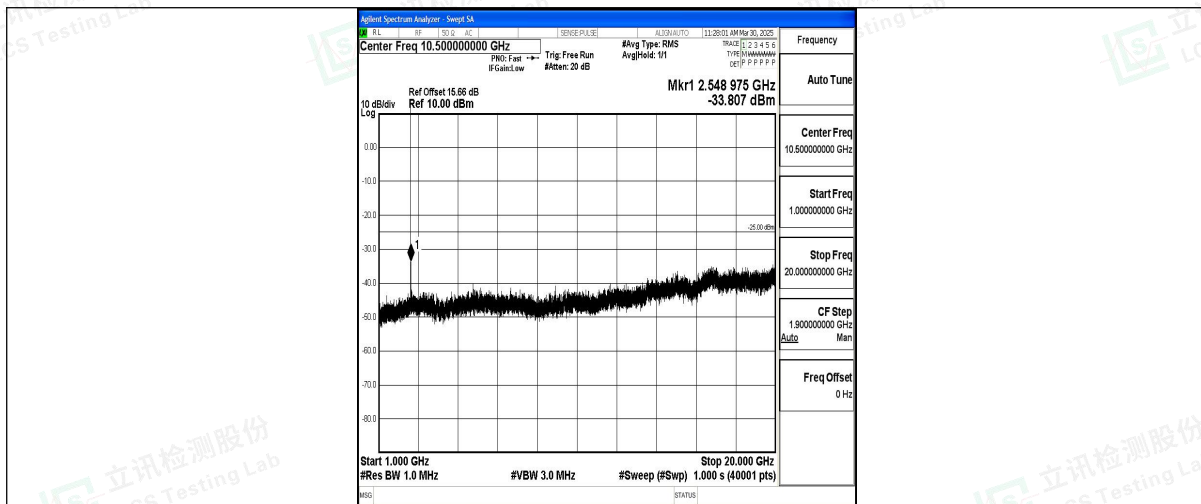
Band7_5MHz_16QAM_21100_1RB#0_1000~20000_1000~20000
