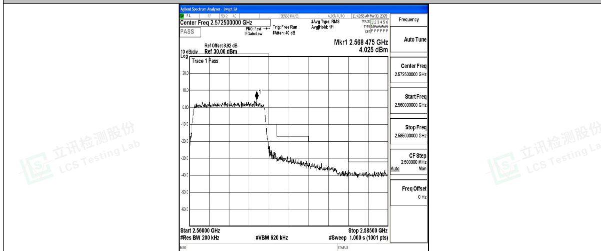
Band7_10MHz_QPSK_21400_50RB#0
