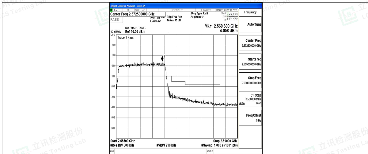
Band7_15MHz_QPSK_21375_75RB#0
