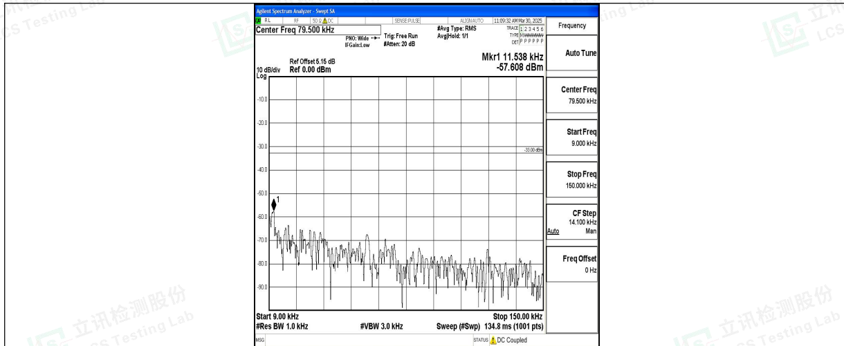
Band5_10MHz_16QAM_20525_1RB#0_0.009~0.15_0.009~0.15
