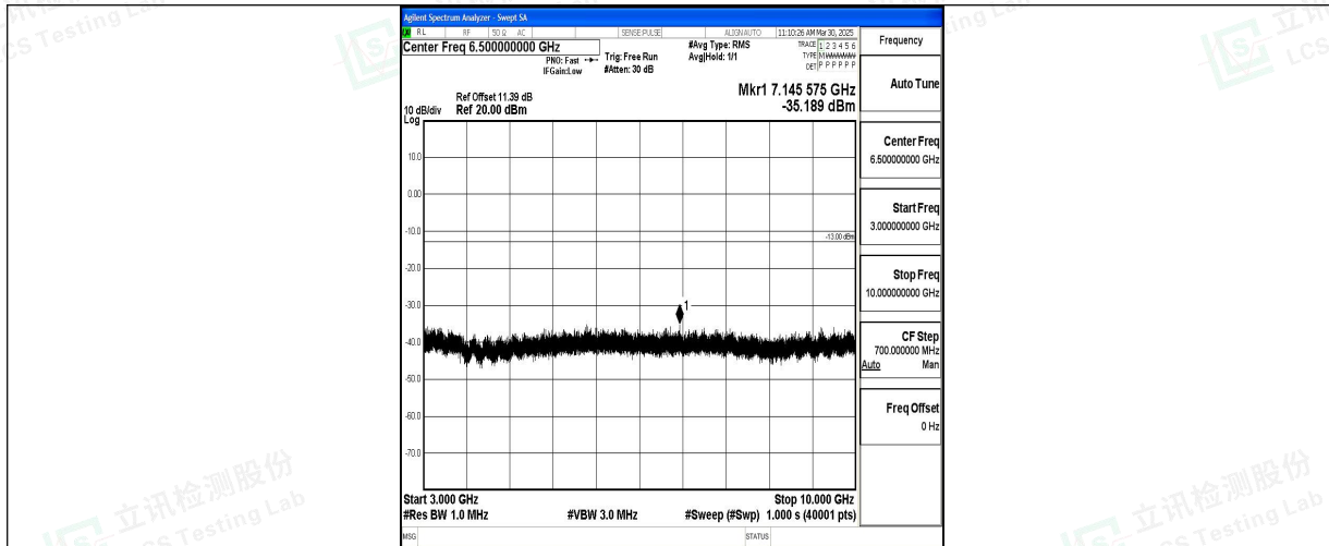
Band5_10MHz_QPSK_20600_1RB#0_3000~10000_3000~10000
