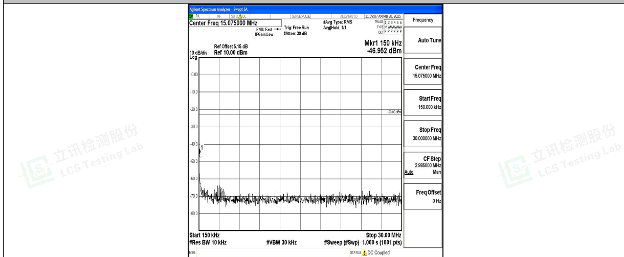
Band5_10MHz_QPSK_20525_1RB#0_0.15~30_0.15~30
