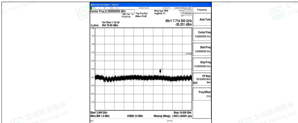
Band5_10MHz_16QAM_20450_1RB#0_3000~10000_3000~10000
