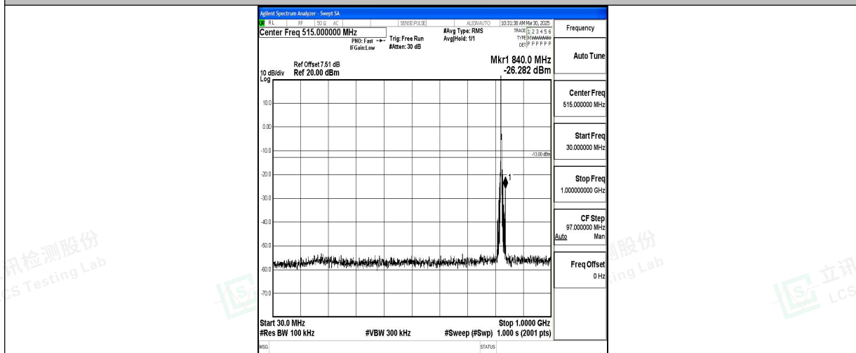
Band5_3MHz_16QAM_20415_1RB#0_30~1000_30~1000
