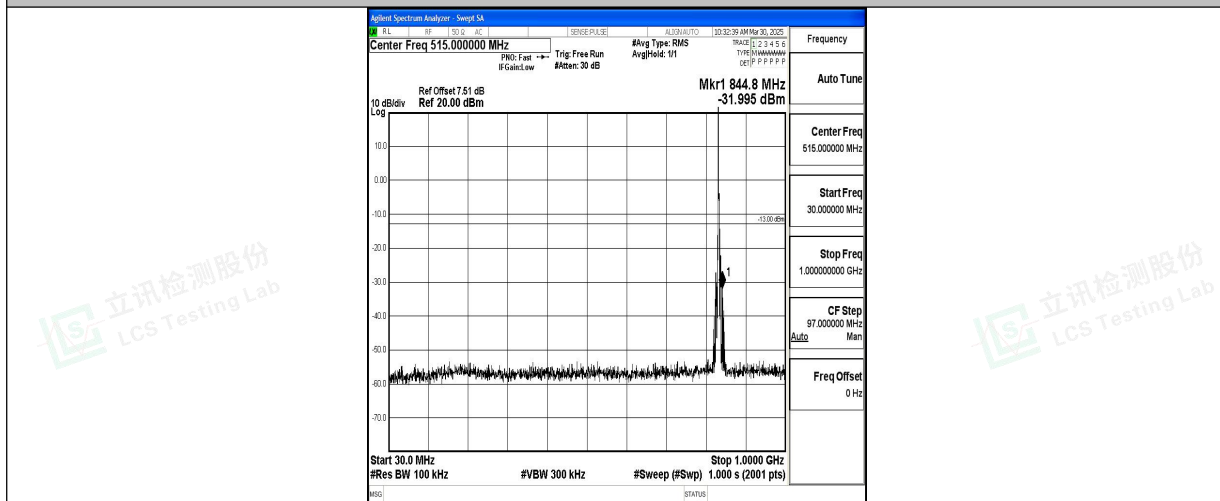
Band5_3MHz_16QAM_20525_1RB#0_30~1000_30~1000
