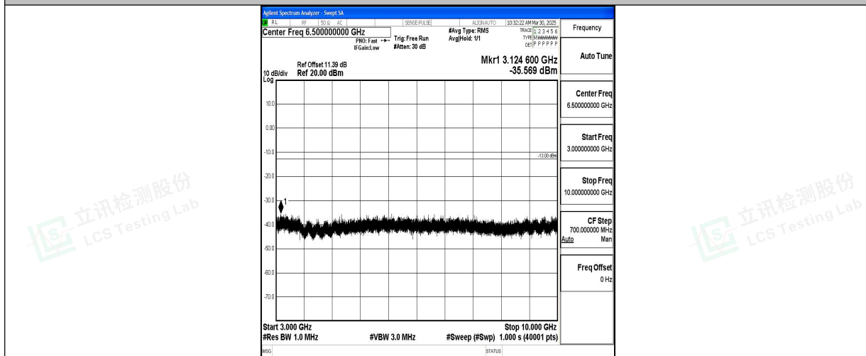
Band5_3MHz_QPSK_20525_1RB#0_3000~10000_3000~10000
