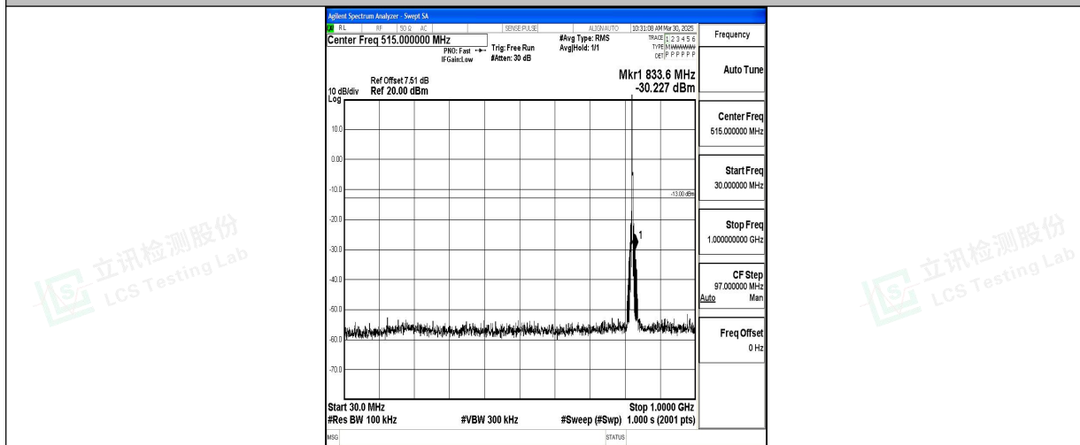
Band5_3MHz_QPSK_20415_1RB#0_30~1000_30~1000
