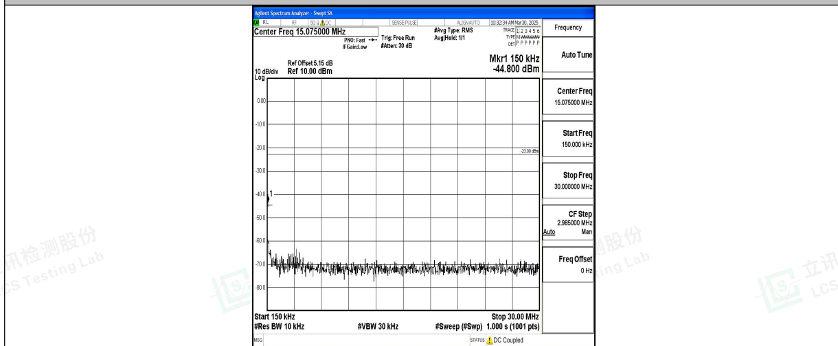
Band5_3MHz_16QAM_20525_1RB#0_0.15~30_0.15~30
