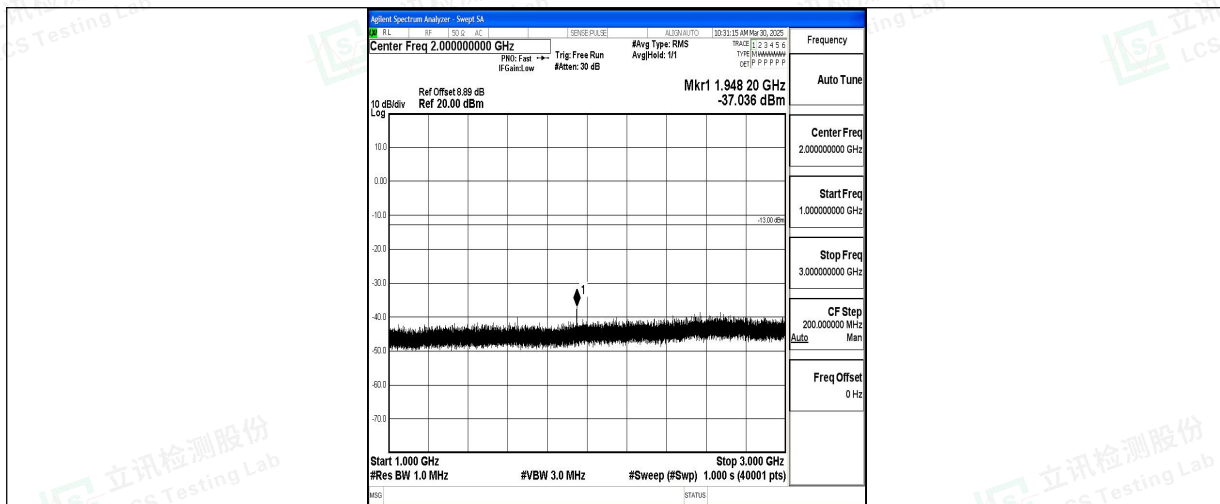
Band5_3MHz_QPSK_20415_1RB#0_1000~3000_1000~3000
