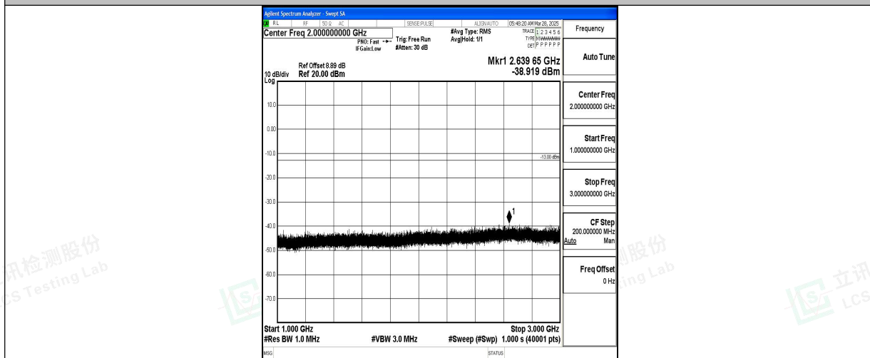
Band5_1.4MHz_16QAM_20643_1RB#0_1000~3000_1000~3000
