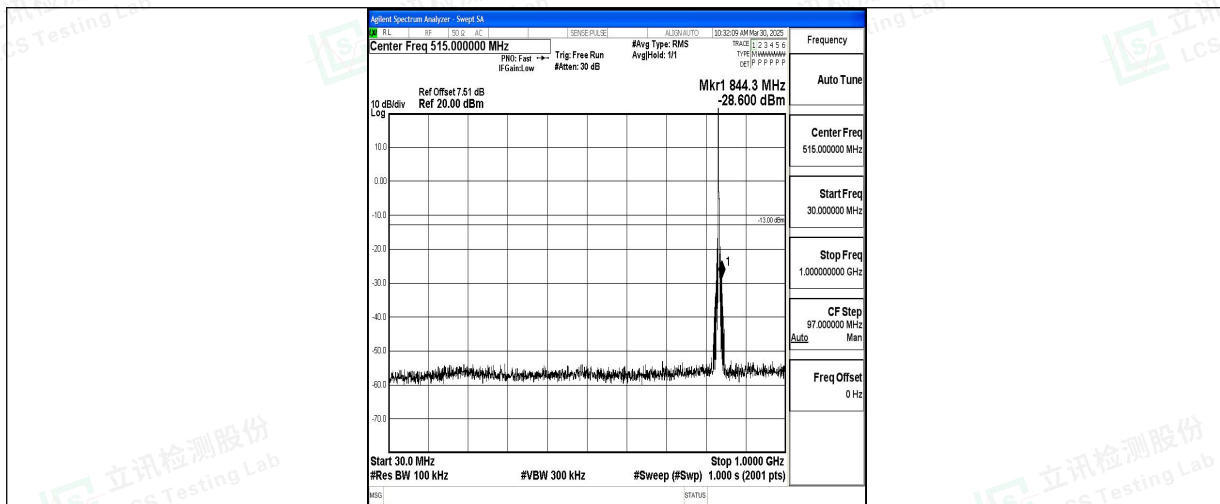
Band5_3MHz_QPSK_20525_1RB#0_30~1000_30~1000
