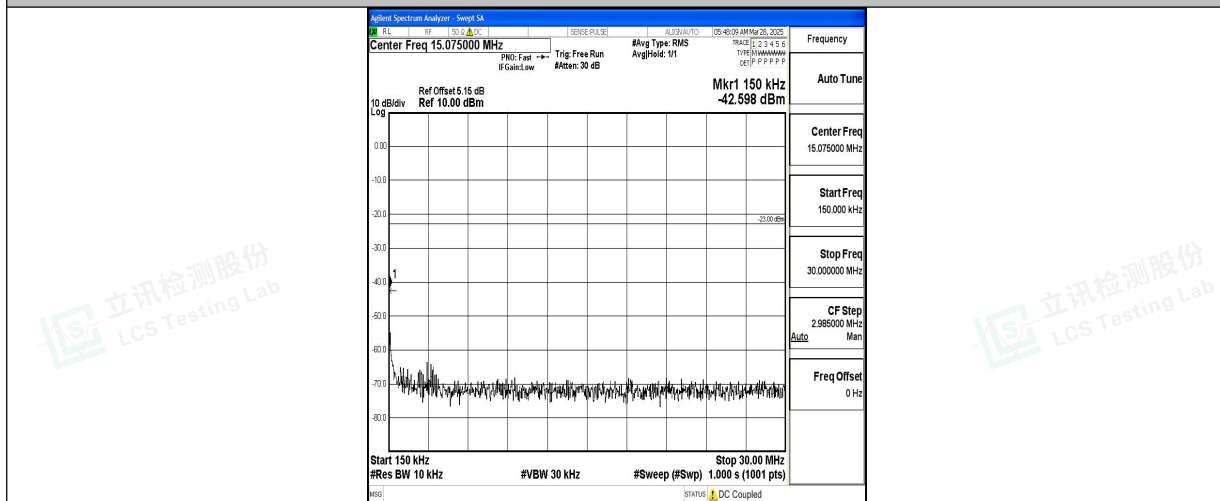
Band5_1.4MHz_16QAM_20643_1RB#0_0.15~30_0.15~30
