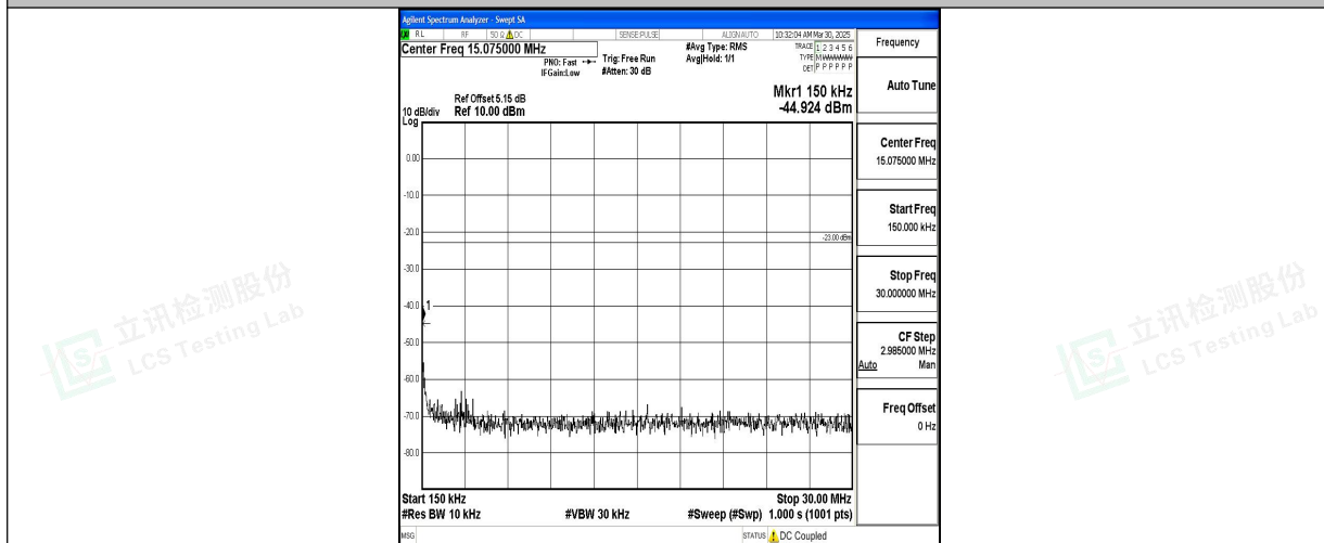
Band5_3MHz_QPSK_20525_1RB#0_0.15~30_0.15~30
