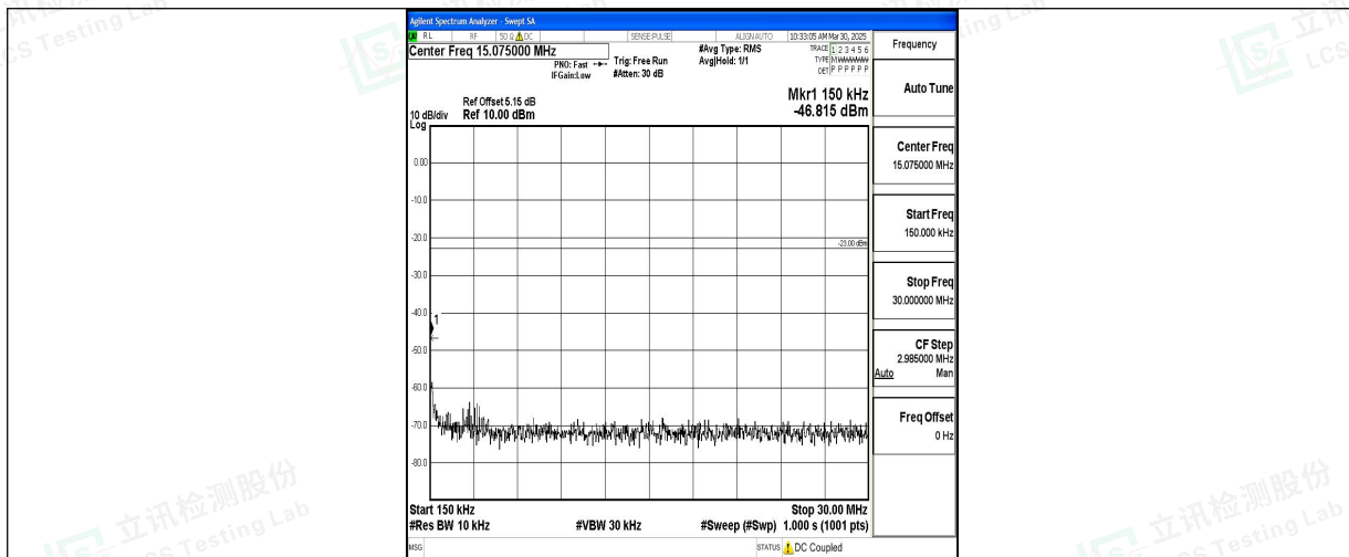
Band5_3MHz_QPSK_20635_1RB#0_0.15~30_0.15~30
