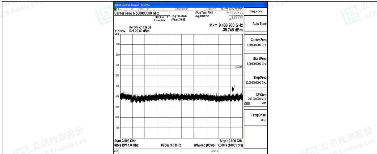
Band5_1.4MHz_QPSK_20643_1RB#0_3000~10000_3000~10000
