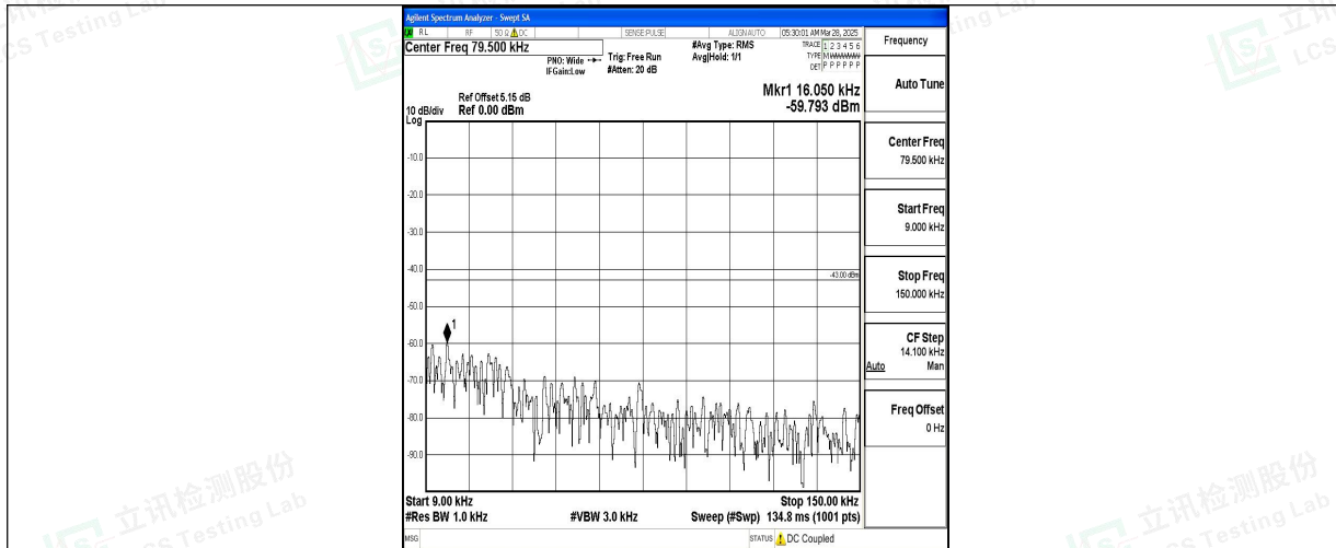
Band4_20MHz_16QAM_20050_1RB#0_0.009~0.15_0.009~0.15
