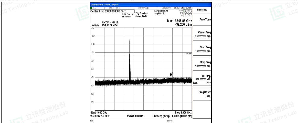
Band4_20MHz_16QAM_20050_1RB#0_1000~3000_1000~3000
