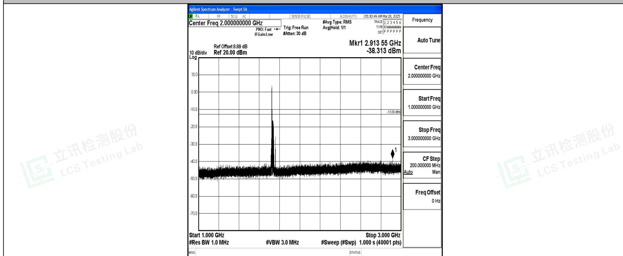
Band4_20MHz_QPSK_20175_1RB#0_1000~3000_1000~3000
