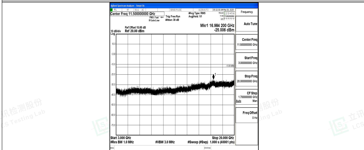
Band4_20MHz_QPSK_20300_1RB#0_3000~20000_3000~20000
