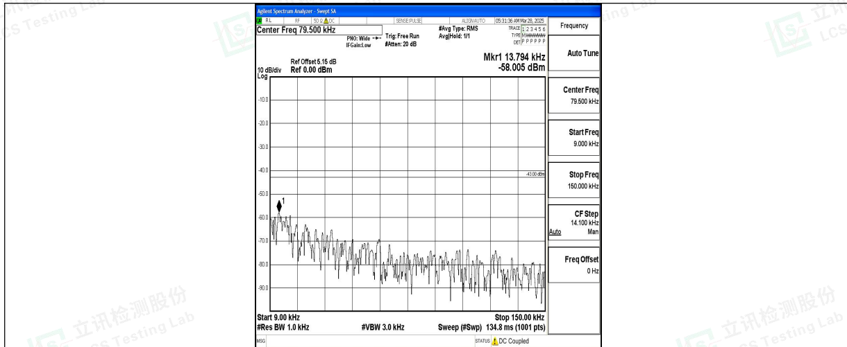
Band4_20MHz_QPSK_20300_1RB#0_0.009~0.15_0.009~0.15
