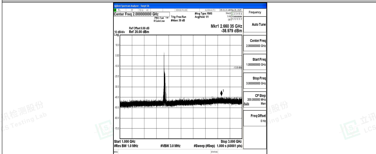
Band4_20MHz_16QAM_20175_1RB#0_1000~3000_1000~3000
