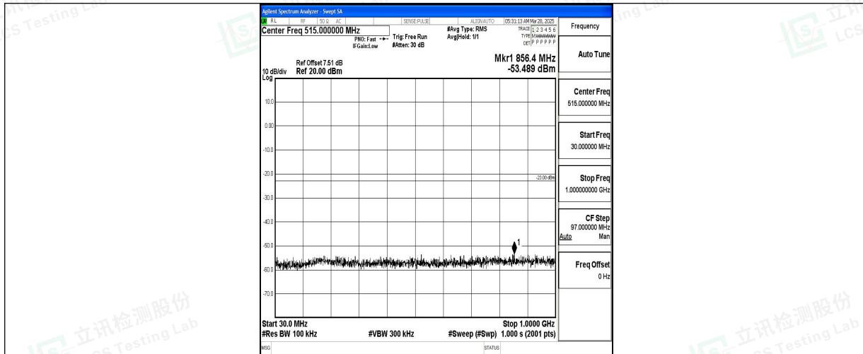
Band4_20MHz_16QAM_20175_1RB#0_30~1000_30~1000
