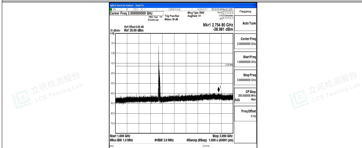
Band4_20MHz_16QAM_20300_1RB#0_1000~3000_1000~3000
