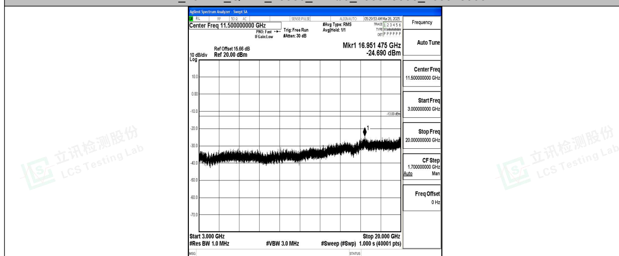
Band4_20MHz_QPSK_20050_1RB#0_3000~20000_3000~20000
