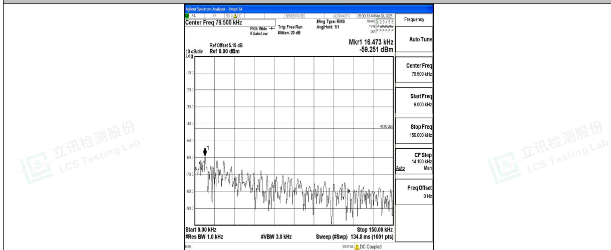
Band4_20MHz_QPSK_20175_1RB#0_0.009~0.15_0.009~0.15
