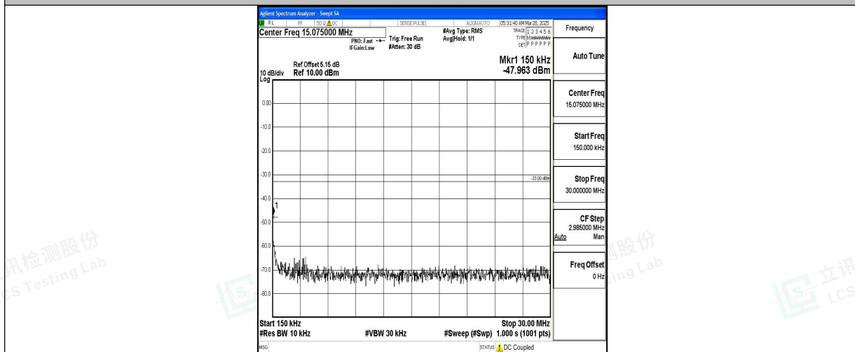
Band4_20MHz_QPSK_20300_1RB#0_0.15~30_0.15~30
