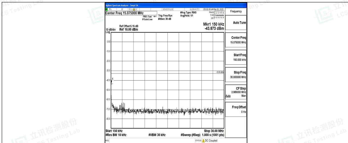
Band4_20MHz_QPSK_20175_1RB#0_0.15~30_0.15~30
