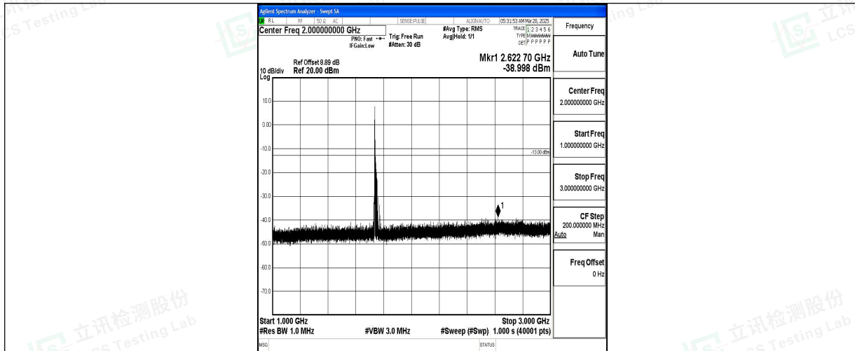
Band4_20MHz_QPSK_20300_1RB#0_1000~3000_1000~3000
