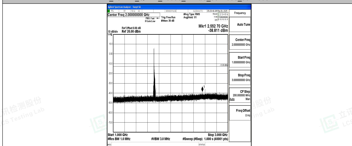
Band4_20MHz_QPSK_20050_1RB#0_1000~3000_1000~3000
