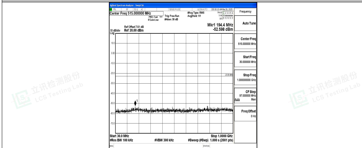
Band4_20MHz_16QAM_20050_1RB#0_30~1000_30~1000
