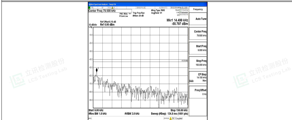
Band4_20MHz_16QAM_20300_1RB#0_0.009~0.15_0.009~0.15
