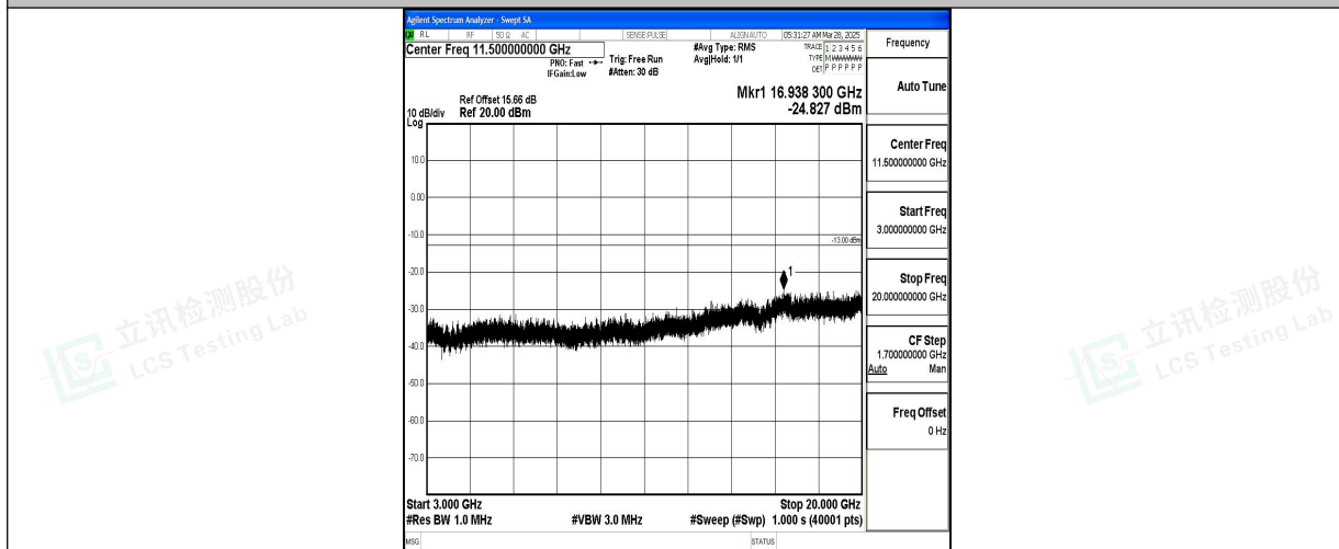
Band4_20MHz_16QAM_20175_1RB#0_3000~20000_3000~20000
