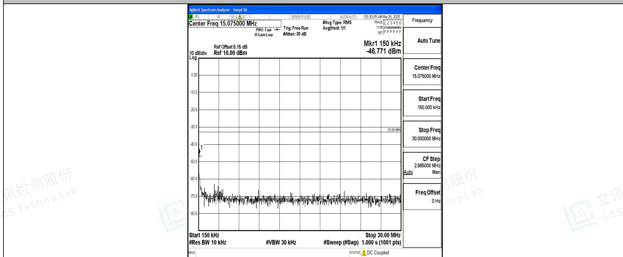
Band4_20MHz_16QAM_20050_1RB#0_0.15~30_0.15~30
