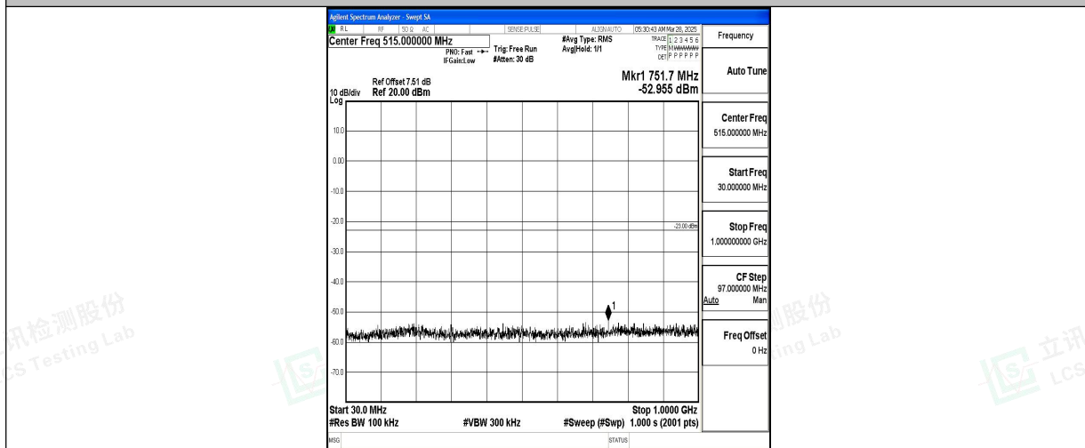
Band4_20MHz_QPSK_20175_1RB#0_30~1000_30~1000
