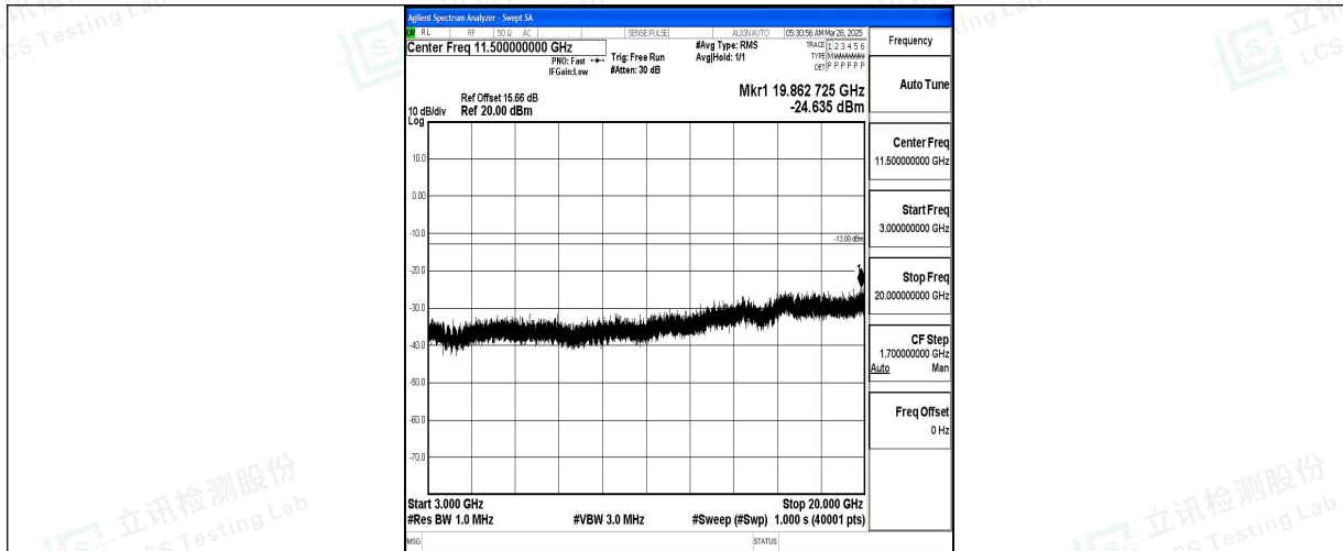
Band4_20MHz_QPSK_20175_1RB#0_3000~20000_3000~20000
