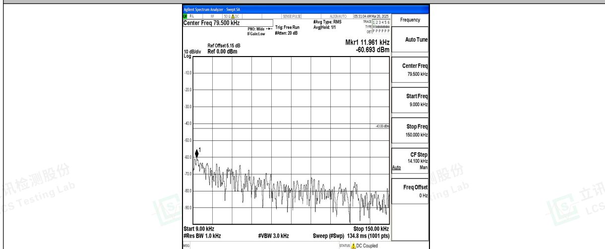
Band4_20MHz_16QAM_20175_1RB#0_0.009~0.15_0.009~0.15
