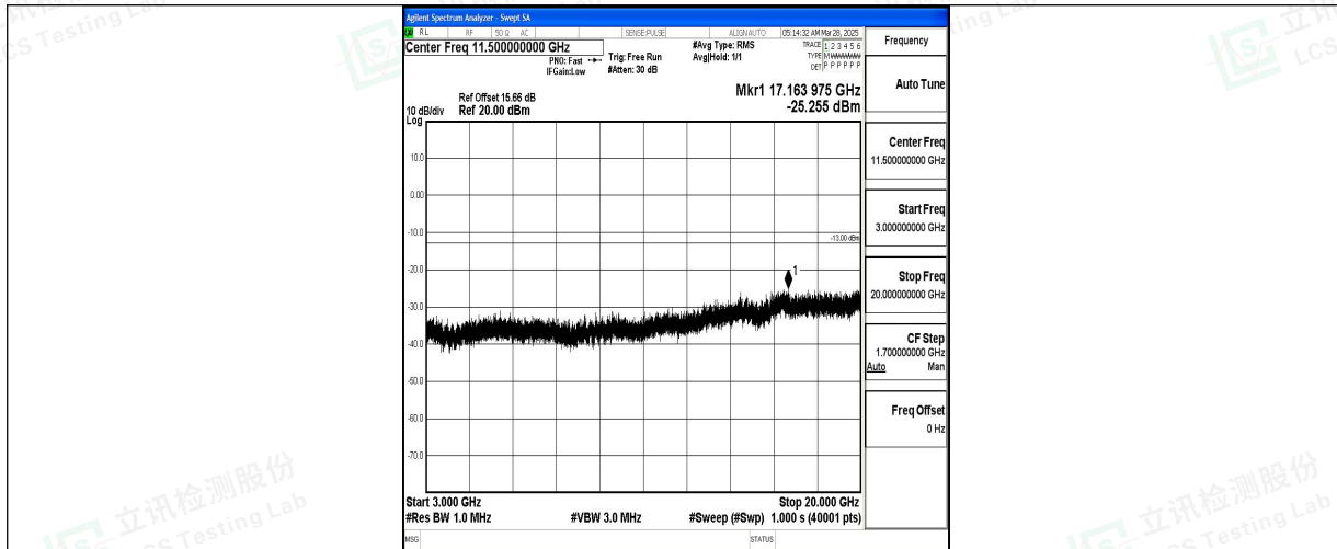
Band4_15MHz_QPSK_20175_1RB#0_3000~20000_3000~20000
