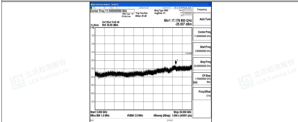
Band4_15MHz_QPSK_20025_1RB#0_3000~20000_3000~20000
