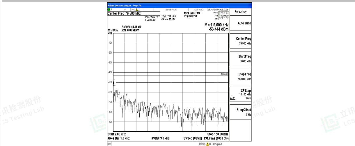
Band4_15MHz_16QAM_20175_1RB#0_0.009~0.15_0.009~0.15
