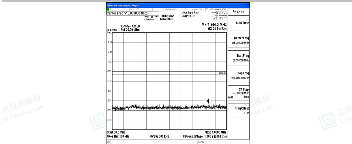
Band4_15MHz_16QAM_20325_1RB#0_30~1000_30~1000
