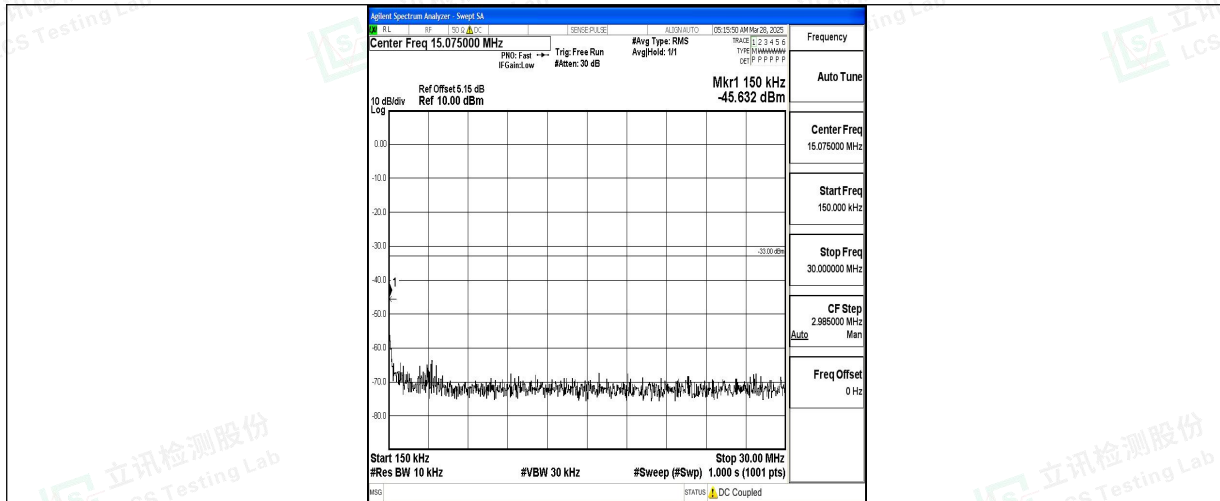
Band4_15MHz_16QAM_20325_1RB#0_0.15~30_0.15~30
