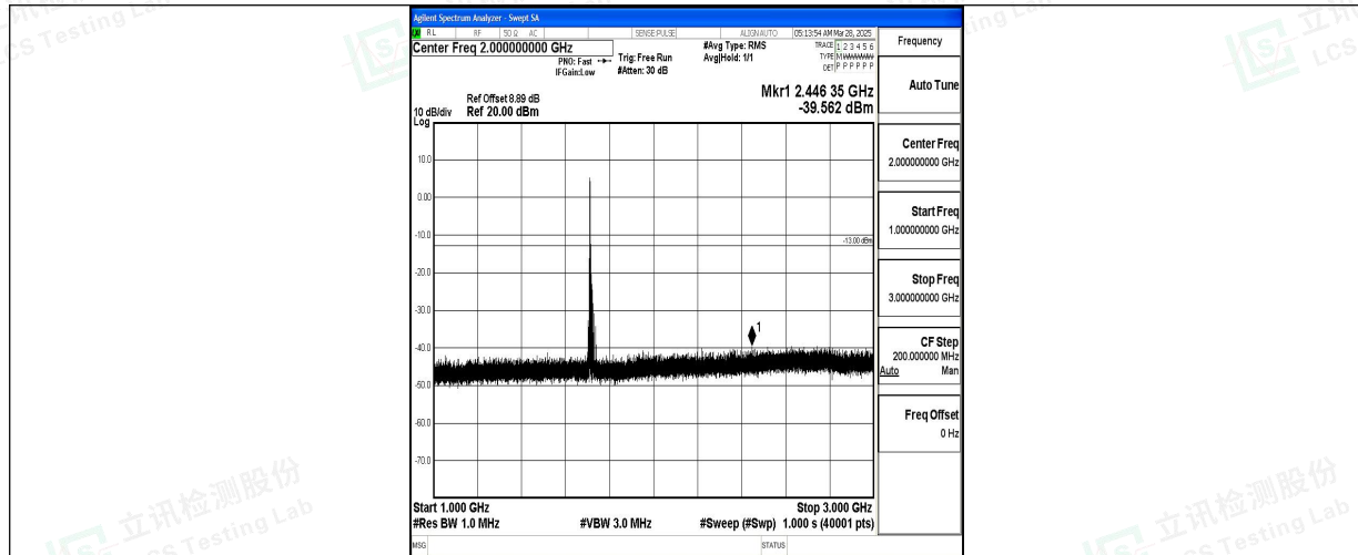
Band4_15MHz_16QAM_20025_1RB#0_1000~3000_1000~3000
