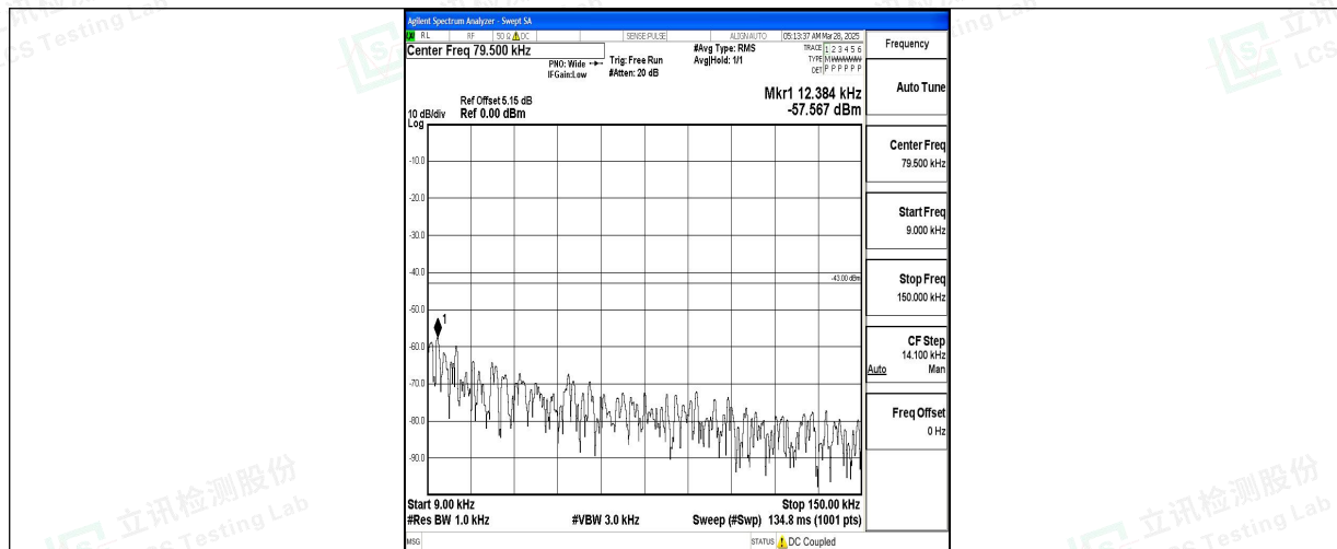
Band4_15MHz_16QAM_20025_1RB#0_0.009~0.15_0.009~0.15
