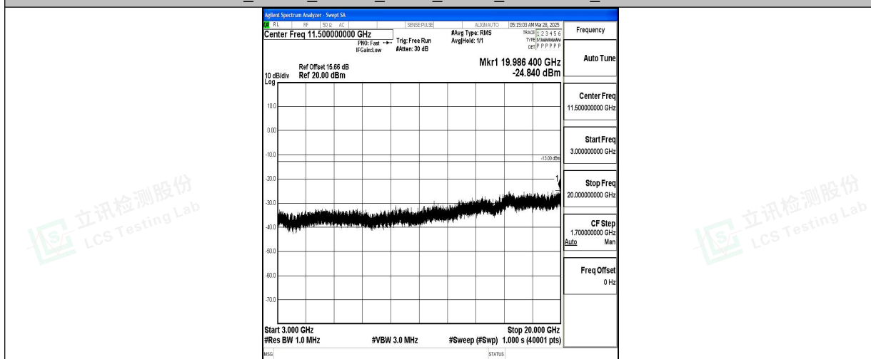
Band4_15MHz_16QAM_20175_1RB#0_3000~20000_3000~20000
