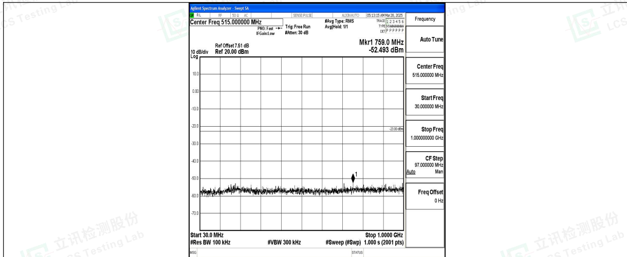
Band4_15MHz_QPSK_20025_1RB#0_30~1000_30~1000
