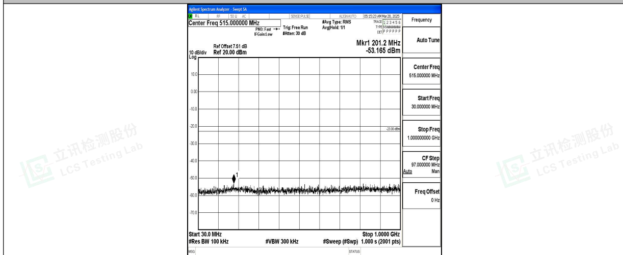
Band4_15MHz_QPSK_20325_1RB#0_30~1000_30~1000
