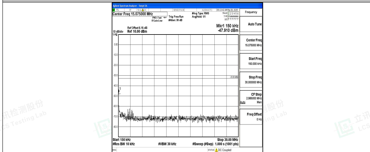
Band4_15MHz_16QAM_20025_1RB#0_0.15~30_0.15~30
