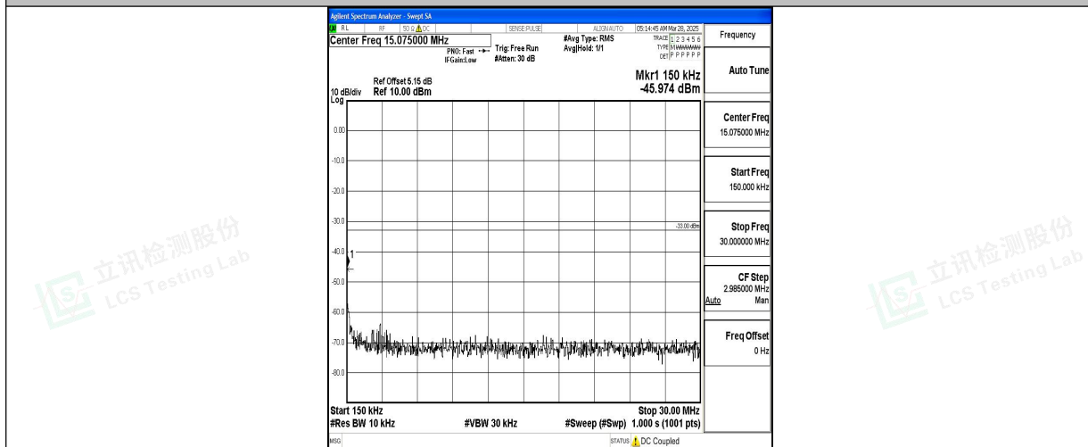
Band4_15MHz_16QAM_20175_1RB#0_0.15~30_0.15~30
