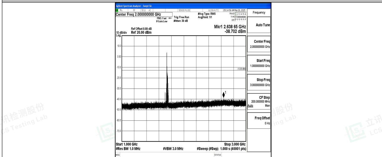
Band4_15MHz_16QAM_20175_1RB#0_1000~3000_1000~3000
