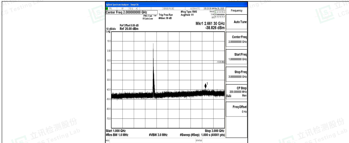
Band4_15MHz_QPSK_20325_1RB#0_1000~3000_1000~3000
