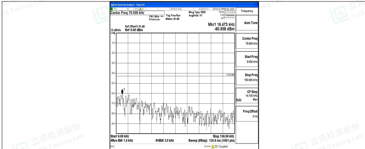
Band4_15MHz_QPSK_20325_1RB#0_0.009~0.15_0.009~0.15
