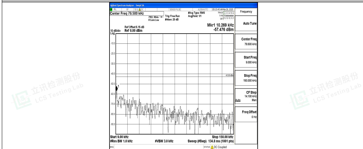
Band4_15MHz_16QAM_20325_1RB#0_0.009~0.15_0.009~0.15
