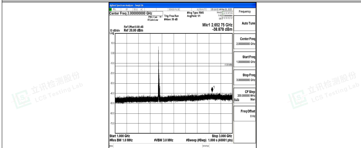
Band4_15MHz_16QAM_20325_1RB#0_1000~3000_1000~3000
