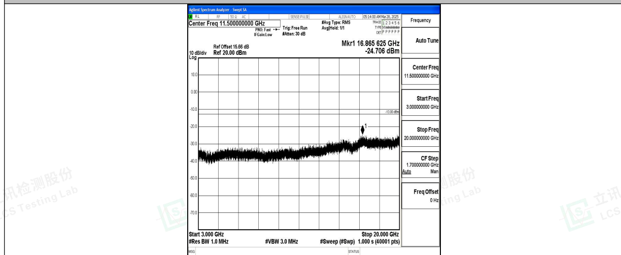
Band4_15MHz_16QAM_20025_1RB#0_3000~20000_3000~20000
