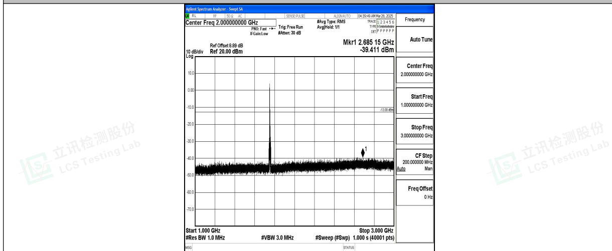
Band4_5MHz_16QAM_20375_1RB#0_1000~3000_1000~3000
