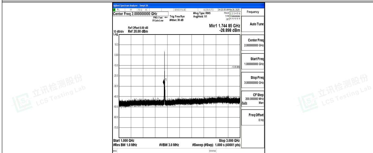
Band4_3MHz_16QAM_20385_1RB#0_1000~3000_1000~3000
