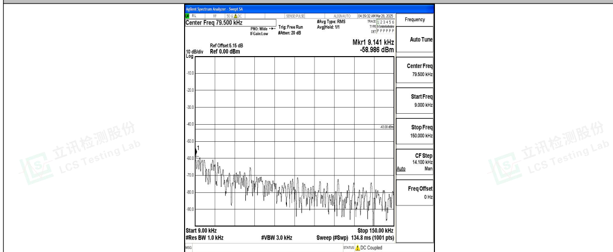
Band4_5MHz_16QAM_20375_1RB#0_0.009~0.15_0.009~0.15
