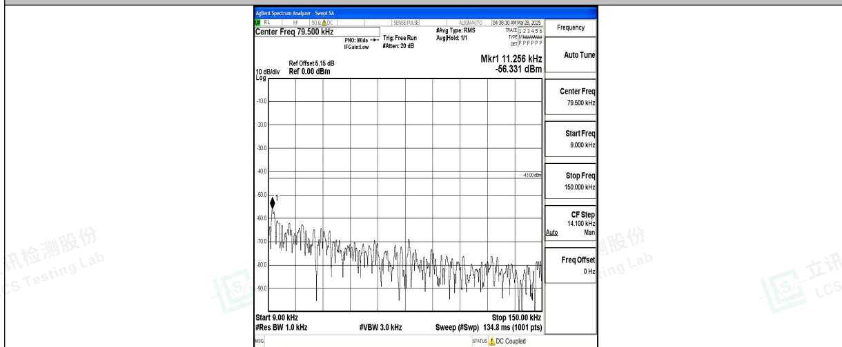
Band4_5MHz_16QAM_20175_1RB#0_0.009~0.15_0.009~0.15
