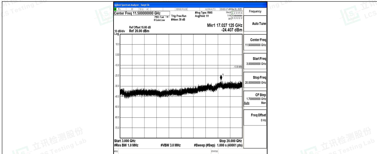
Band2_10MHz_16QAM_18900_1RB#0_3000~20000_3000~20000
