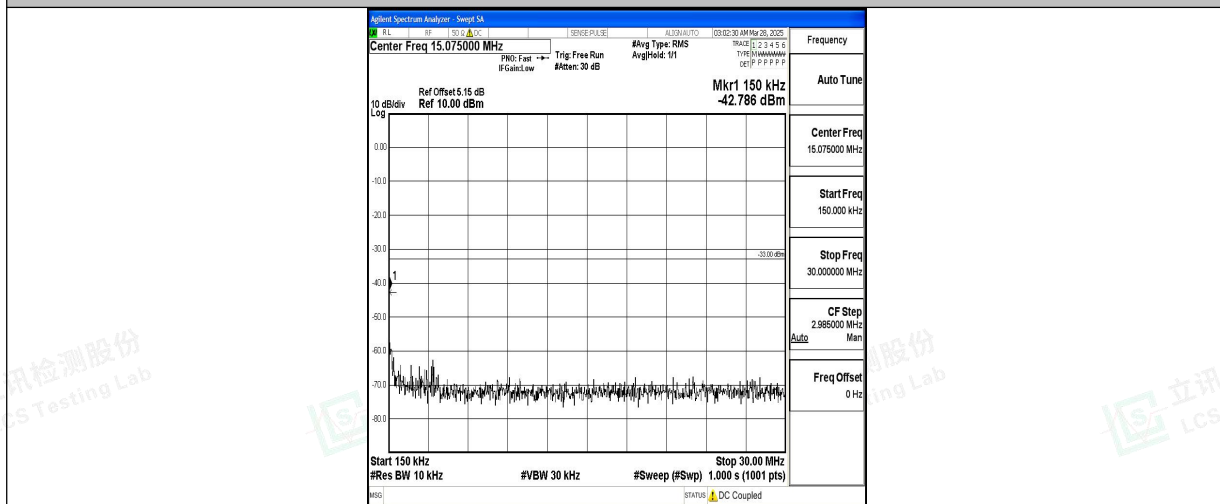
Band2_10MHz_QPSK_18900_1RB#0_0.15~30_0.15~30
