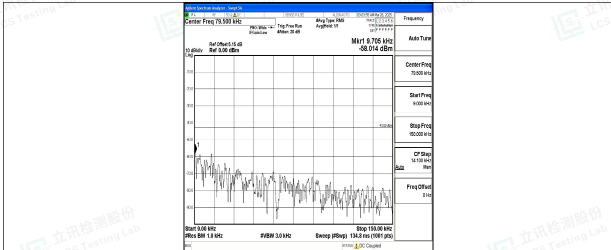
Band2_10MHz_16QAM_19150_1RB#0_0.009~0.15_0.009~0.15
