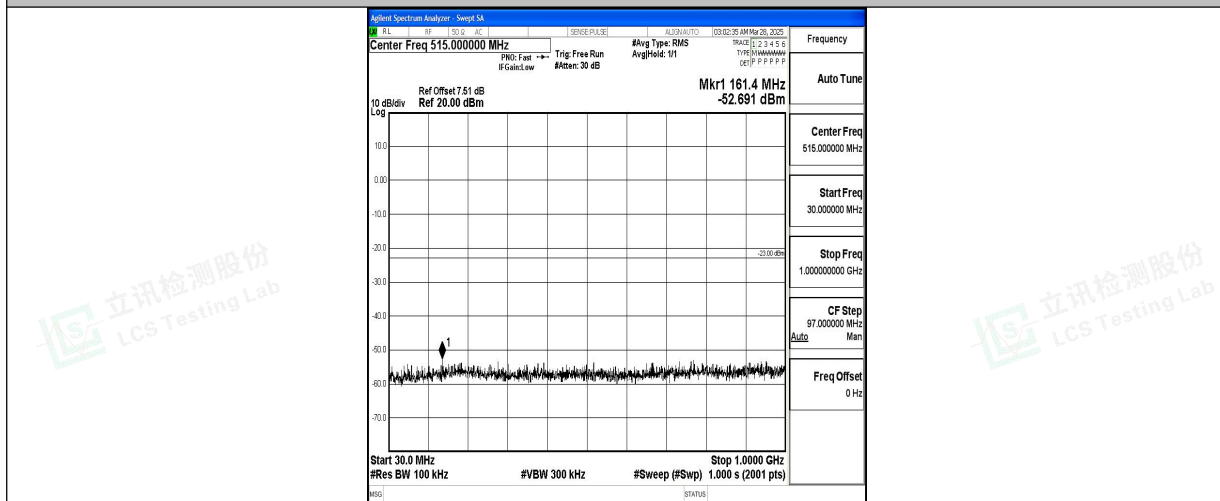
Band2_10MHz_QPSK_18900_1RB#0_30~1000_30~1000
