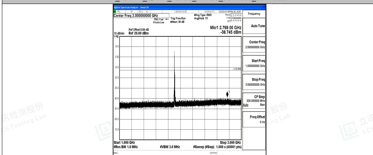
Band2_10MHz_QPSK_19150_1RB#0_1000~3000_1000~3000
