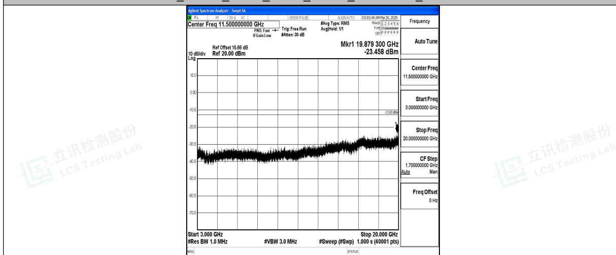
Band2_10MHz_QPSK_19150_1RB#0_3000~20000_3000~20000
