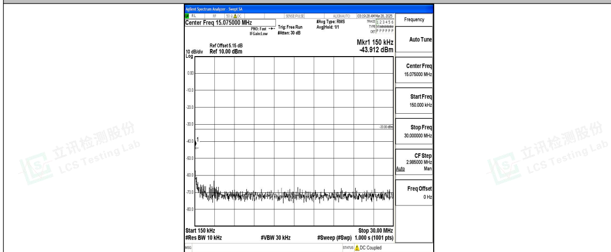
Band2_15MHz_16QAM_18675_1RB#0_0.15~30_0.15~30
