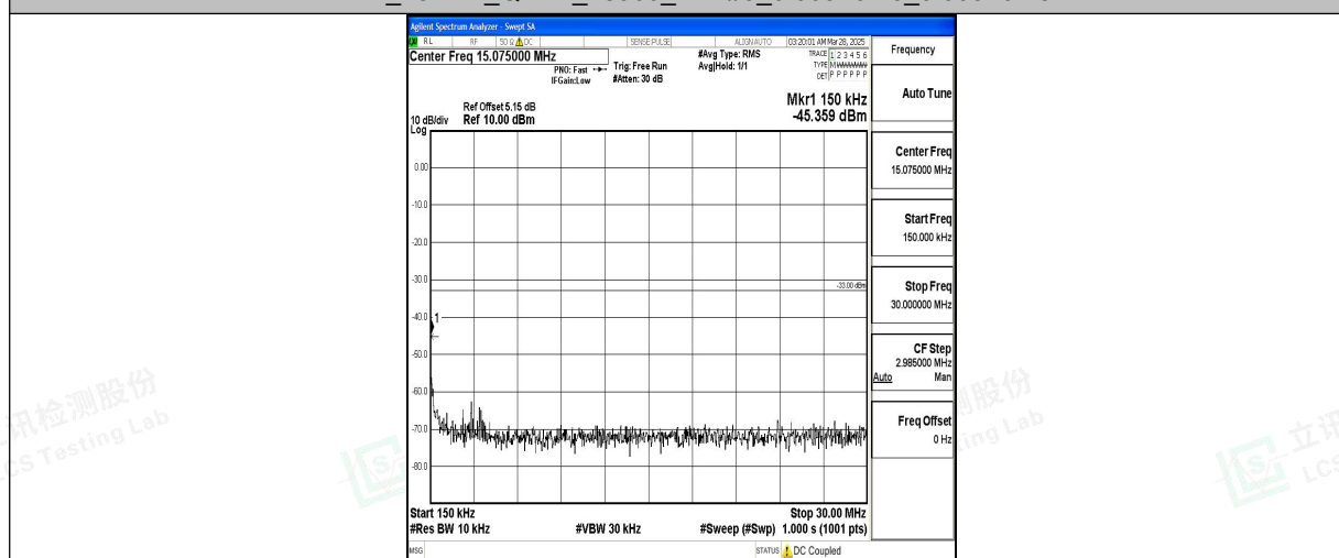
Band2_15MHz_QPSK_18900_1RB#0_0.15~30_0.15~30
