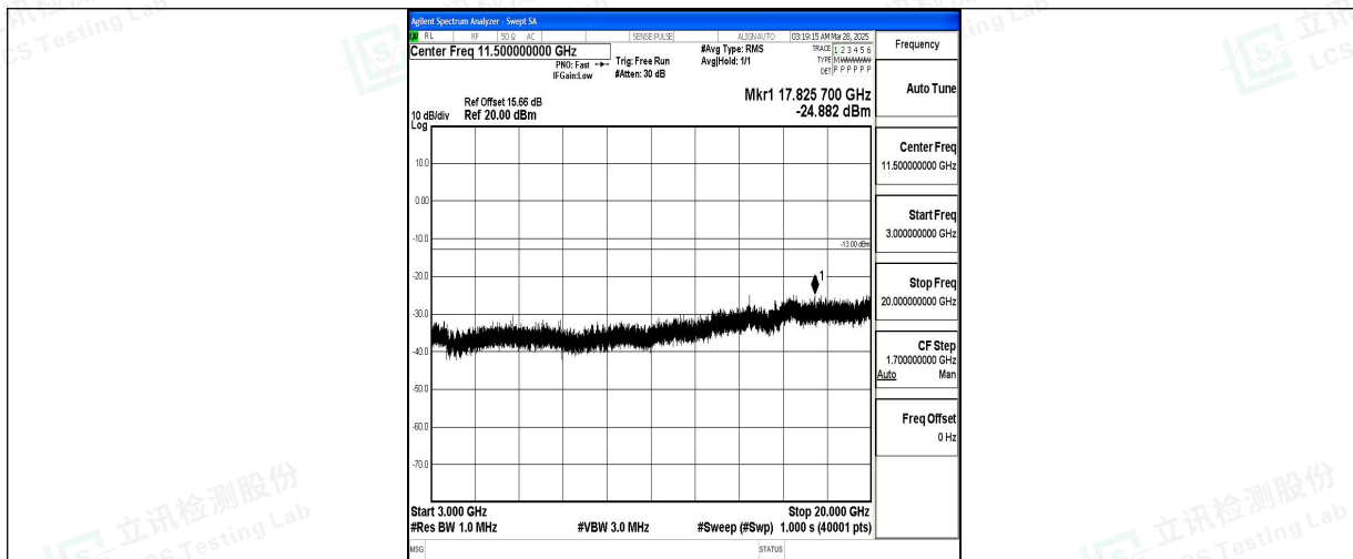
Band2_15MHz_QPSK_18675_1RB#0_3000~20000_3000~20000
