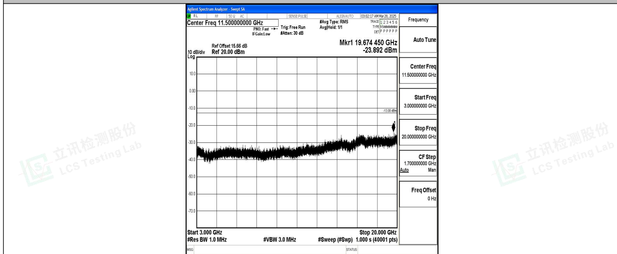
Band2_10MHz_16QAM_18650_1RB#0_3000~20000_3000~20000
