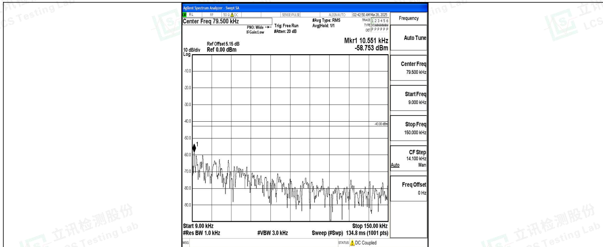
Band2_5MHz_QPSK_18900_1RB#0_0.009~0.15_0.009~0.15
