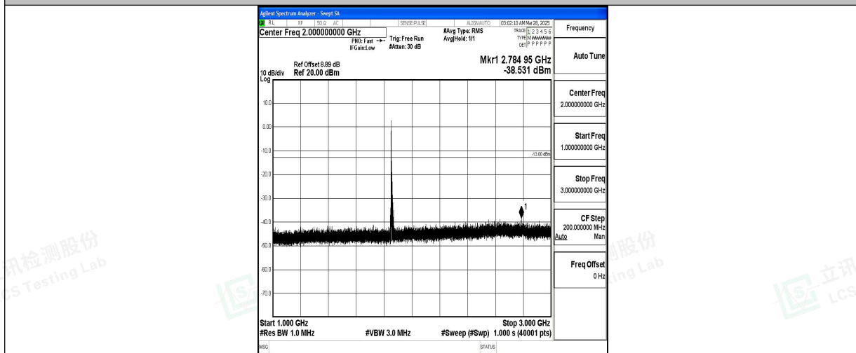
Band2_10MHz_16QAM_18650_1RB#0_1000~3000_1000~3000
