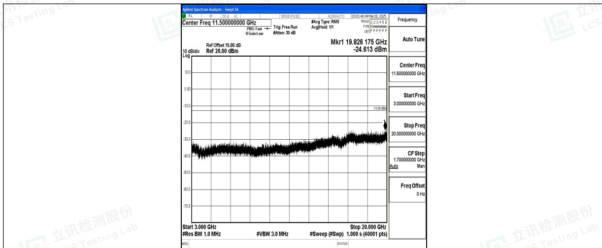
Band2_10MHz_QPSK_18650_1RB#0_3000~20000_3000~20000
