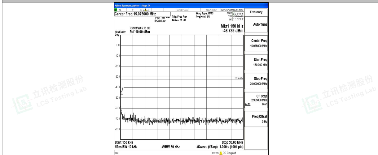
Band2_5MHz_QPSK_19175_1RB#0_0.15~30_0.15~30
