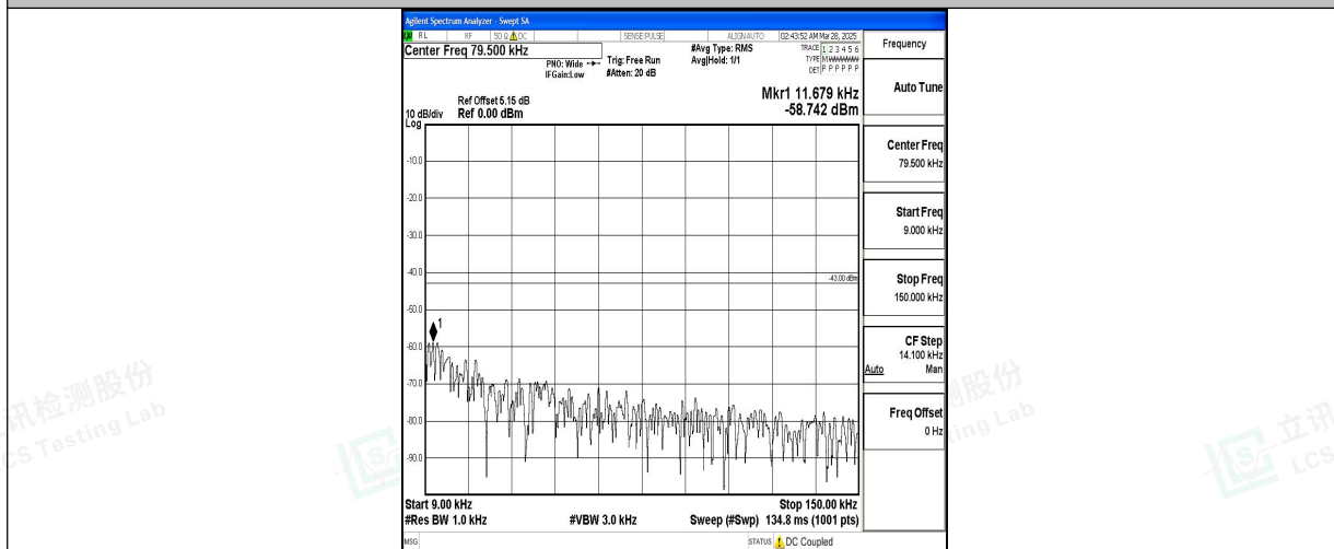
Band2_5MHz_QPSK_19175_1RB#0_0.009~0.15_0.009~0.15
