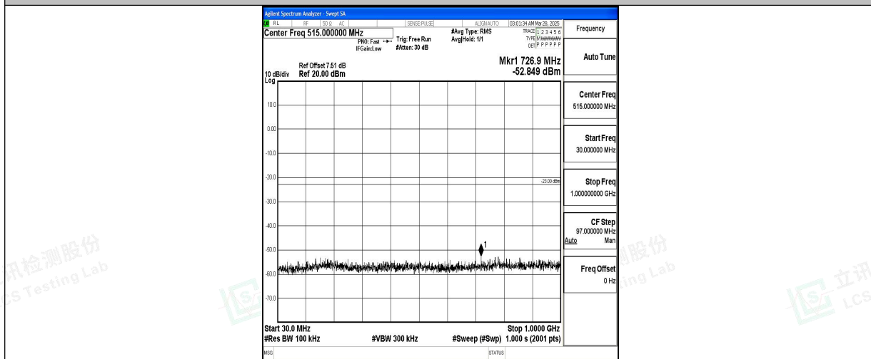
Band2_10MHz_QPSK_18650_1RB#0_30~1000_30~1000
