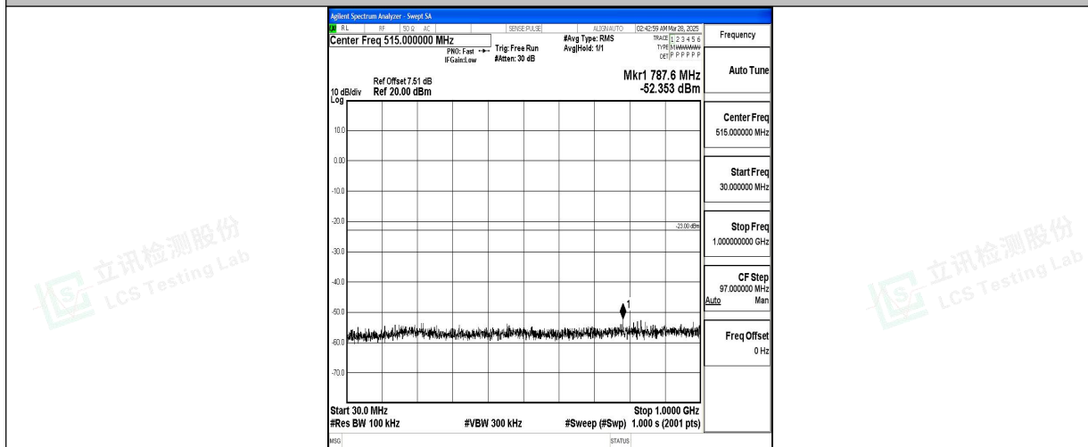
Band2_5MHz_QPSK_18900_1RB#0_30~1000_30~1000
