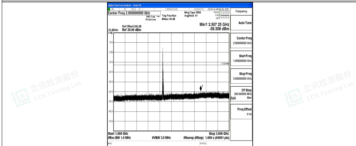
Band2_10MHz_QPSK_18650_1RB#0_1000~3000_1000~3000
