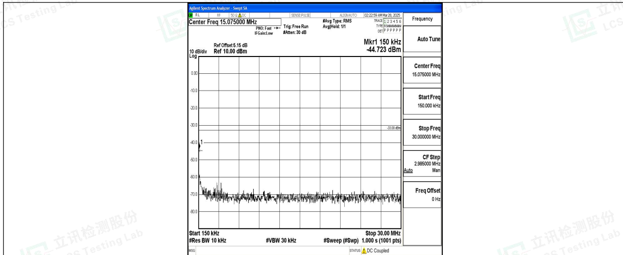
Band2_3MHz_16QAM_18900_1RB#0_0.15~30_0.15~30
