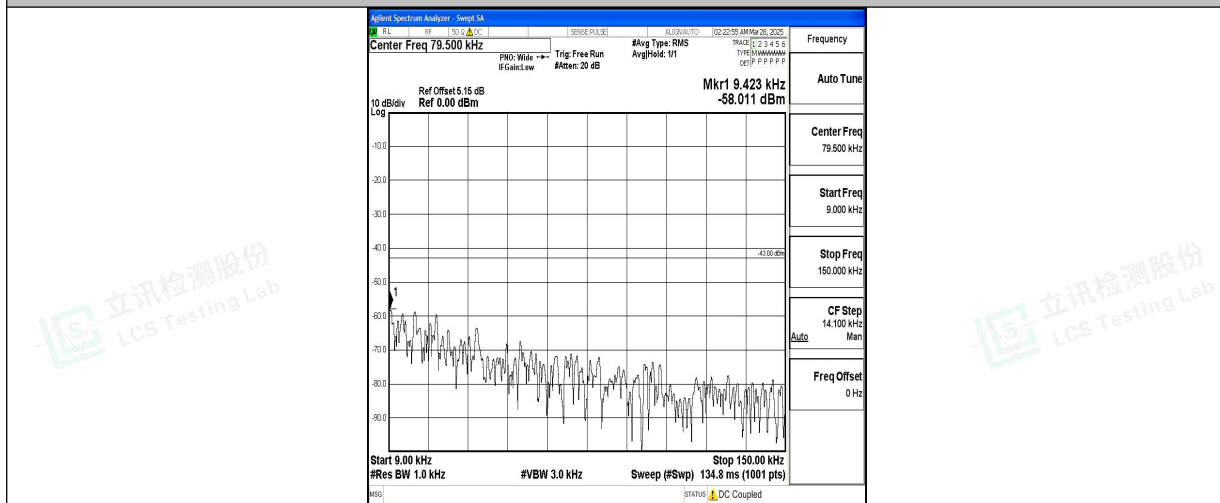
Band2_3MHz_16QAM_18900_1RB#0_0.009~0.15_0.009~0.15
