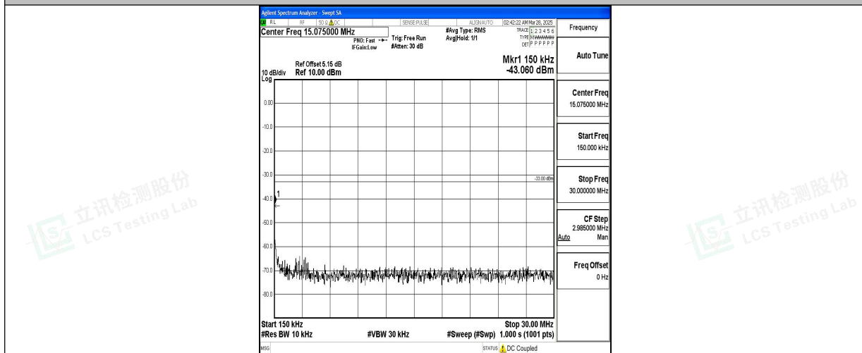
Band2_5MHz_16QAM_18625_1RB#0_0.15~30_0.15~30
