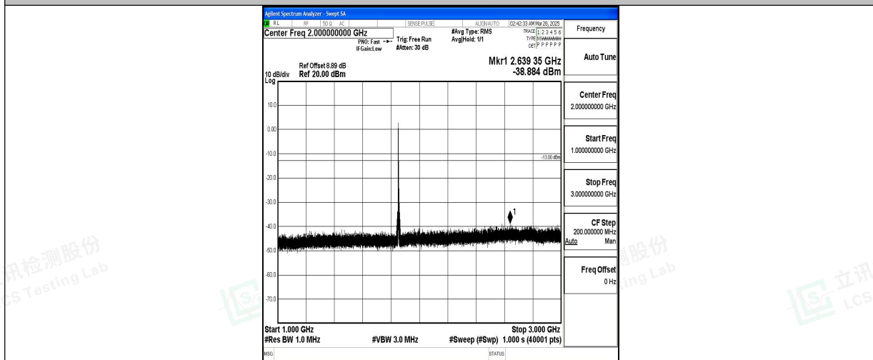
Band2_5MHz_16QAM_18625_1RB#0_1000~3000_1000~3000
