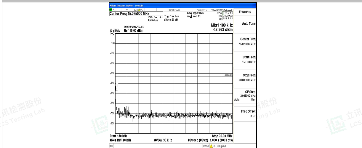
Band2_3MHz_QPSK_18900_1RB#0_0.15~30_0.15~30
