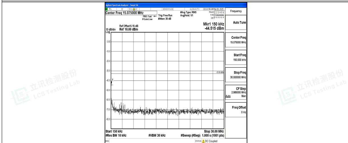
Band2_3MHz_16QAM_18615_1RB#0_0.15~30_0.15~30
