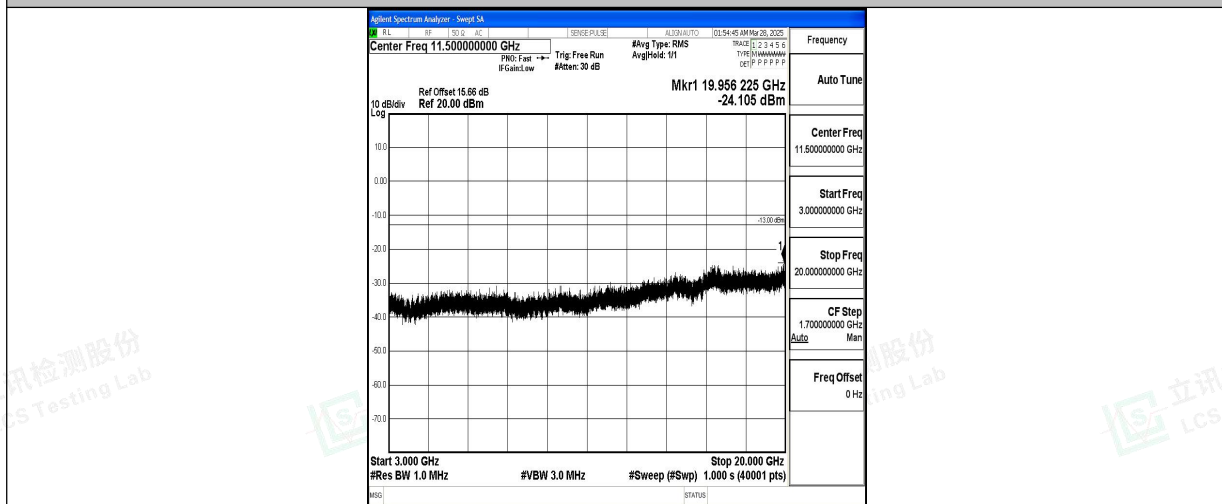
Band2_1.4MHz_QPSK_18900_1RB#0_3000~20000_3000~20000
