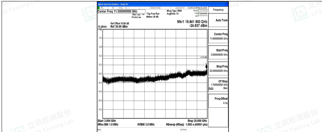
Band2_1.4MHz_16QAM_18900_1RB#0_3000~20000_3000~20000
