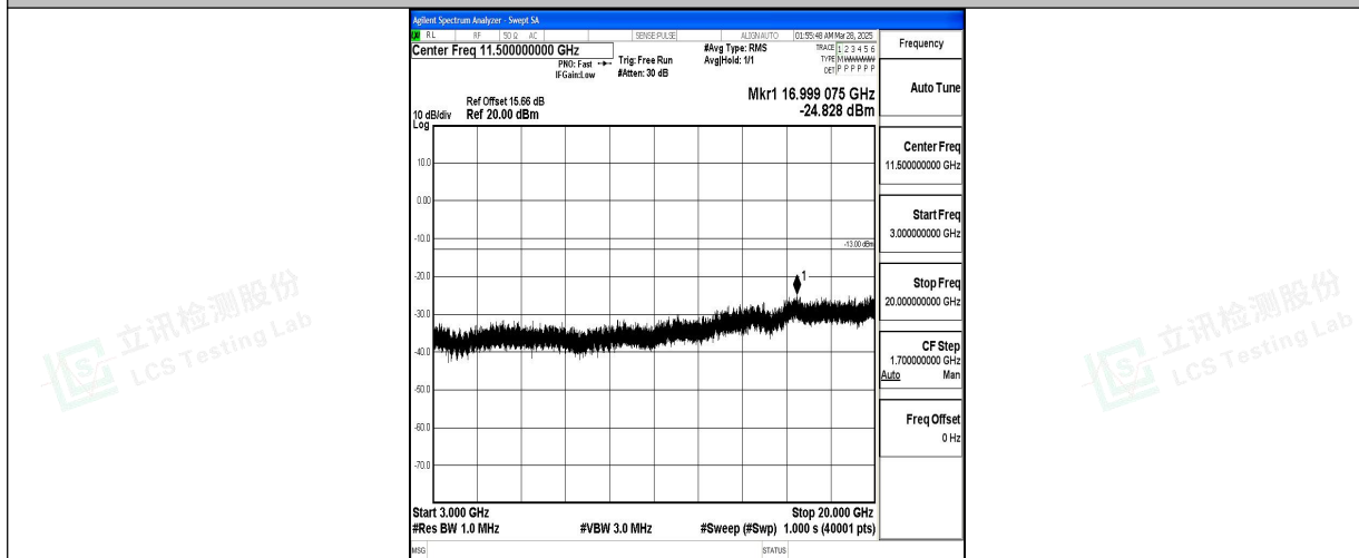
Band2_1.4MHz_QPSK_19193_1RB#0_3000~20000_3000~20000
