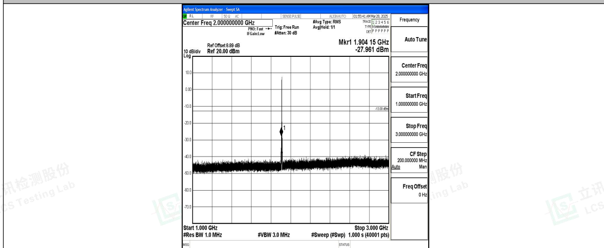
Band2_1.4MHz_QPSK_19193_1RB#0_1000~3000_1000~3000
