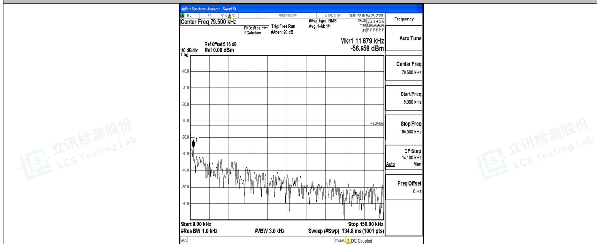
Band2_1.4MHz_16QAM_18900_1RB#0_0.009~0.15_0.009~0.15
