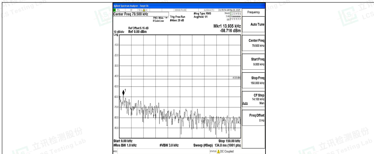
Band2_1.4MHz_16QAM_19193_1RB#0_0.009~0.15_0.009~0.15
