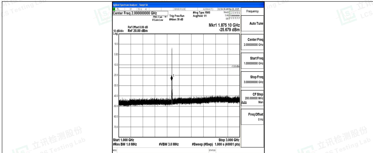
Band2_1.4MHz_QPSK_18900_1RB#0_1000~3000_1000~3000
