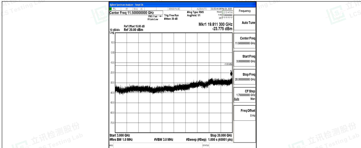
Band2_1.4MHz_QPSK_18607_1RB#0_3000~20000_3000~20000
