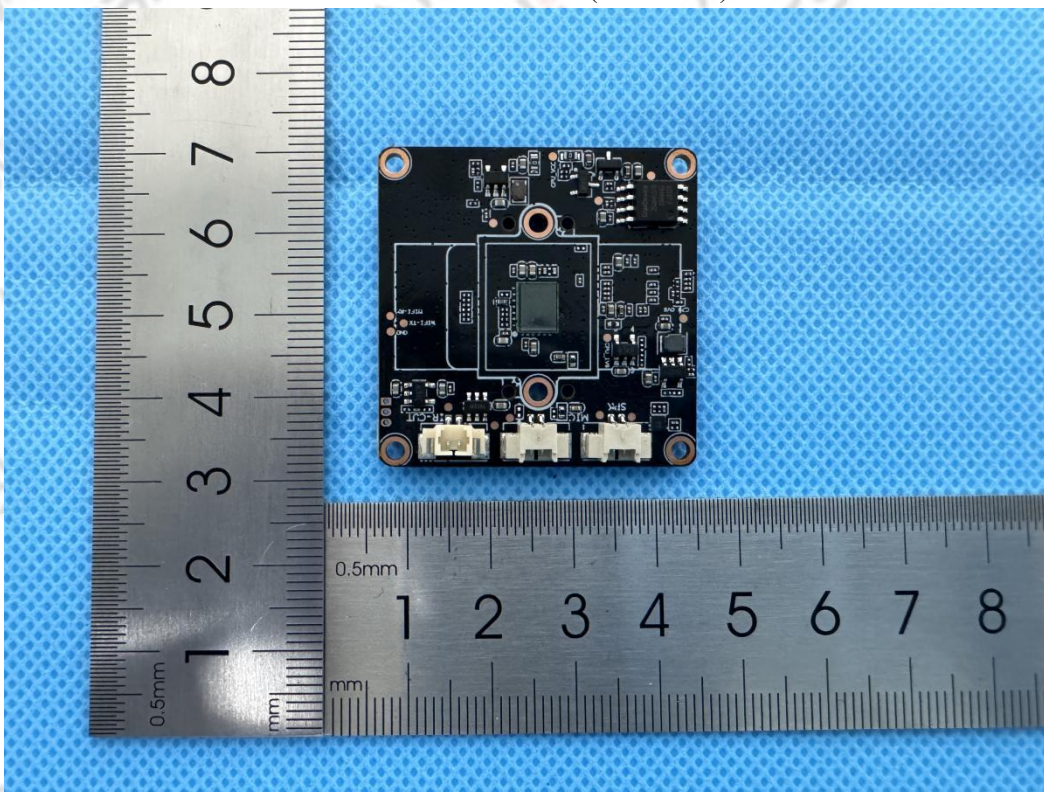
OPEN VIEW OF EUT(FIGURE 4)
