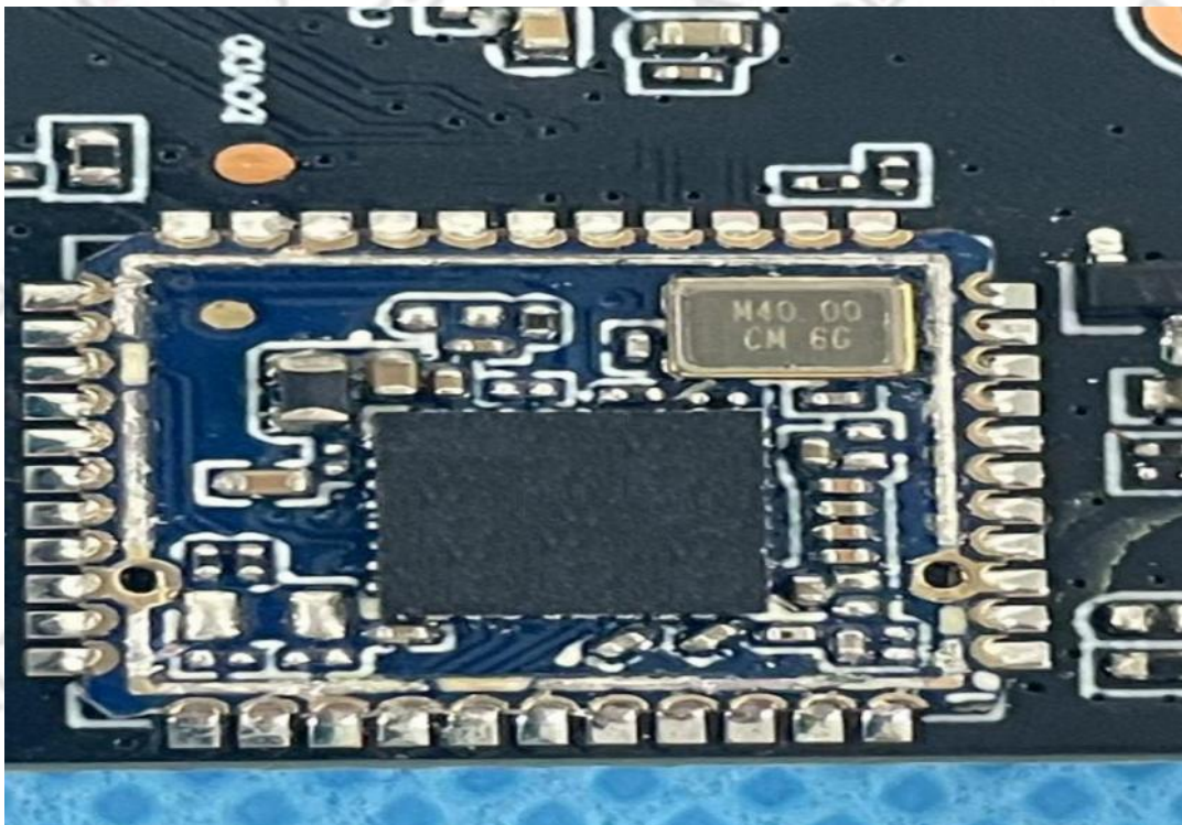
INTERNAL VIEW OF EUT(FIGURE 2)
