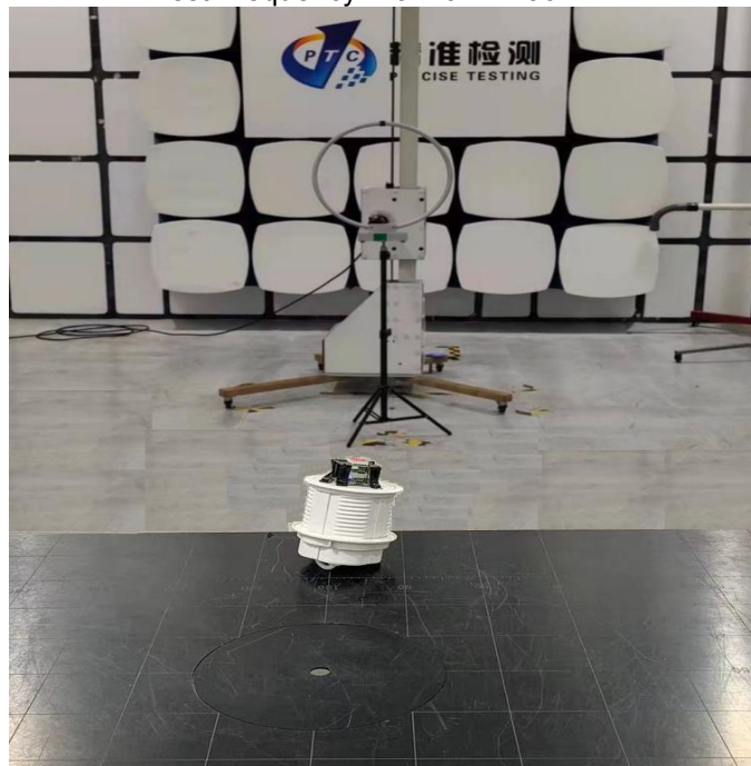
Radiated Spurious Emissions Test Frequency From 9KHz-30MHz
