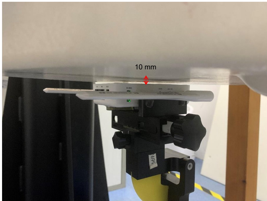
Back Side (10mm) of WWAN Antenna
