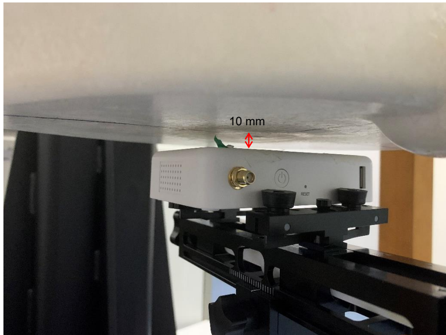
Front Side (10mm) of WLAN Antenna
