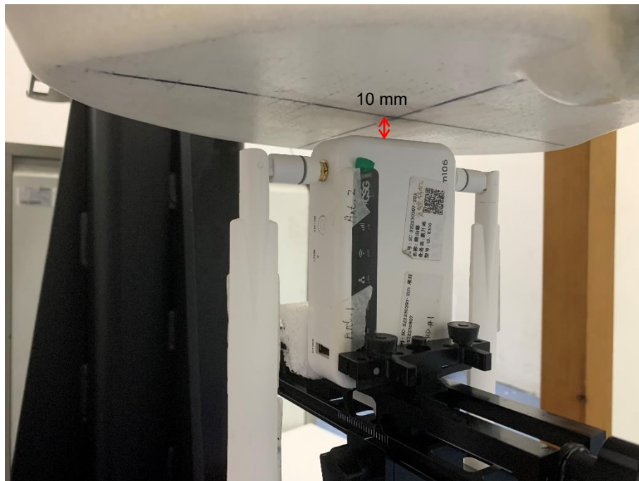
Left Side (10mm) of WWAN Antenna
