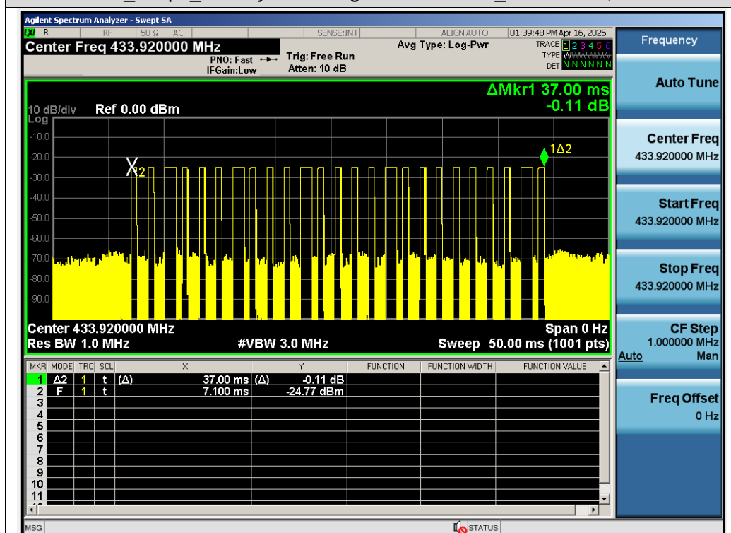
Test_Graph_Pulse Cycle Number Display
