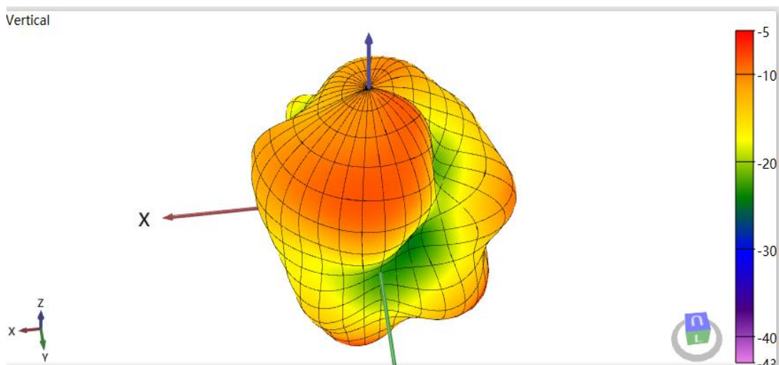
Antenna 2440MHz 3D-Vertical Pattern
