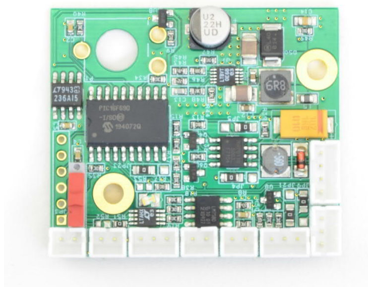
EUT_PCB brightness controller front side view (Photos provided by the applicant)
