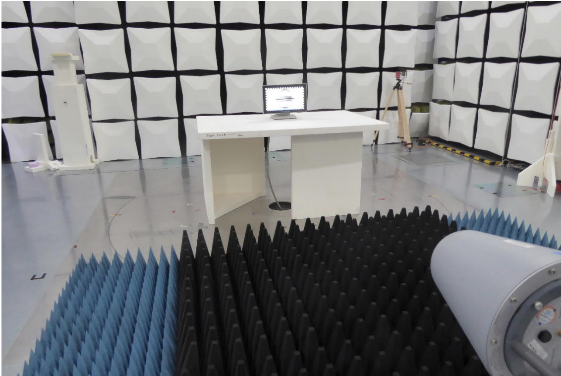
Test setup 3: Radiated Emission 1GHz to 12 GHz/Front side view
