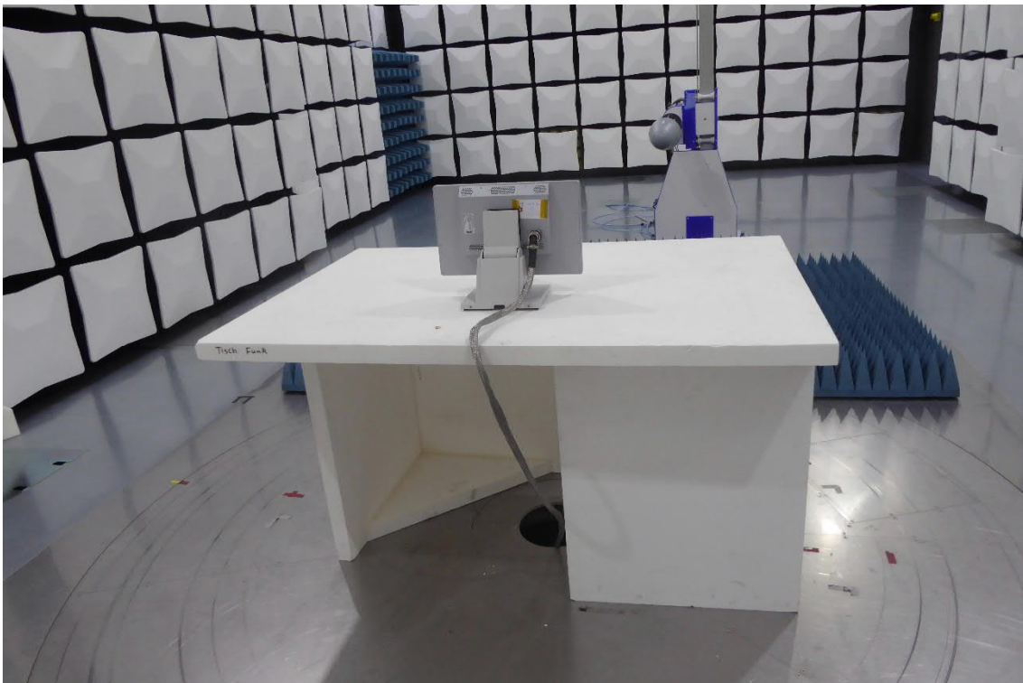
Test setup 4: Radiated Emission 1GHz to 12 GHz/Rear side view
