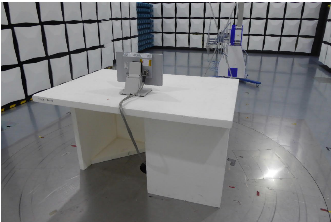
Test setup 2: Radiated Emission 30 MHz to 1 GHz/Rear side view
