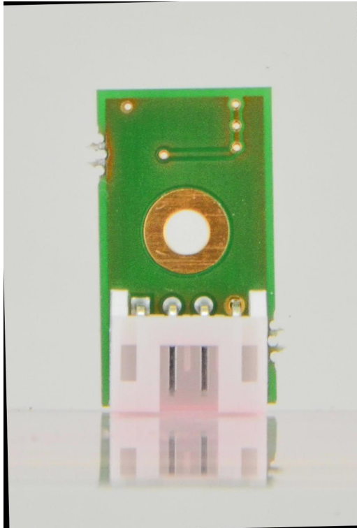
Photo 11: EUT/PCB light sensor card front side view
