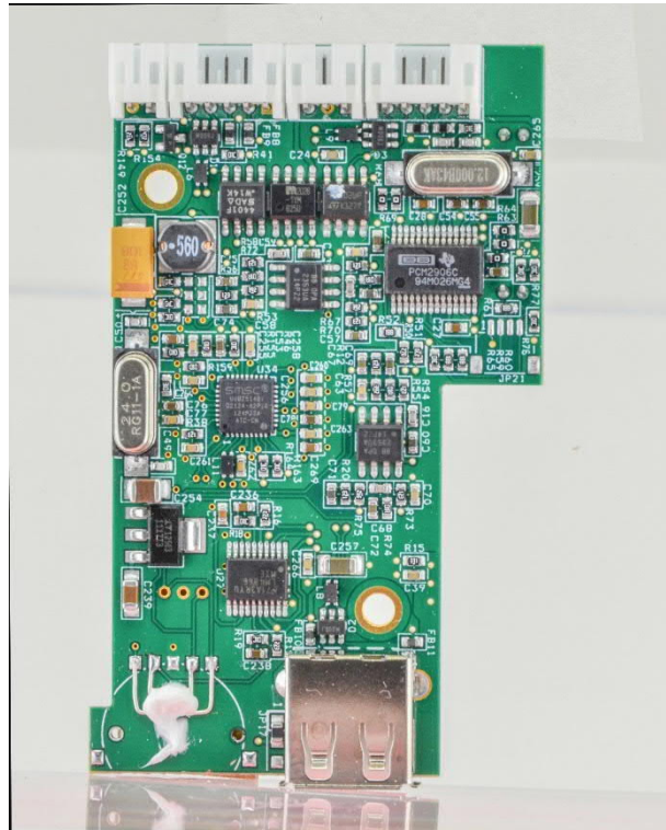
Photo 15: EUT/PCB USB-HUB&Sound front side view
