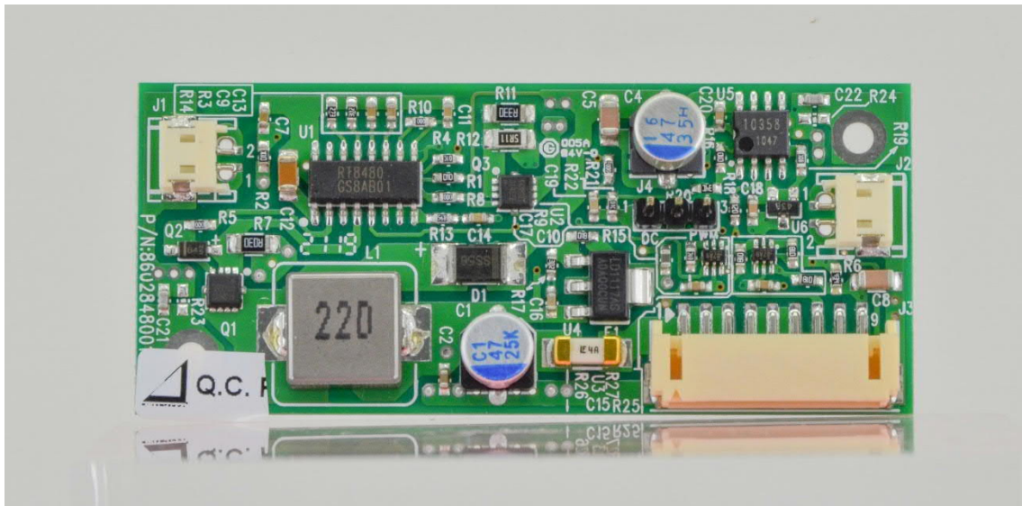
Photo 9: EUT/PCB LED-Drivingboard front side view
