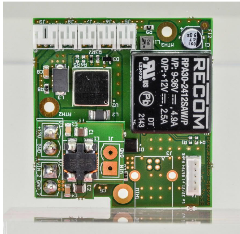
Photo 5: EUT/PCB DC-DC converter front side view
