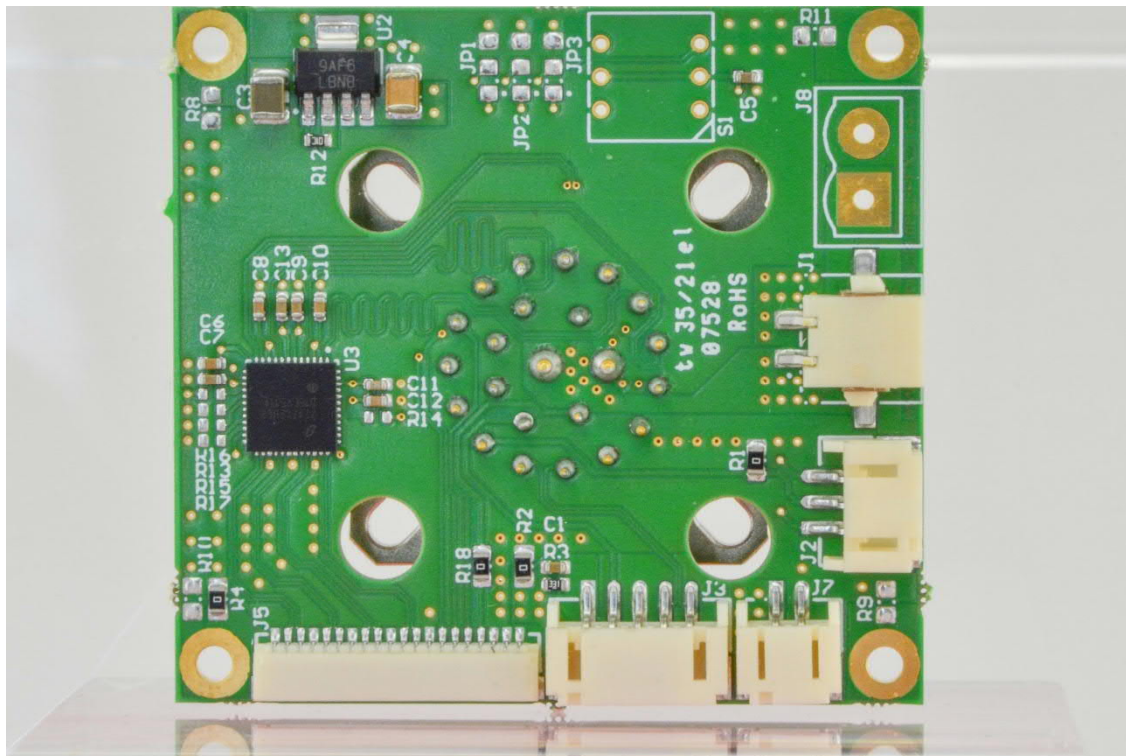
Photo 4: EUT/PCB connection board Mil rear side
