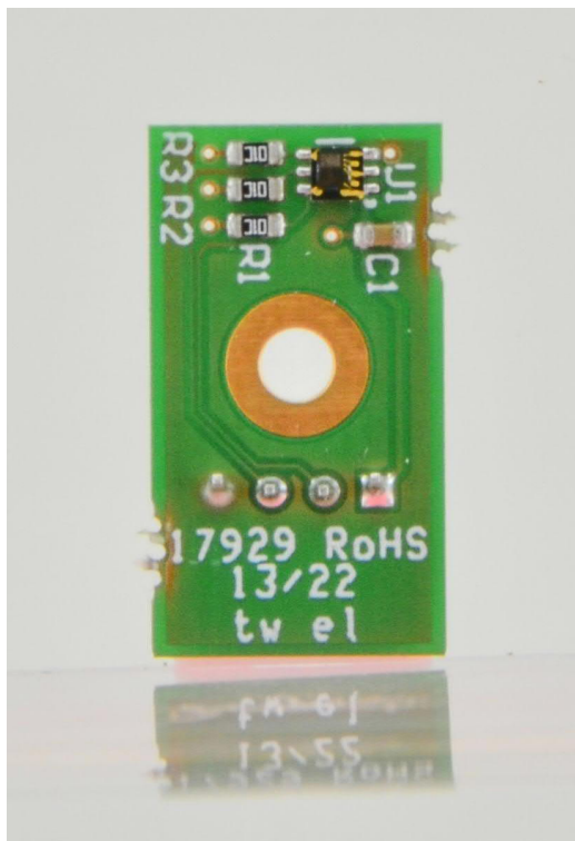
Photo 12: EUT/PCB light sensor card rear side view
