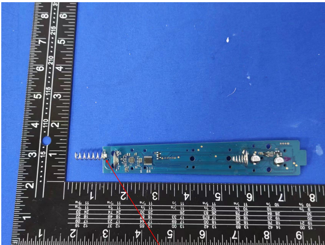
Spring antenna
