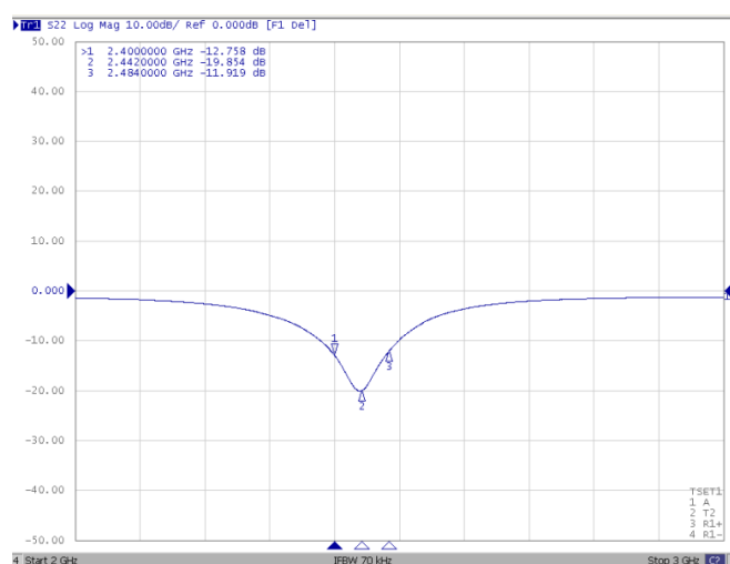
Return Loss & Radiation
