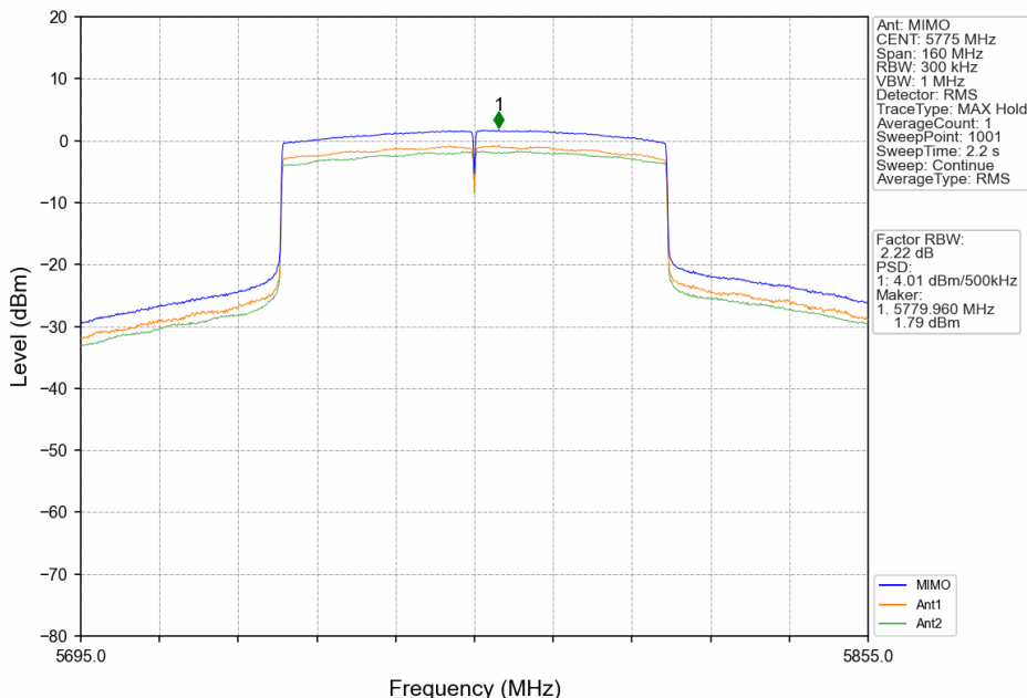
802.11ax(HEW80)_MCH_5775MHz_RU996_Left_MIMO_NTNV
