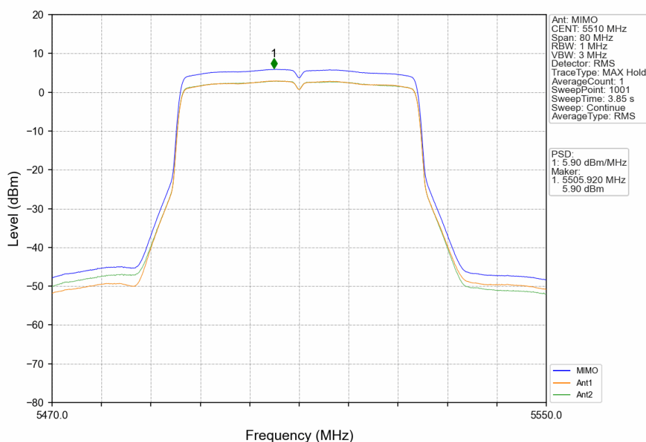
802.11ax(HEW40)_LCH_5510MHz_RU484_Left_MIMO_NTNV
