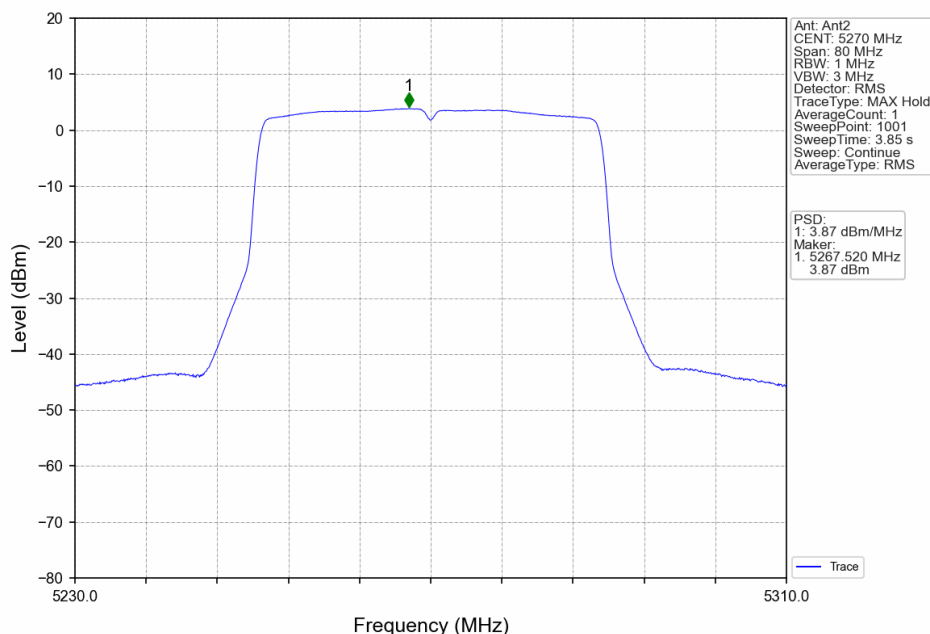
802.11ax(HEW40)_LCH_5270MHz_RU484_Left_MIMO_NTNV
