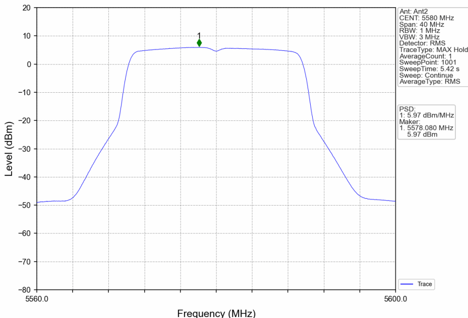
802.11ax(HEW20)_MCH_5580MHz_RU242_Left_MIMO_NTNV
