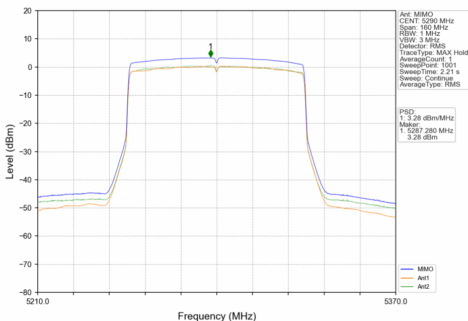
802.11ax(HEW80)_MCH_5290MHz_RU996_Left_MIMO_NTNV
