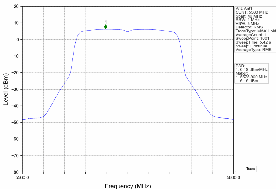
802.11ax(HEW20)_MCH_5580MHz_RU242_Left_Ant1_NTNV
