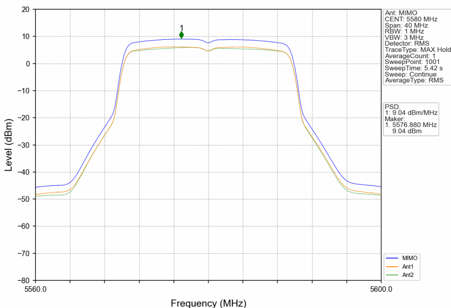
802.11ax(HEW20)_MCH_5580MHz_RU242_Left_MIMO_NTNV
