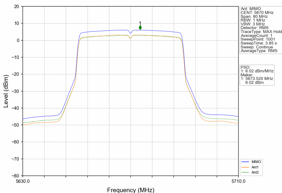
802.11ax(HEW40)_HCH_5670MHz_RU484_Left_MIMO_NTNV
