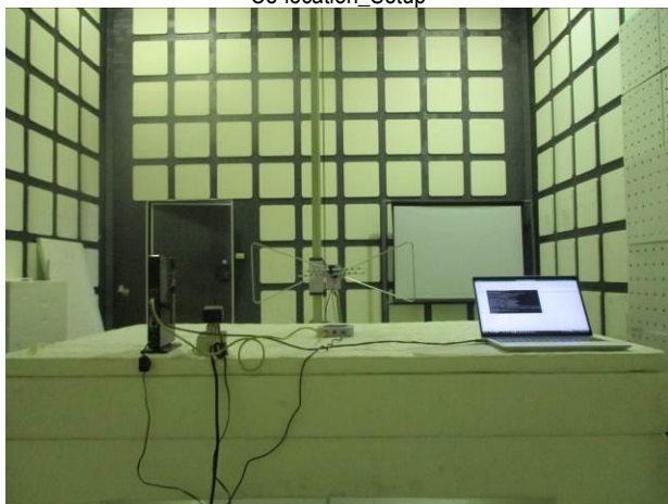
Co-location_Setup
