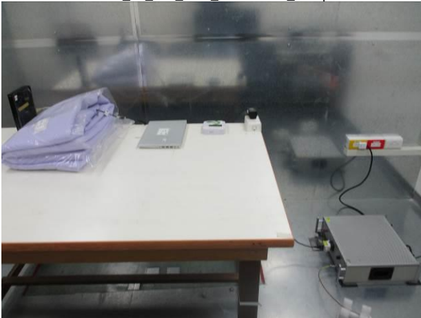
FCC_15_225_NFC_Conduction_Setup
