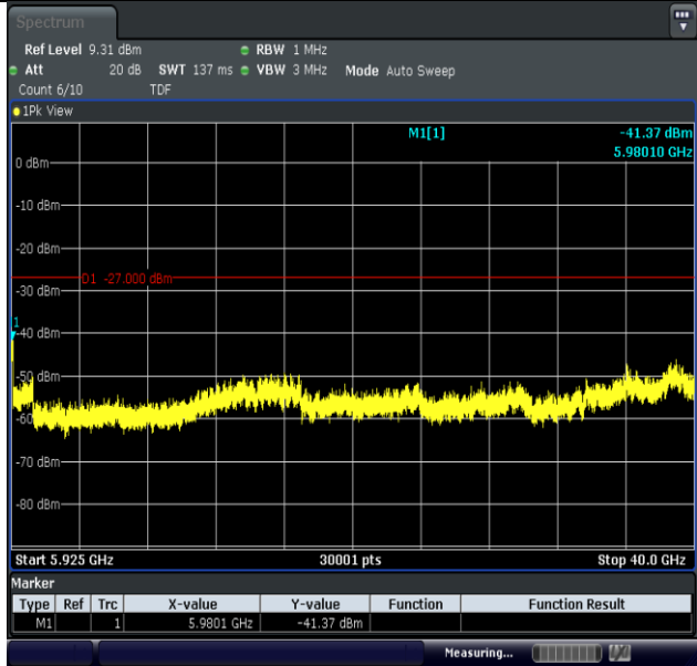
11A-Ant2-5785-5925~40000-PASS
