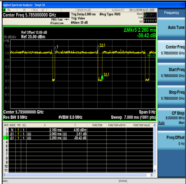
NTNV-11A-Ant2-5785
