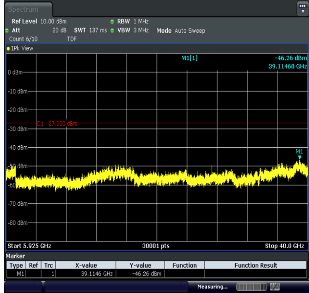
11A-Ant1-5825-5925~40000-PASS
