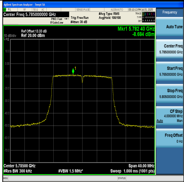
11A-Ant1-5785-PASS
