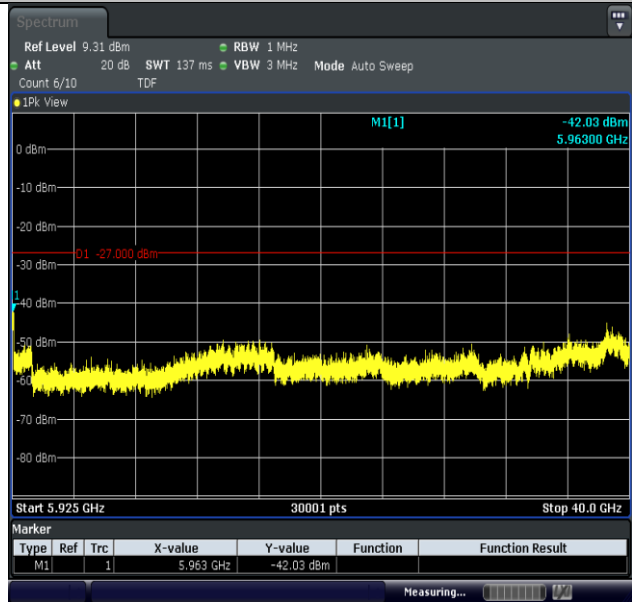
11A-Ant1-5745-5925~40000-PASS
