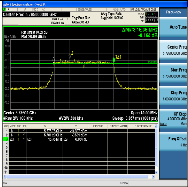
11A-Ant2-5785-PASS
