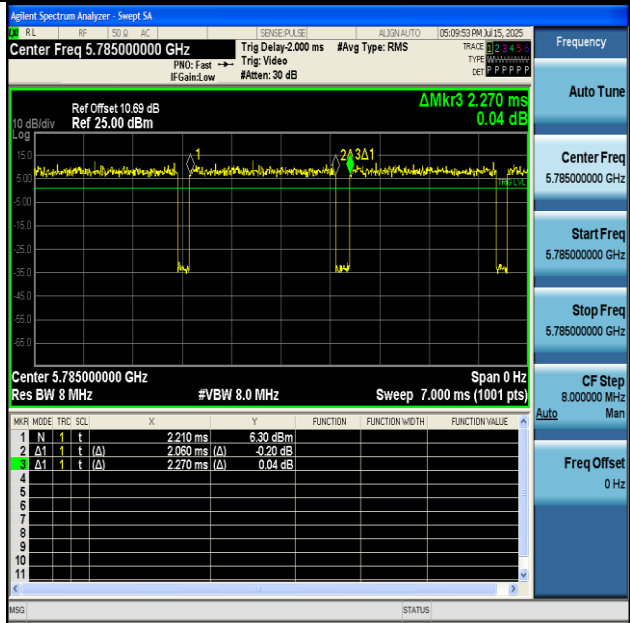
NTNV-11A-Ant1-5785
