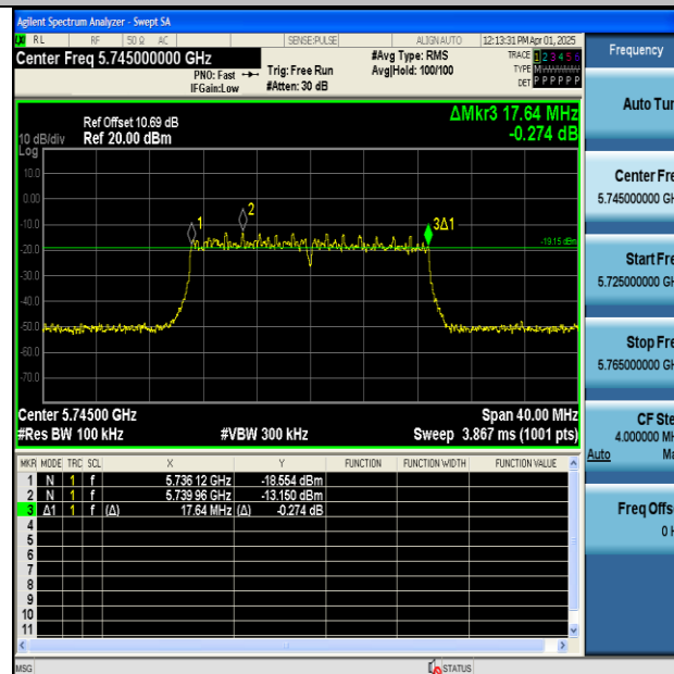
11AC20MIMO-Ant1-5745-PASS
