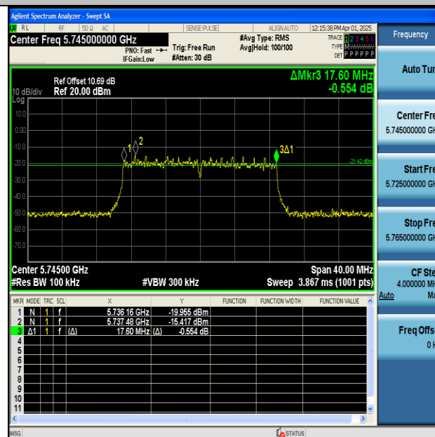
11AC20MIMO-Ant2-5745-PASS
