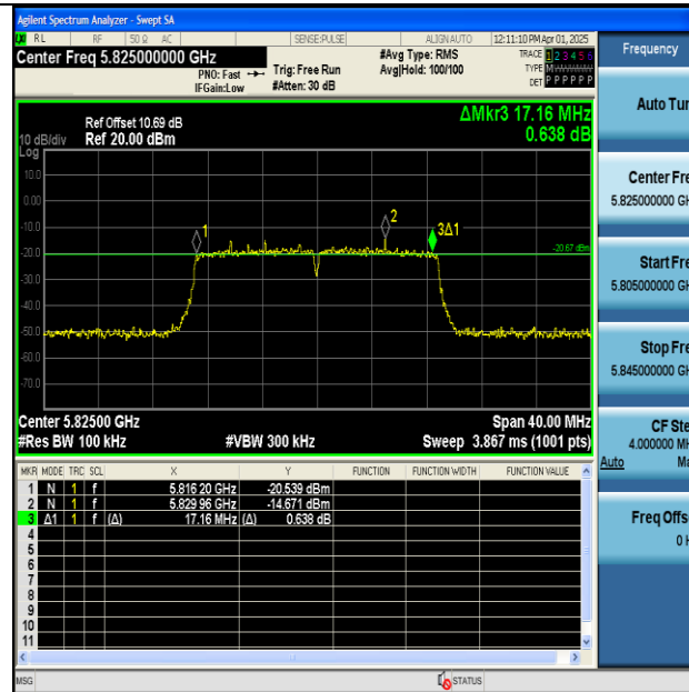
11N20MIMO-Ant2-5825-PASS
