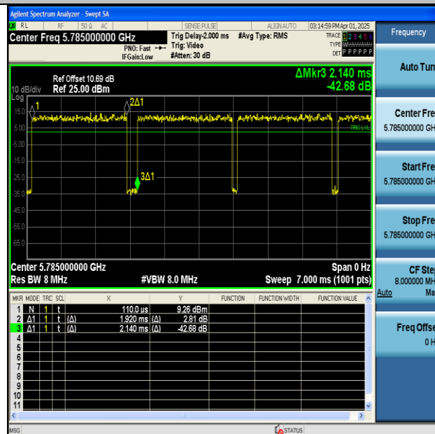
NTNV-11N20MIMO-Ant2-5785
