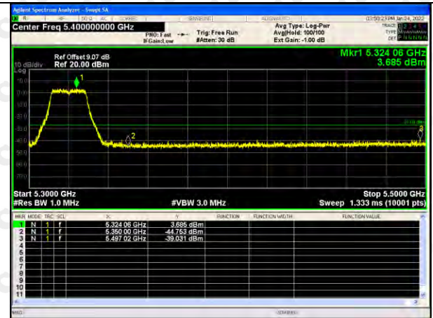
802.11n(HT40)-5310
