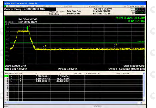
802.11n(HT40)-5310
