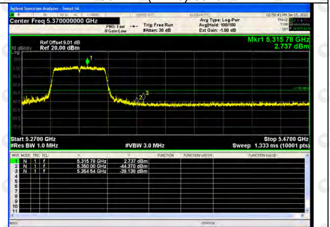
802.11n(HT40)-5310
