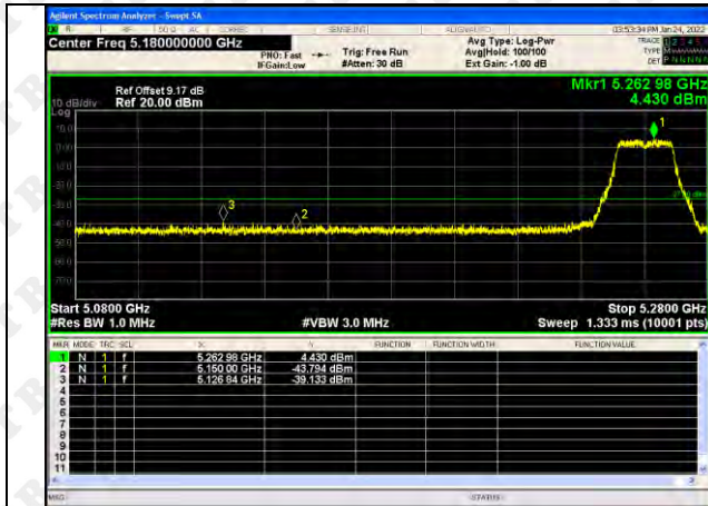
802.11n(HT40)-5270
