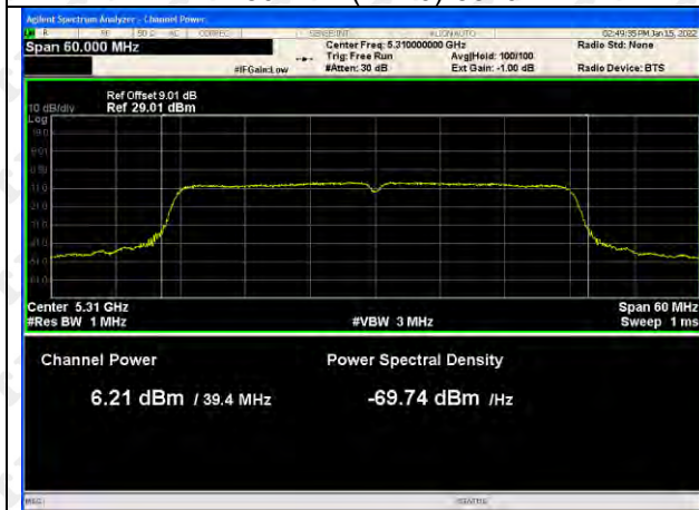
802.11n(HT40)-5310
