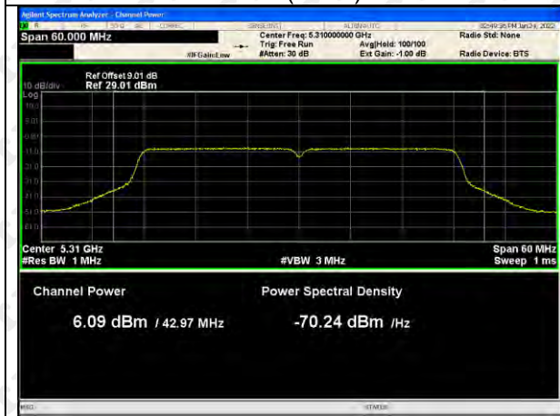
802.11n(HT40)-5310
