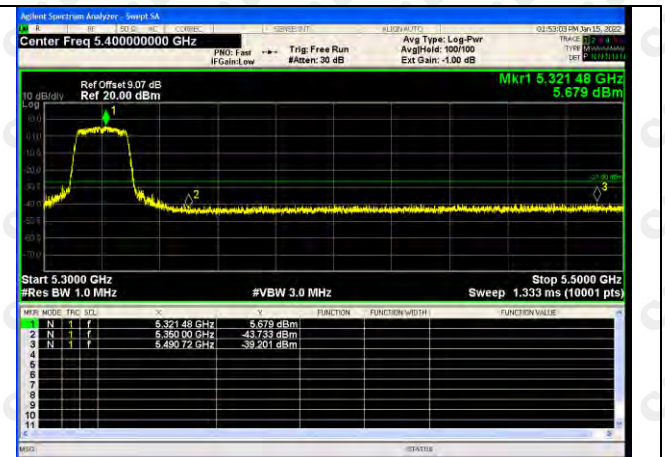
802.11n(HT40)-5310
