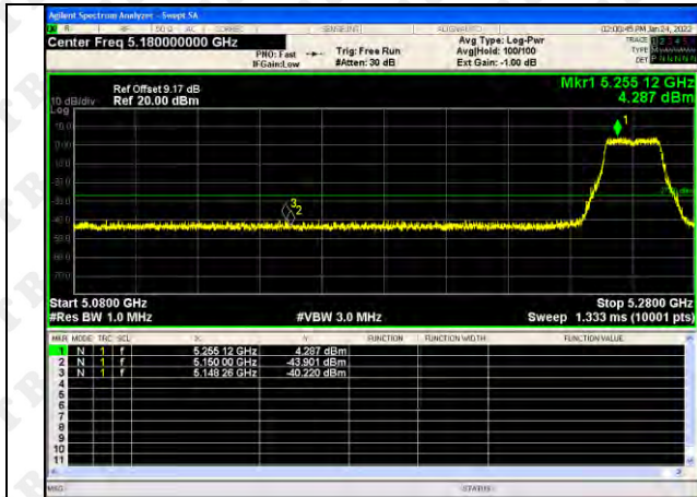
802.11n(HT40)-5270
