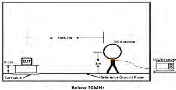
Figure 1. Below 30MHz
