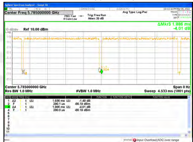
Band 4-802.11ac20
