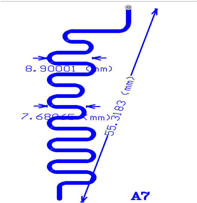
AntennaPhoto&Length(mm)
