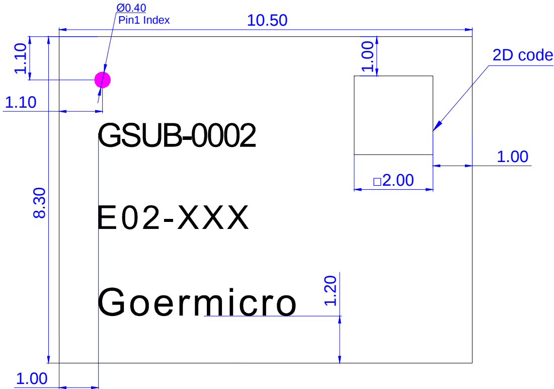
Top View (Chip Side View)
