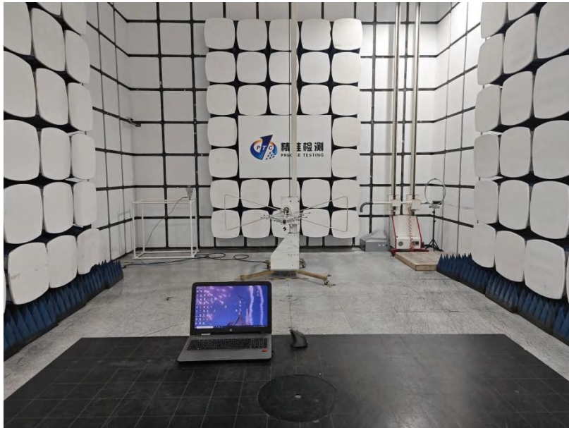
RADIATED EMISSION TEST(Below 1G)
