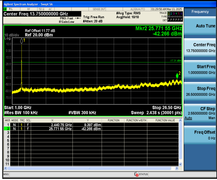
11G-Ant2-2462-0~Reference-PASS
