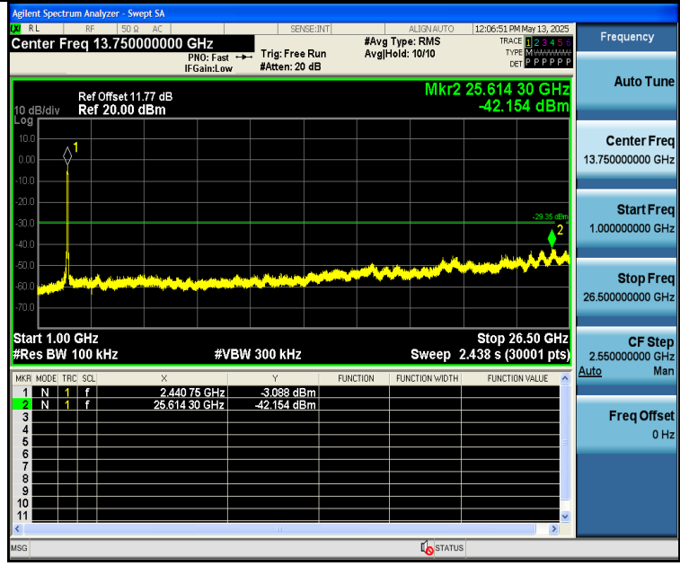
11N40SISO-Ant2-2452-0~Reference-PASS
