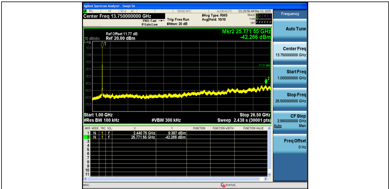
11G-Ant1-2462-0~Reference-PASS
