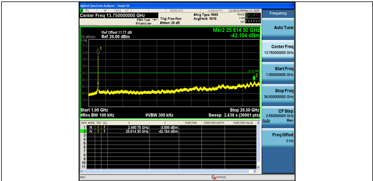
11N40SISO-Ant1-2452-0~Reference-PASS
