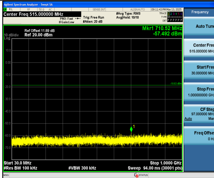
BLE_2M-Ant2-2440-0~Reference-PASS
