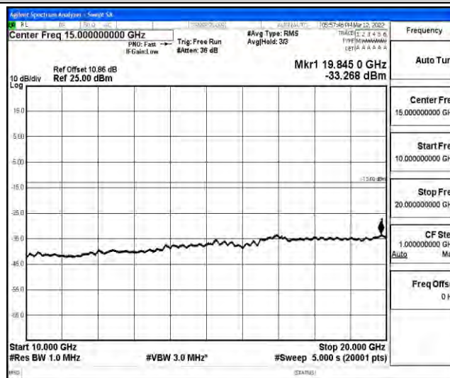
Band66-10MHz-QPSK-132622-1RB#0-Range5:10000~20000MHz
