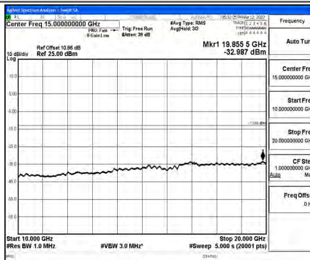
Band66-5MHz-QPSK-132647-1RB#0-Range5:10000~20000MHz
