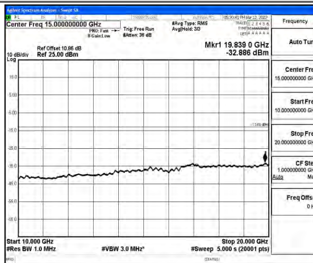
Band66-5MHz-16QAM-132322-1RB#0-Range5:10000~20000MHz
