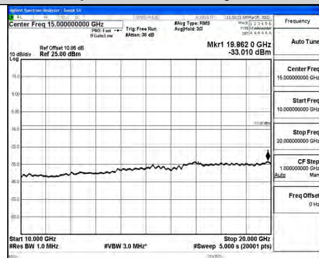
Band2-20MHz-16QAM-19100-1RB#0-Range5:10000~20000MHz
