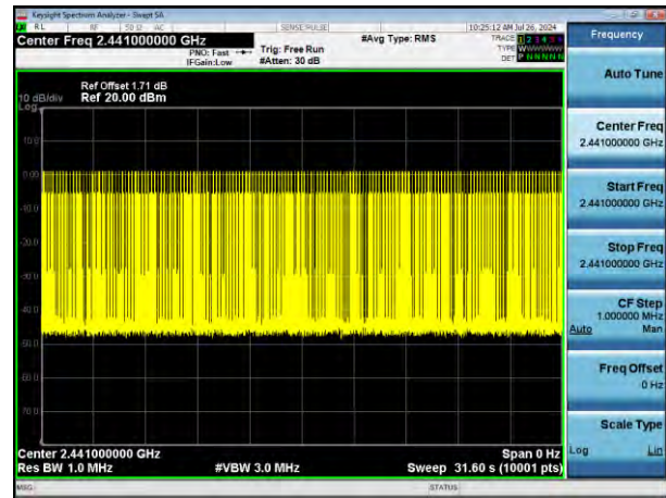
Accumulate(3DH1)
