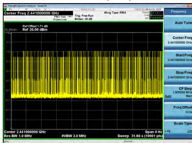
Accumulate(3DH5)
