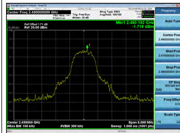
Reference Power
