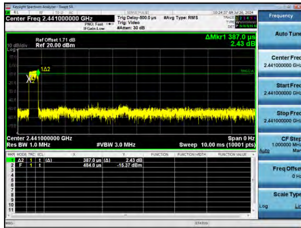
Burst(3DH1)
