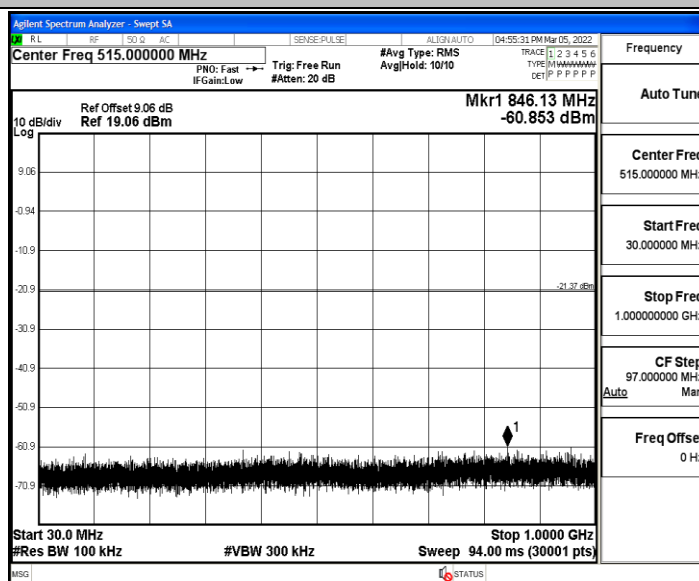
SRD_Ant1_2441.85_1000~26500
