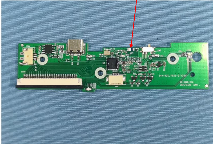
Ceramic Antenna
